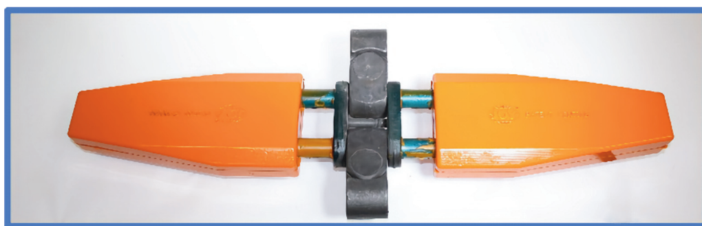
Figure 14 Urethane-coated dual sprocket flight bar.
