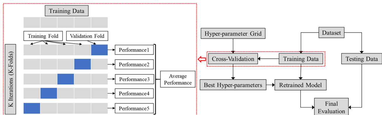
Fig. 4 Grid search with cross-validation to tune hyper-parameters
