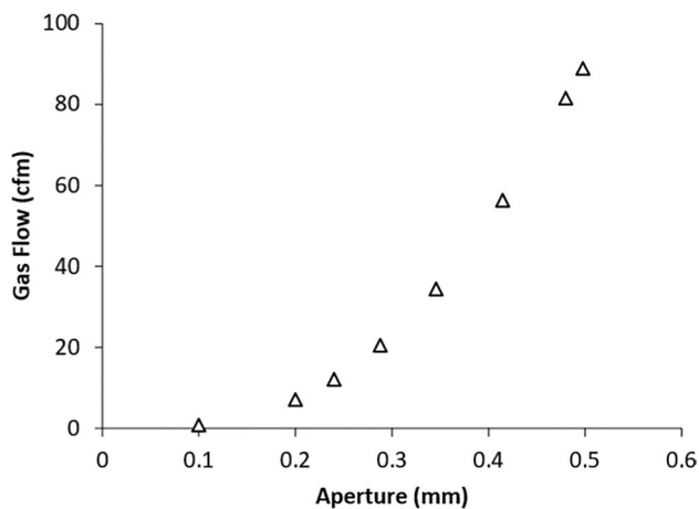
Fig. 5 Plot of variation in gas flow to the mine with changes in aperture of fracture connected to the casing breach (node 2 in Fig. 2)
