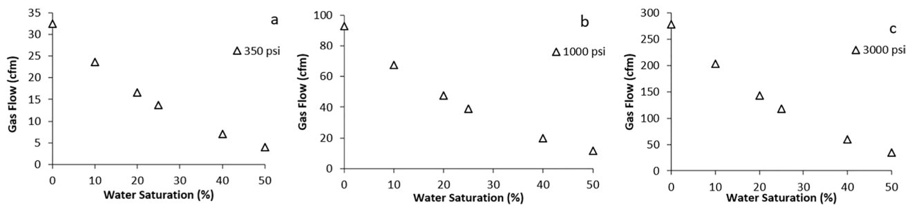
Fig. 4 Variation in gas flow with water saturation level
