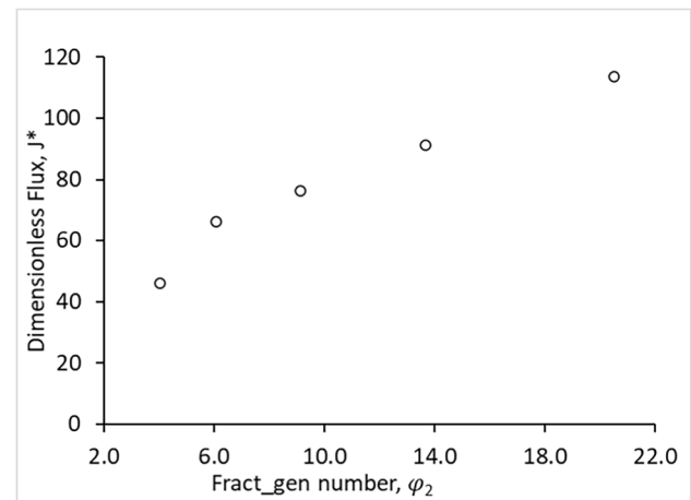
Fig. 3 Plot of dimensionless flux with Fract_gen number
