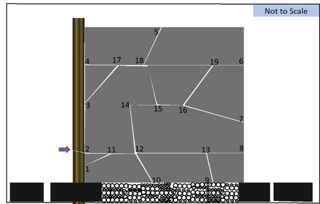
Fig. 2 A representation of the conceptual/deterministic discrete fracture network (DFN) used for this study. The arrow indicates the breach location. Nodes 1–10 are external nodes of the fracture network and nodes 11–19 are internal nodes of the fracture network
