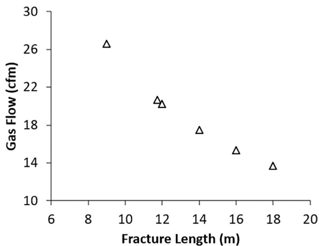
Fig. 6 Plot of gas flow to the mine with variation in fracture length from breach sources (nodes 2–11 in Fig. 2 and Table 1)
