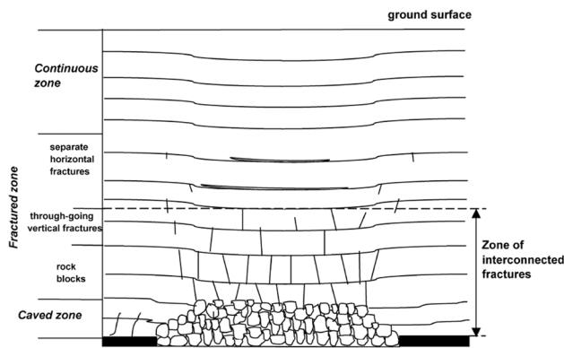
Fig. 12 Overburden zone movement due to longwall mining [12]
