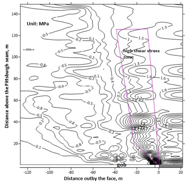
Fig. 13 Shear stress ( S_{xz} ) distribution in the overburden over the longwall face
