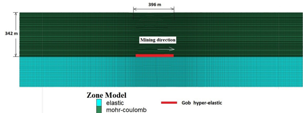
Fig. 8 Cross-sectional view of the FLAC3D model
