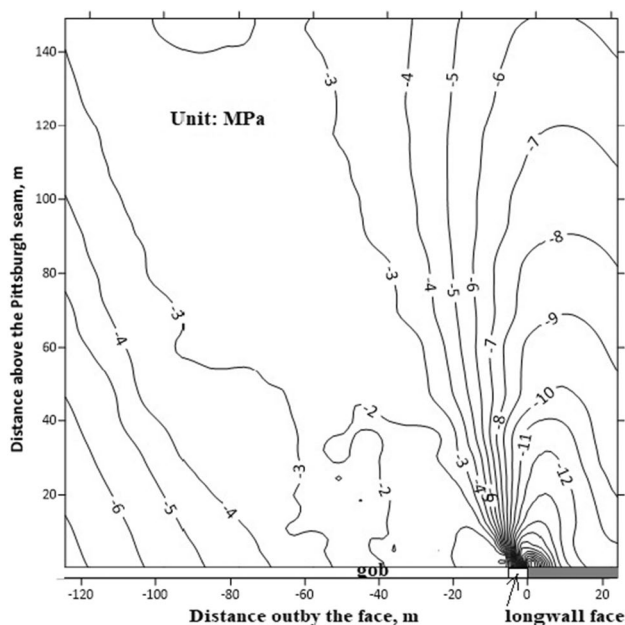
Fig. 10 Vertical stress distribution in the overburden over the longwall face
