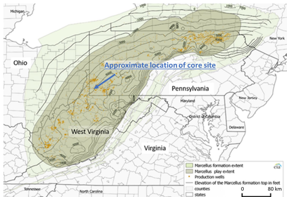
Fig. 2 Extent of the Marcellus Shale Formation [2]
