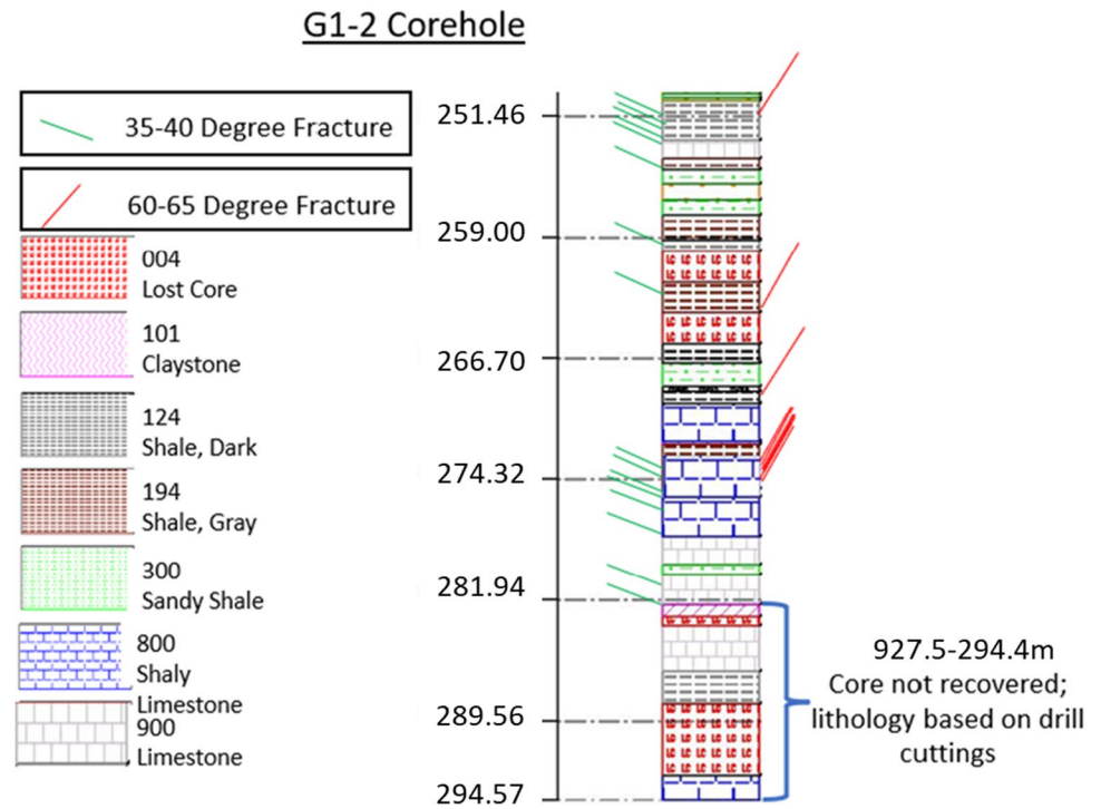
Fig. 7 Log of the corehole from 251.4 to 294.57 m
