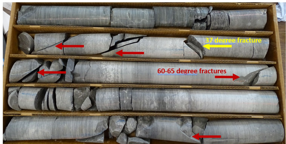
Fig. 6 High-angle fractures (in red) and low-angle fractures (in yellow) at a depth of 270.3 to 273.4 m
