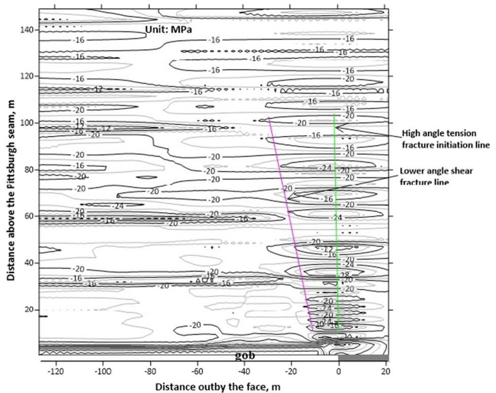
Fig. 14 Horizontal stress distribution in the overburden over the longwall face
