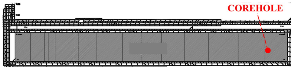
Fig. 1 Location of the corehole drilled into a mined-out longwall panel
