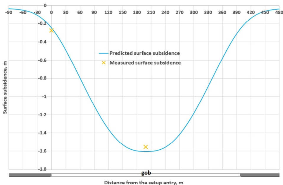
Fig. 9 Predicted surface subsidence along the longwall panel
