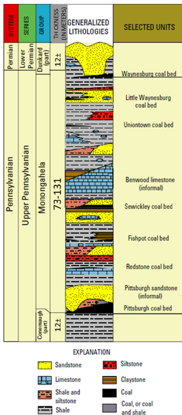
Fig. 4 General stratigraphic column of the Monongahela group including the Pittsburgh seam [4]
