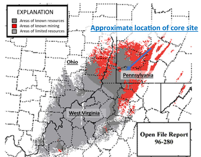
Fig. 3 Extent of the Pittsburgh Coal [3]
