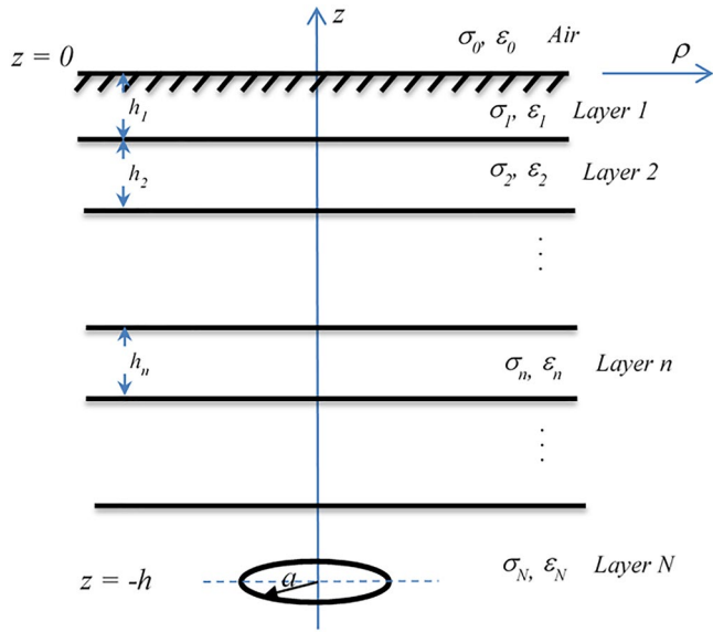
Figure 1. Magnetic dipole buried in a semi-infinite region which is comprised of N ( N > 3 ) layered Earth.
