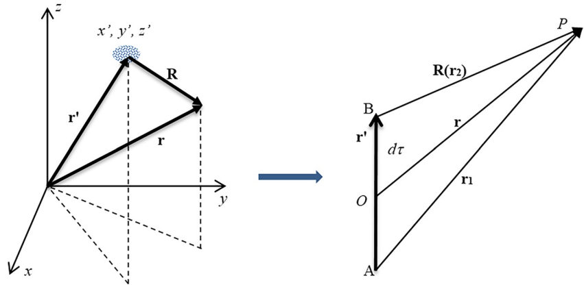
Figure 2. Coordinate system for computing radiation fields due to source domain not at origin (left); and vector potential A(r) at point P is calculated by integrating the current distribution J(r') throughout region d\tau . The source region is an electric dipole AB (right).
