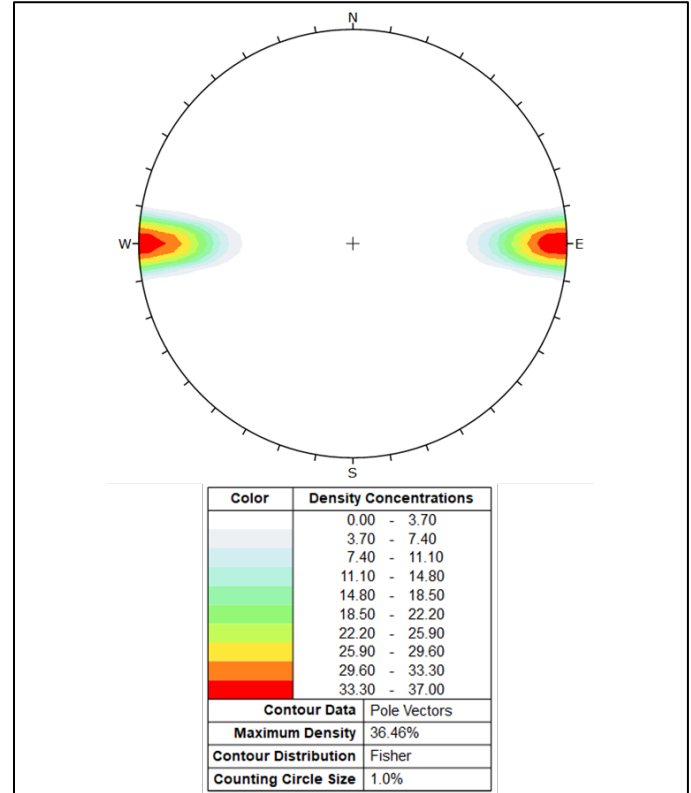
Figure 2. Lower hemisphere stereonet of subvertical fractures in 3DEC model.
