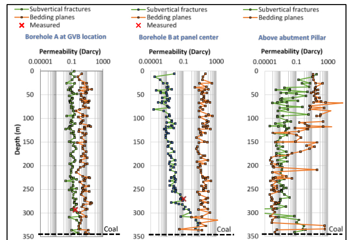
Figure 8. Results of modeled and measured permeability along the depth for when (a) first panel mining face is inby the test site at the GVB area in borehole A, (b) first panel mining face is outby the test site at the center of the first panel in borehole B. (c) the modeled permeabilities above the abutment pillar when second panel is outby the test site.
