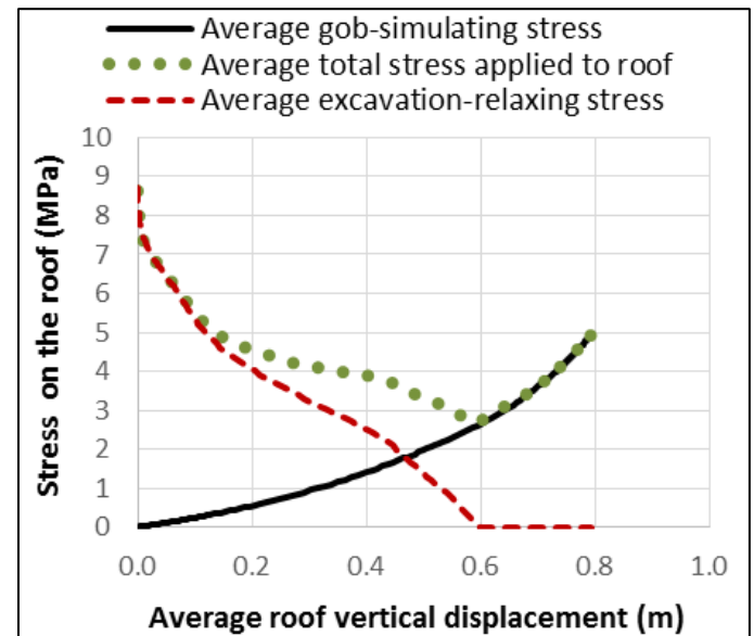
Figure 4. Boundary loads applied to the mine roof in 3DEC model.
