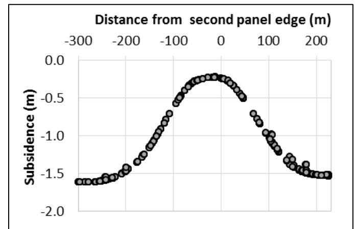
Figure 5. Surface subsidence calculated in the 3DEC model with a maximum subsidence of 1.63m.
