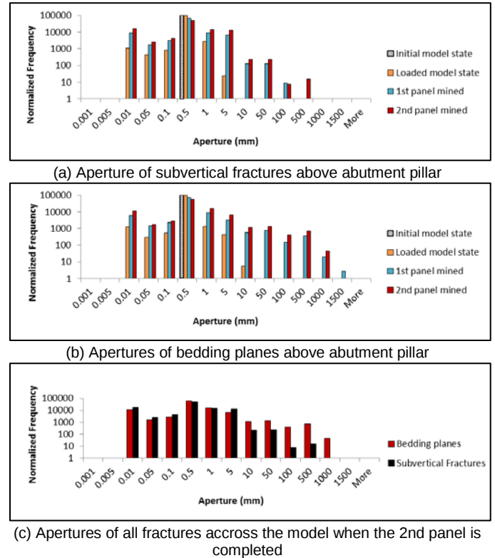
Figure 7. 3DEC results on the aperture values for (a) subvertical fractures and (b) bedding planes over the abutment pillar. (c) comparison of bedding planes and subvertical fracture apertures after mining the second panel.
