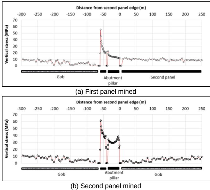
Figure 6. Modeled pillar vertical stress (a) after mining the first panel and (b) after mining the second panel. The gob stress approaches the vertical in-situ stress, 9 MPa, at the mine level.
