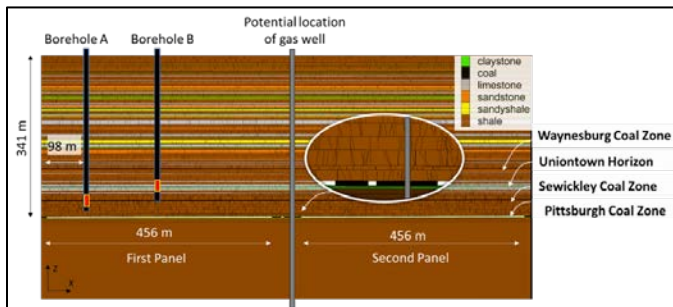
Figure 1. Details of the central part of the 3DEC model of the deep longwall mine with DFN elements defining rockmass structures in 105 modeled lithologies. Boreholes A and B and their permeability test intervals are shown along with the potential location of a gas well in the abutment pillar.
