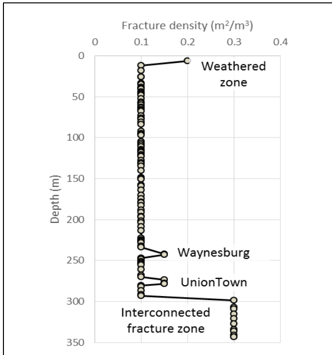
Figure 3. DFN density applied to generate subvertical fractures.
