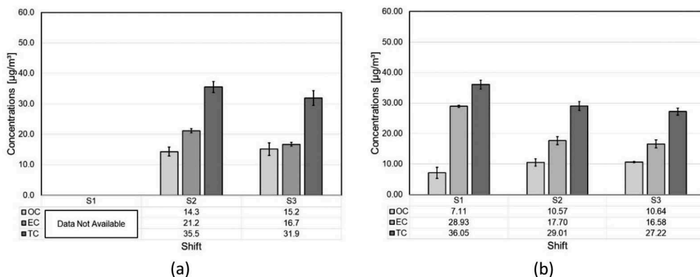
Figure 5. Average OC, EC, and TC concentrations at: (a) CM OMS and (b) LW OMS.
