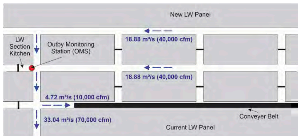
Figure 2. The longwall (LW) section.
