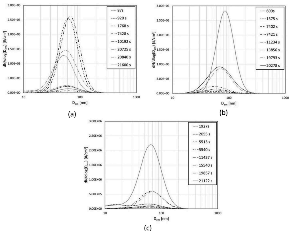
Figure 4. Size distributions of aerosols at CM OMS for: (a) S1, (b) S2, and (c) S3.
