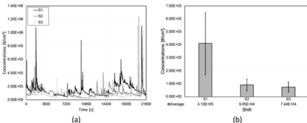
Figure 3. Number concentrations of aerosols measured with the FMPS at CM during S1, S2, and S3 shifts: (a) traces, and (b) average concentrations.
