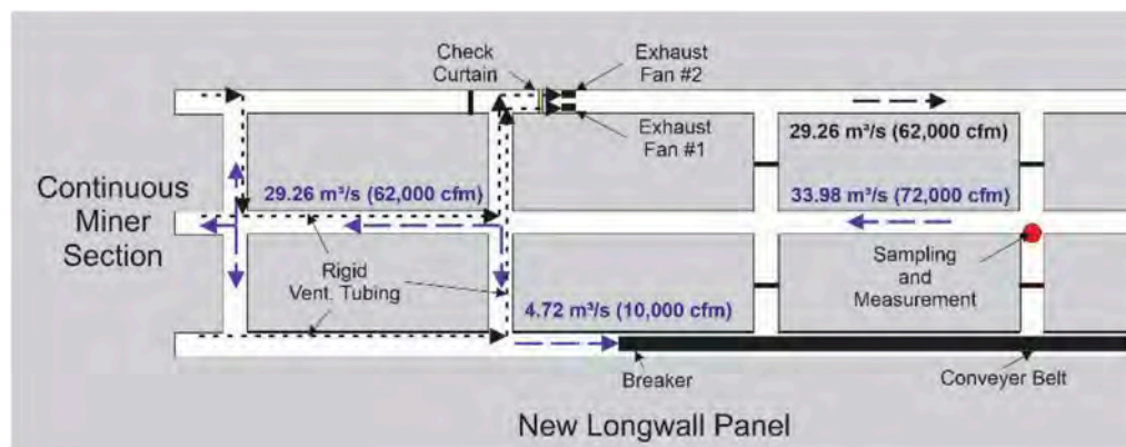
Figure 1. The continuous miner (CM) section.
