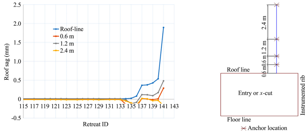
Fig. 15. Measured roof displacement at site-2 and schematic for anchor locations.
