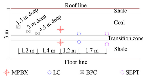
Fig. 5. Instrumentation type and location for the cross-cut side of instrumented pillar at site-1.
