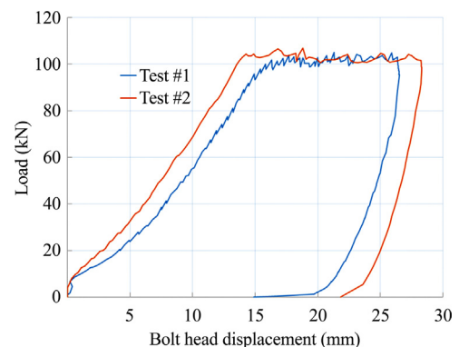
Fig. 9. Typical load displacement curve for the pull-out test.
