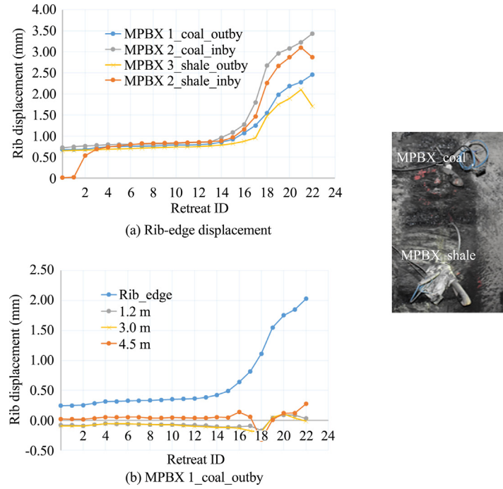
Fig. 13. Measured rib displacement at rib edge and multi-anchor points inside the pillar for the entry side at site-1.
