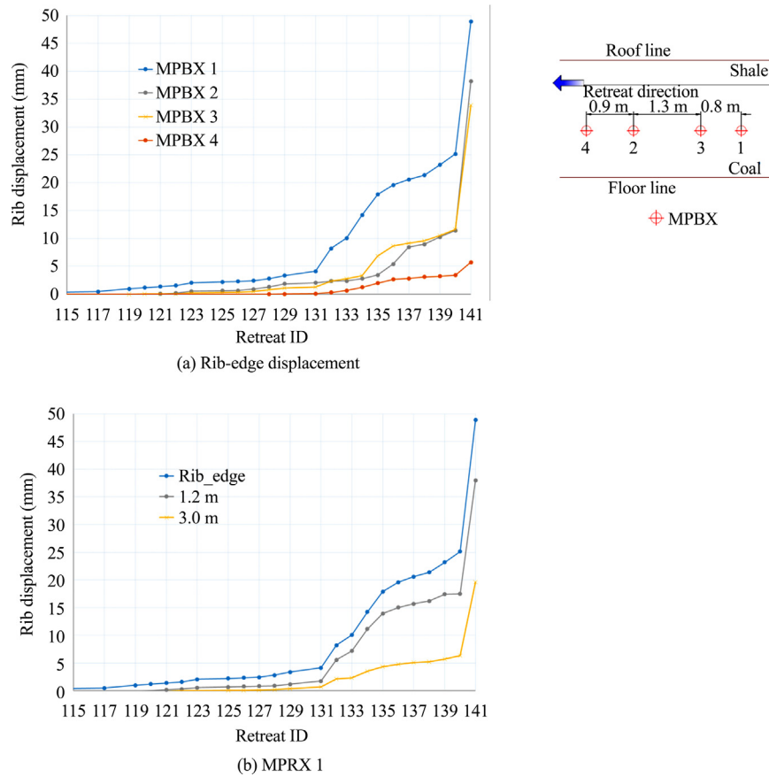
Fig. 14. Measured rib deformation at rib edge and multi-anchor points inside the pillar for the entry side at site-2.
