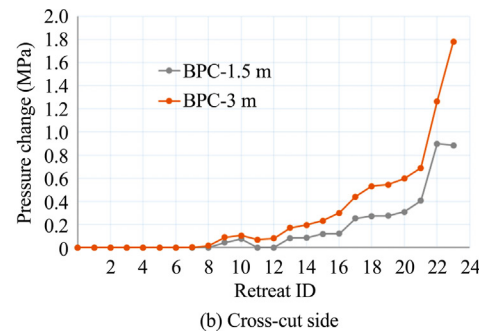
Fig. 10. Pressure change in the BPCs for the entry and cross-cut sides at site-1.
