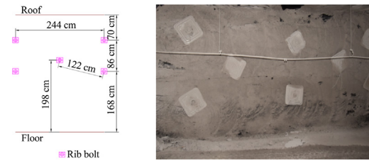
Fig. 2. Typical rib support pattern at site-1 for a mining height of more than 2.1 m.
