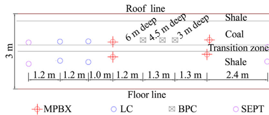
Fig. 4. Instrumentation type and location for the entry side of the instrumented pillar at site-1.
