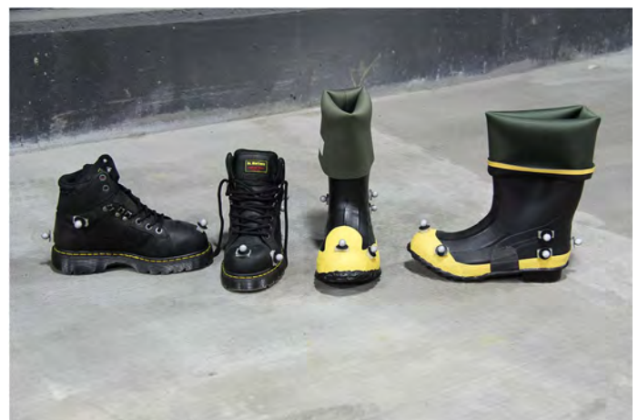
Figure 1 — Four styles of work boots worn by participants during the study, including (left to right): Hiker style with metatarsal, hiker style with steel toe, wader style with metatarsal, and wader style with steel toe.
