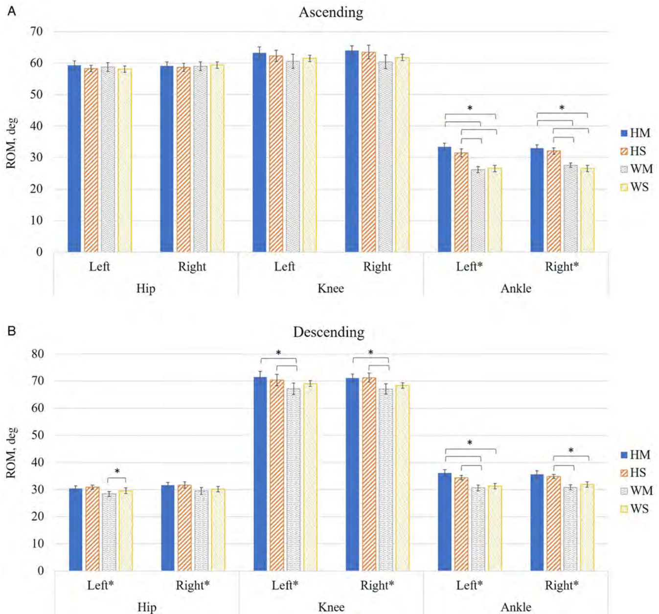
Figure 5 — Lower limb ROM by boot style and side when (A) ascending and (B) descending the walkway across incline level conditions. Error bars show SEs of the mean. HM indicates hiker style with metatarsal; HS, hiker style with steel toe; ROM, range of motion; WM, wader style with metatarsal; WS, wader style with steel toe. *Significant main effects or post hoc comparisons.
