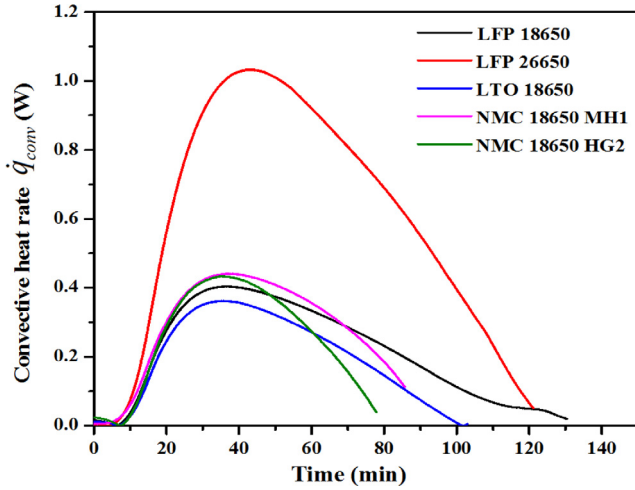
Fig. 6. Convective heat transfer to the battery surface.
