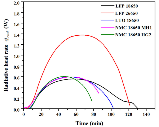
Fig. 5. Radiative heat transfer from the wall to the battery surface.
