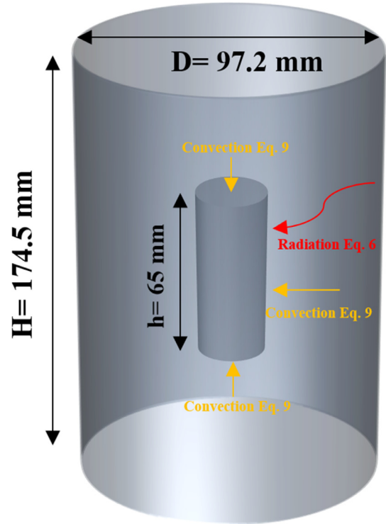
Fig. 4. Radiation and convection heat transfer to the battery.
