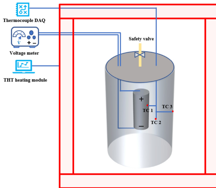
1c. Schematic setup of the test
