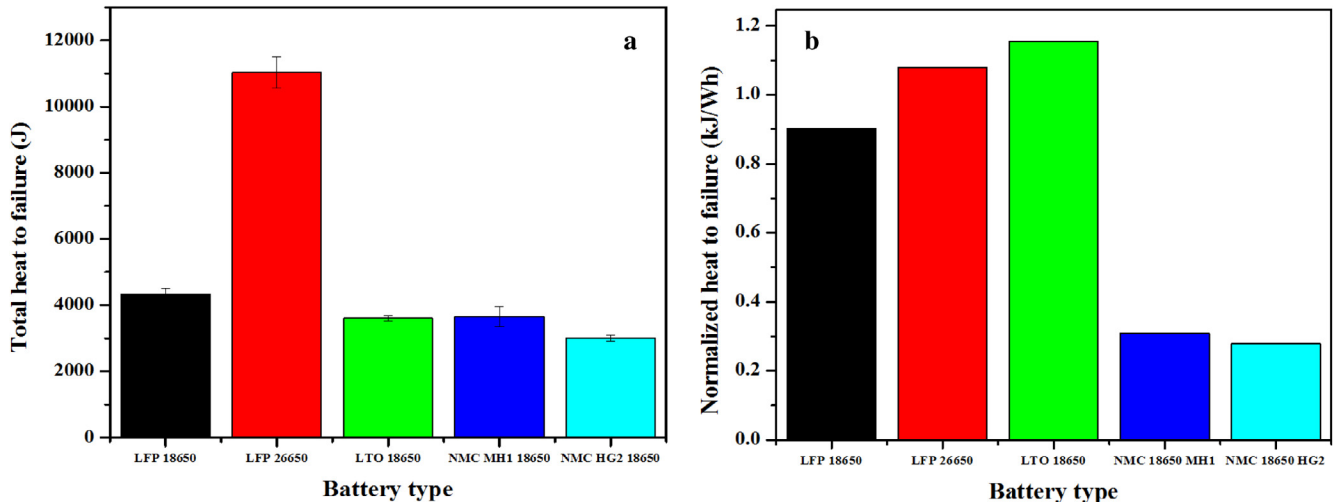
Fig. 7. (a) Total heat to failure for batteries of different types, (b) Normalized heat to failure by battery nominal energy capacity.
