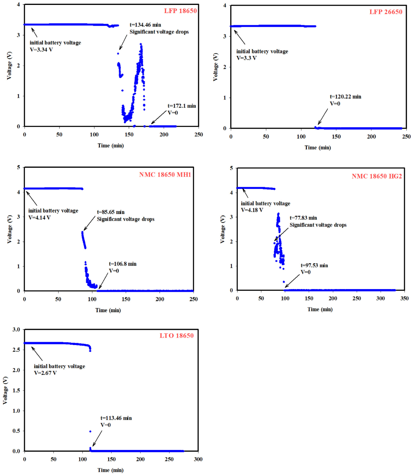
Fig. 2. Battery voltage changes in thermal tests.
