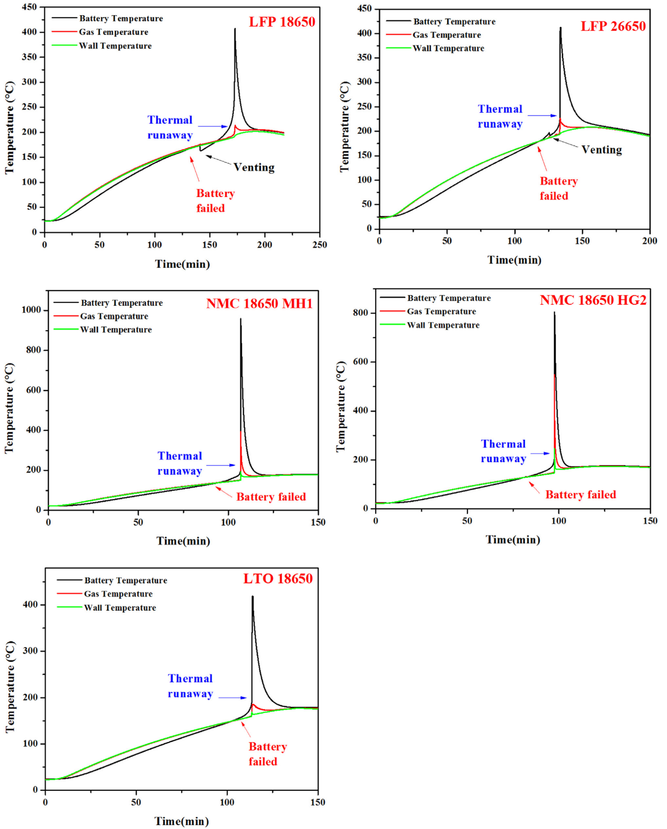
Fig. 3. Battery surface, gas, and wall temperatures during ARC tests.
