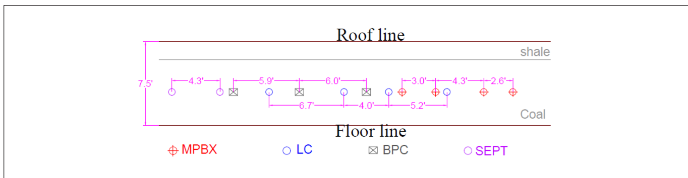
Figure 6. Instrumentation type and location for entry side of the instrumented pillar at Site 2.
