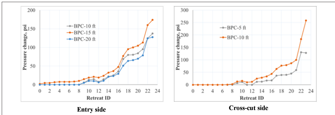
Figure 10. Pressure change in the BPCs for the entry and crosscut sides at Site 1.
