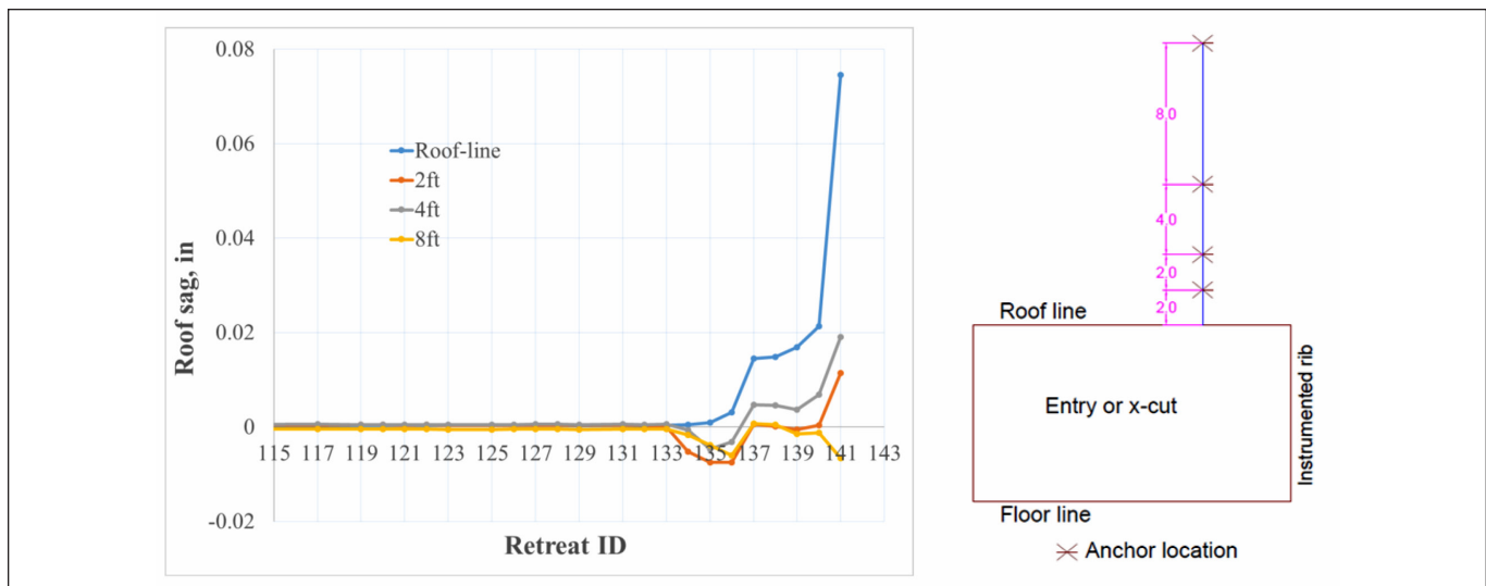
Figure 15. Measured roof displacement at Site 2 and schematic for anchor locations.
