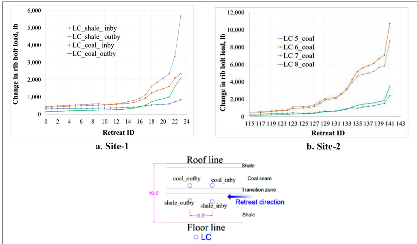
Figure 12. Change in rib-bolt load for the entry side at Site 1 and Site 2.
