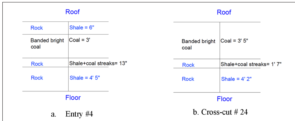
Figure 1. Rib profiles of the study pillar at an instrumented Site 1.
