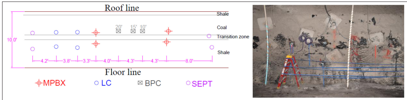
Figure 4. Instrumentation type and location for the entry side of the instrumented pillar at Site 1.
