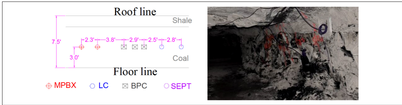
Figure 7. Instrumentation type and location for the crosscut side of the instrumented pillar at Site 2.
