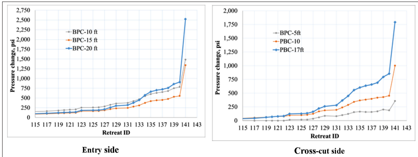
Figure 11. Pressure changes in the BPCs for the entry and crosscut sides at Site 2.
