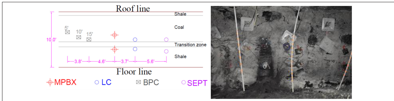
Figure 5. Instrumentation type and location for the crosscut side of instrumented pillar at Site 1.
