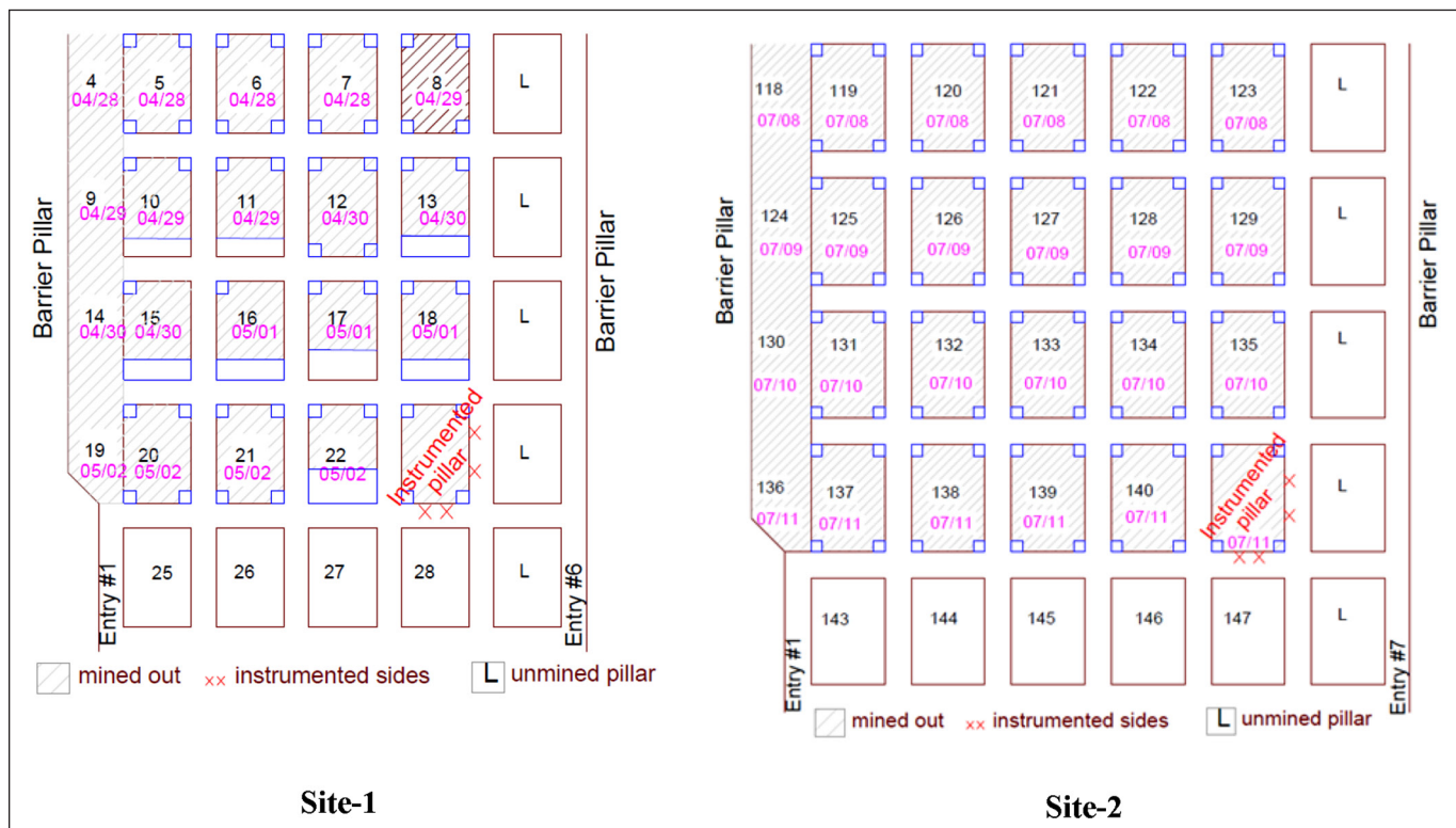
Figure 8. Retreat plan and cutting sequence at Site 1 and Site 2.
