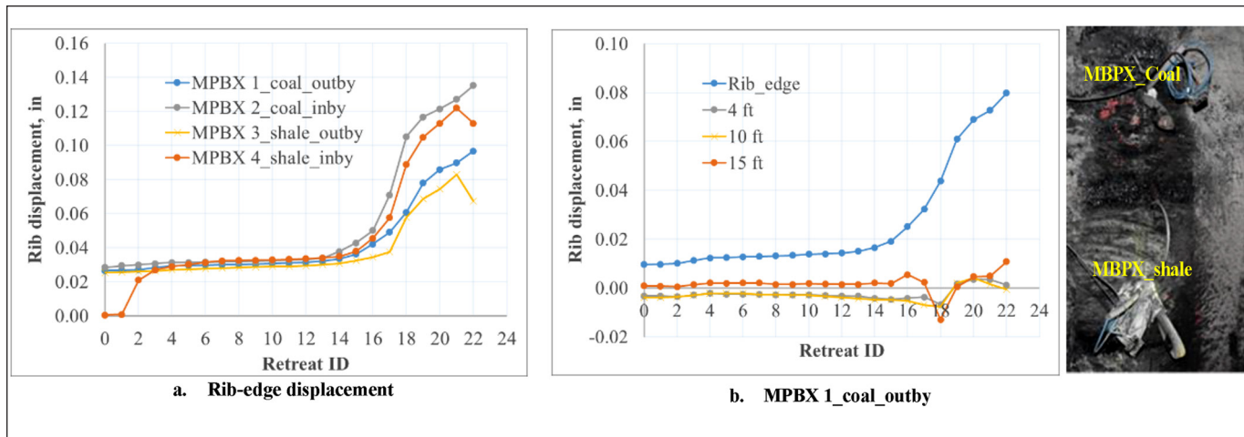
Figure 13. Measured rib displacement at (a) rib edge and (b) multi-anchor points inside the pillar for the entry side at Site 1.
