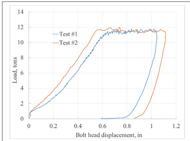
Figure 9. Typical load displacement curve for the pull-out test.
