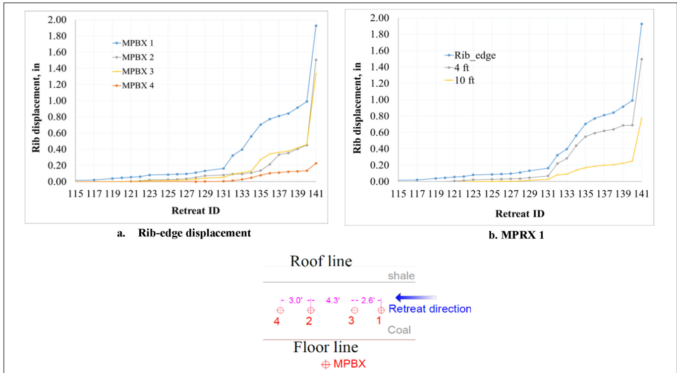
Figure 14. Measured rib deformation at (a) rib edge and (b) multi-anchor points inside the pillar for the entry side at Site 2.
