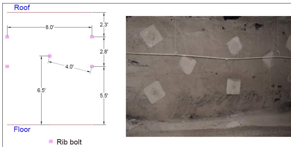
Figure 2. Typical rib support pattern at Site 1 for a mining height of more than 7 ft.
