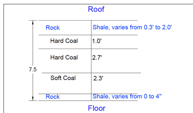
Figure 3. Rib profile of the study pillar at instrumented Site 2.
