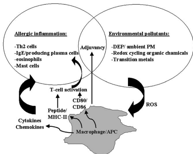
Fig. 6. Schematic to explain the molecular basis for the adjuvant effect of DEP at the level of the antigen-presenting cell (APC). Oxidative stress induces cytokines and chemokines that contribute to allergic inflammation through effects on T cells, B cells, and eosinophils. In addition, oxidative stress assists in the expression of costimulatory receptors (CD80, CD86) as well as enhancing antigen processing. This increases antigen-specific T-helper 2 cells responsiveness. These interactions likely only require a limited mucosal area to lead to allergen-specific IgE production. Once sensitized to an allergen, re-exposure may lead to widespread allergic inflammation in the bronchial mucosa.
