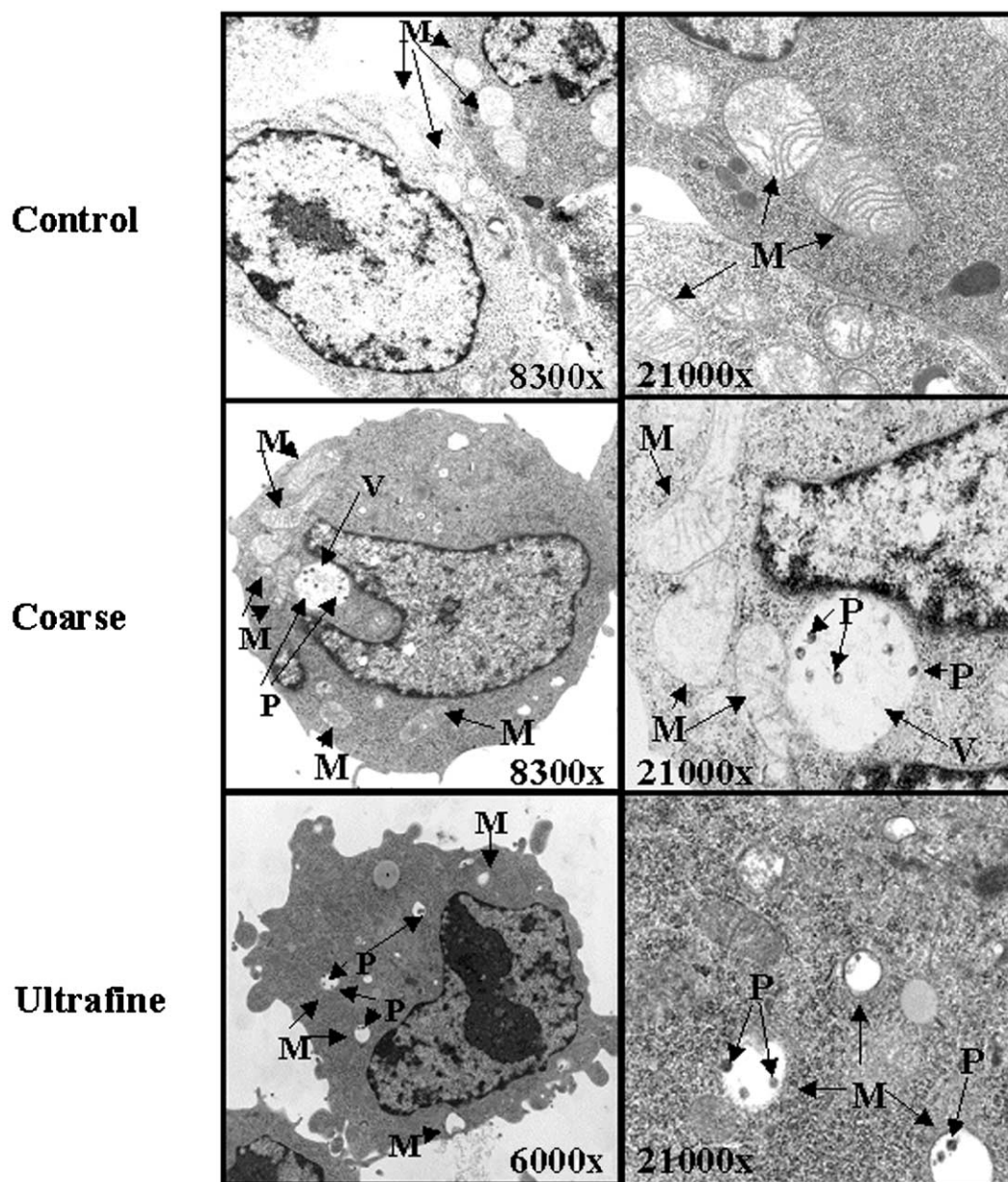
Fig. 7. Electron microscopy (EM) showing select subcellular localization of ultrafine and coarse particles. Coarse (2.5–10 \mu\text{m} ) and ultrafine (<0.15 \mu\text{m} ) CAPs were collected in an aqueous medium in Claremont, CA, using the VACES [84]. RAW264.7 cells were incubated with these particles for 16 h before fixation. EM was performed as previously described [84]. While coarse CAPs are localized in large vacuoles (phagosomes?) and do not damage mitochondria, ultrafine particles often induce structural damage as demonstrated by the disappearance of cristae. In addition, ultrafine particles appear to lodge inside damaged mitochondria. M, mitochondria; P, particles; V, vacuoles.
