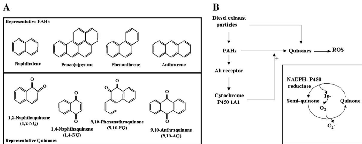
Fig. 2. Redox cycling organic compounds. (A) Representative PAH and quinone compounds. (B) PAH can be converted to quinones through the action of cytochrome P450 1A1 in the cells. This cytochrome is expressed via the aryl hydrocarbon (Ah) receptor. One-electron reduction of quinones results in the formation of semiquinones, which can be recycled to a quinone. In the process, the electron is donated to molecular O 2 , leading to the formation of O 2 -• .
