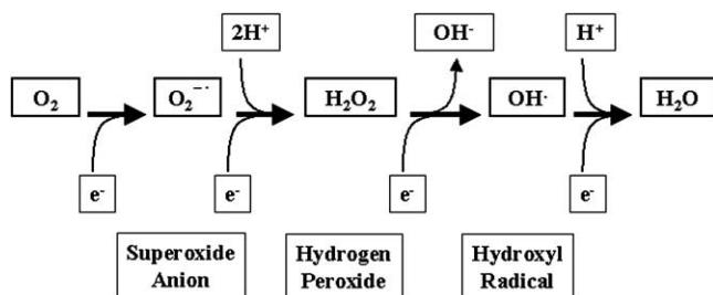
Fig. 1. ROS generation during oxidative phosphorylation. In this process, O_2 receives 4 electrons to form H_2O . Occasional 1-electron additions result in the formation of O_2^{\bullet -} , which can be converted to H_2O_2 or OH^{\bullet} .
