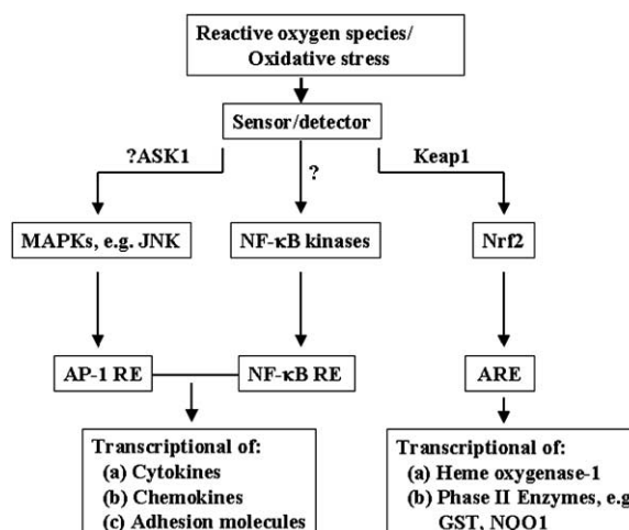
Fig. 5. Cellular sensors and signaling pathways involved in oxidative stress. ROS generation and/or oxidative stress is detected by cellular sensors. The possible candidates for the sensors include ASK1 for the AP-1 pathway and Keap-1 for the ARE pathway. These afferent components activate the MAP kinase cascade and, in the case of Keap1, lead to the release of the transcription factor, Nrf2, to the nucleus. The sensor for the NF-κB cascade is unknown, but ultimately leads to the phosphorylation and degradation of I-κBα, thereby releasing the attached Rel protein to the nucleus. Binding of AP-1 and/or NF-κB transcription factors to their respective DNA binding sites eventually leads to the production of cytokines, chemokines, and adhesion molecules. These products exert proinflammatory effects. The binding of Nrf2 to the ARE results in the expression of HO-1 (antioxidative) and phase II (detoxifying) enzymes. These products are cytoprotective.
