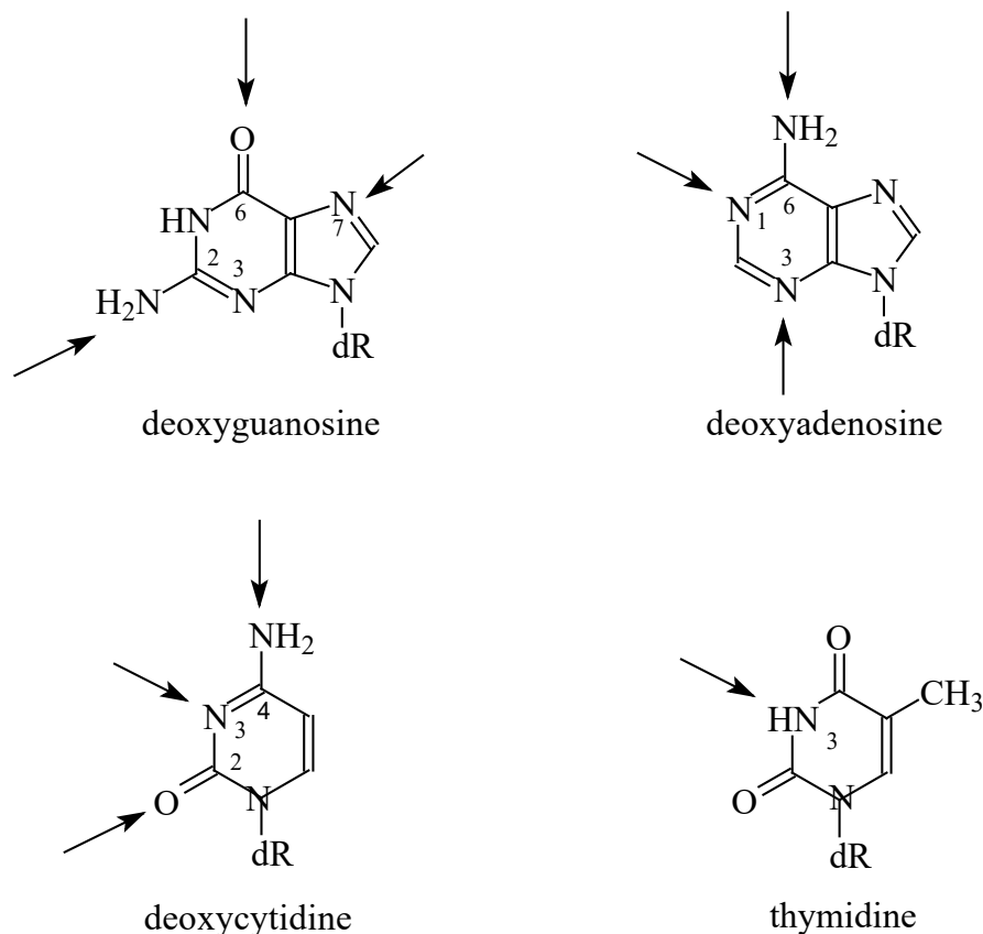
Fig. 4.3 Nucleophilic sites in DNA bases found to be covalently modified by styrene-7,8-oxide
