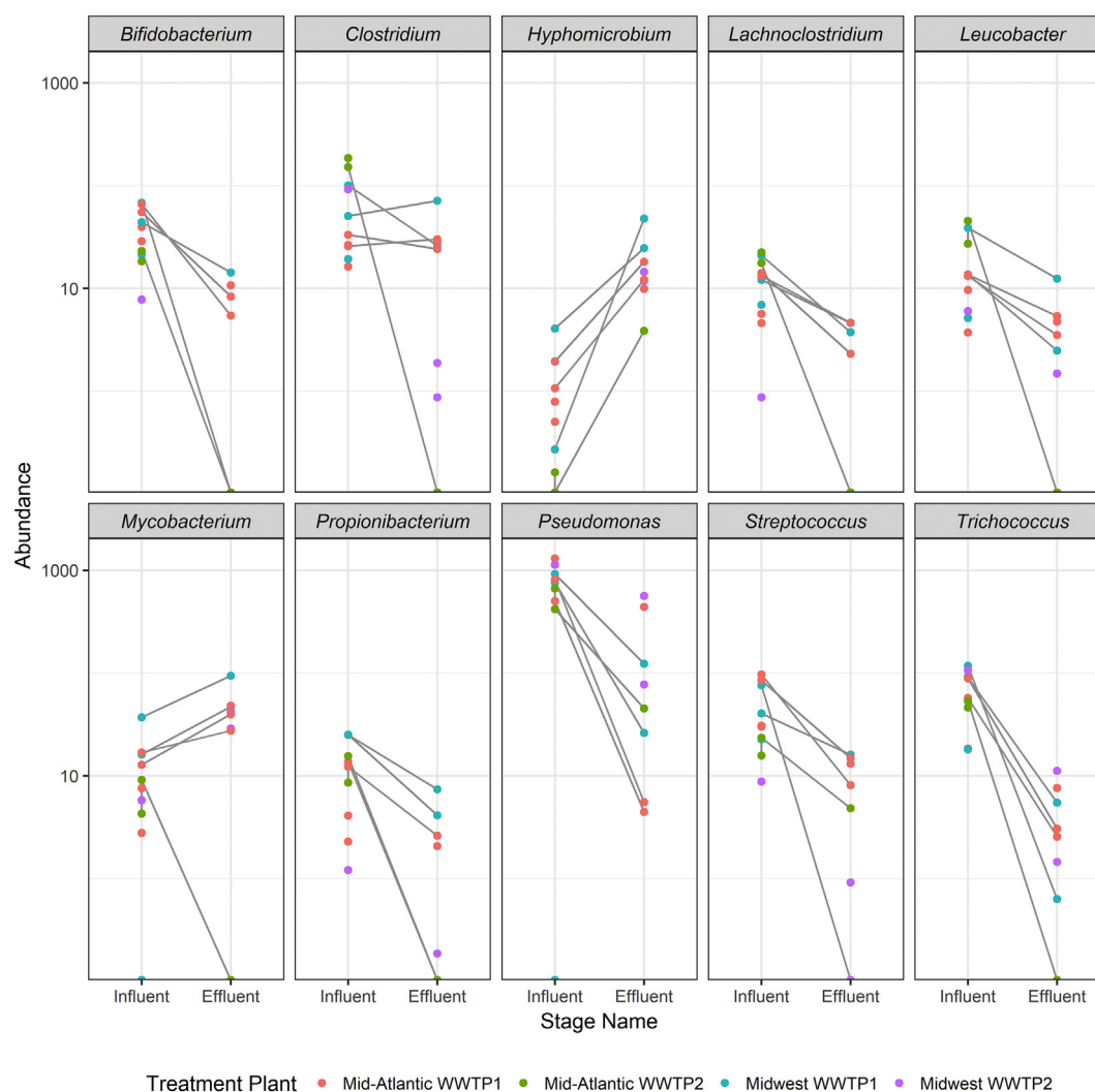
Fig. 3. Significant differentially abundant ( p < 0.01 ) bacterial genera across same-day influent-effluent pairs from all four wastewater treatment plants. The cumulative sum scaling (CSS) normalized counts are depicted on the y axis (Abundance) and the corresponding sample type on the x axis. Grey lines link influent-effluent samples collected on the same day. Except for one collection date, the relative abundance of Mycobacterium was higher in effluent samples compared to influent samples.
