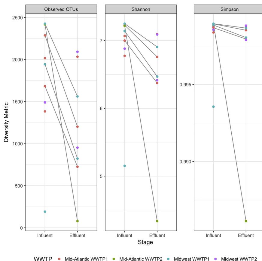
Fig. 2. Alpha-diversity estimates and observed number of operational taxonomic units (OTUs) in same-day influent-effluent pairs from all four wastewater treatment plants. Observed number of OTUs was significantly ( p < 0.01 ) higher in influent samples compared to effluent samples.
