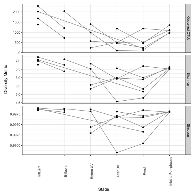
Fig. 6. Alpha-diversity estimates and observed number of OTUs in samples from the influent stage at Mid-Atlantic WWTP1 to the inlet to the pumphouse stage at Mid-Atlantic SI1. Significant differences in alpha-diversity estimates were found for Shannon index ( p < 0.01 ) and observed number of OTUs ( p < 0.01 ) with alpha-diversity decreasing with wastewater plant treatment and ultraviolet treatment at the spray irrigation site, but increasing after storage in an open-air pond at the spray irrigation site.
