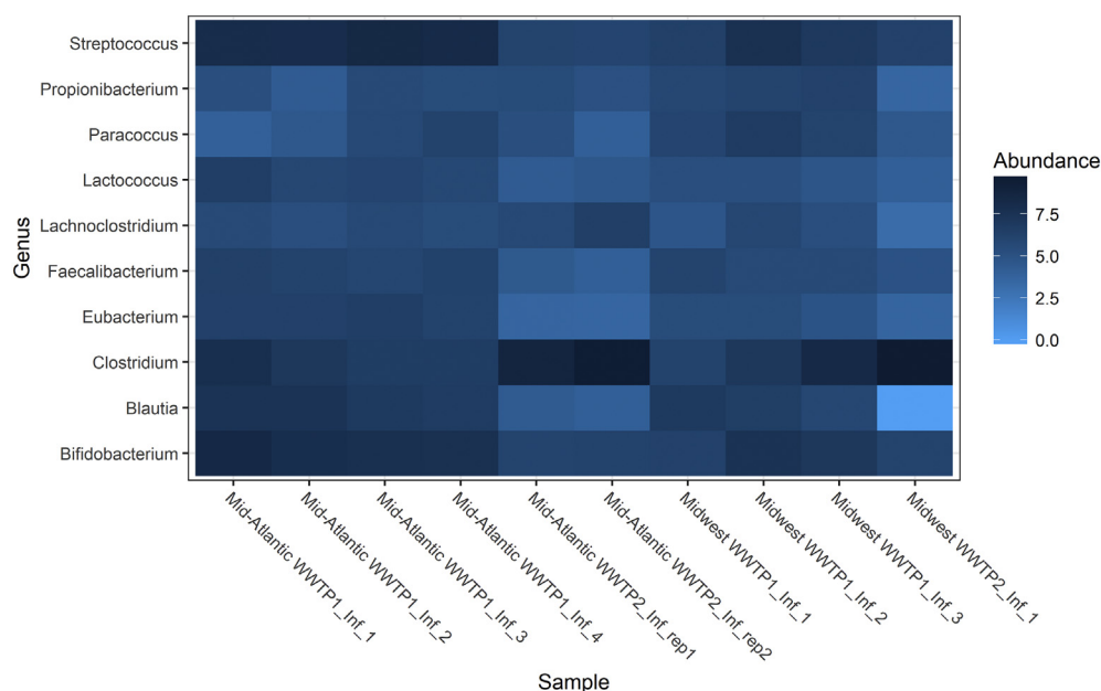
Fig. 1. Heatmap showing genera with significant ( p < 0.01 ) differences in abundance between influent samples collected from each of the four wastewater treatment plants. Genera that were highly abundant have been depicted in darker shades of blue while those that were less abundant are depicted in lighter shades of blue.
