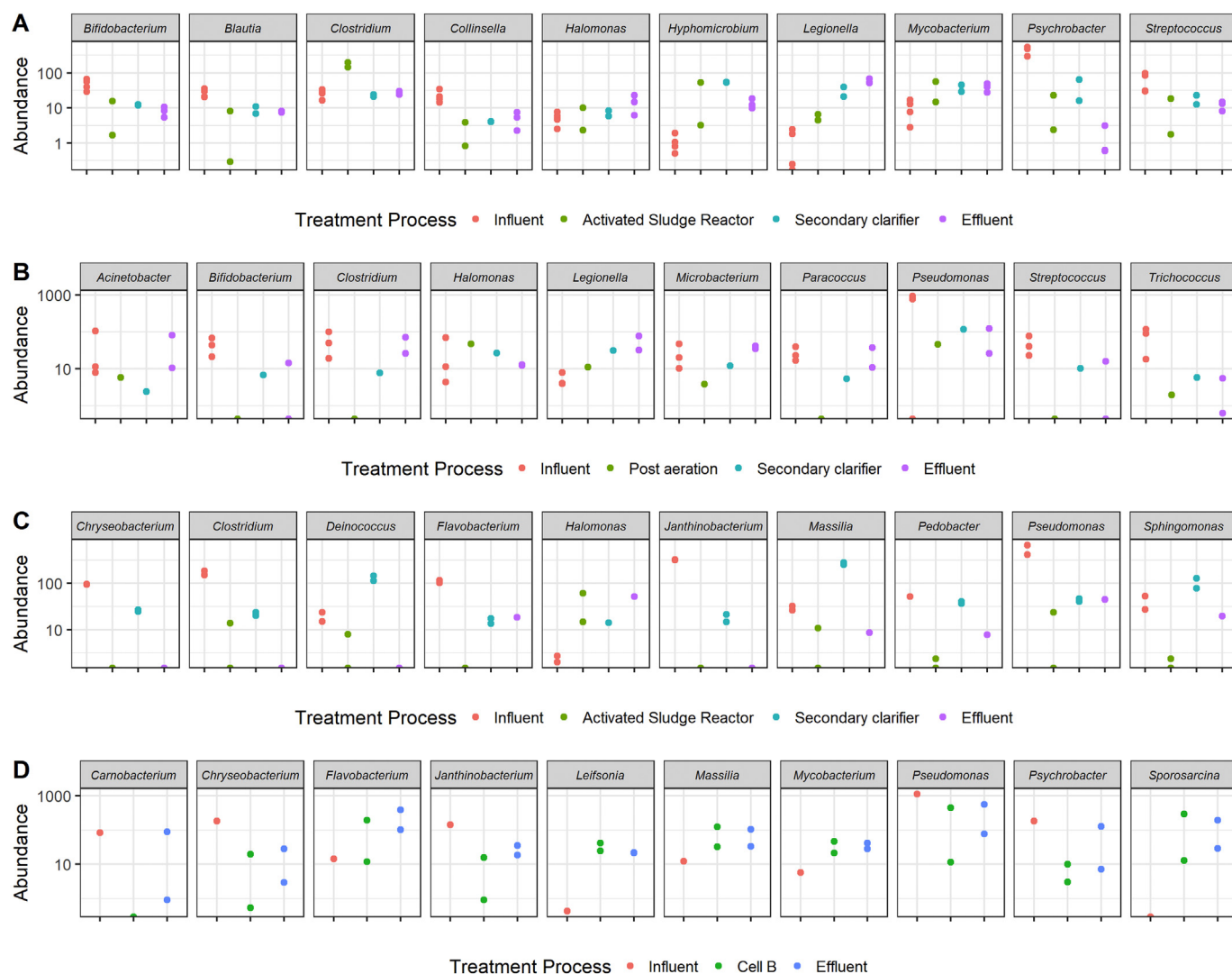
Fig. 5. A–D Significant differentially abundant ( p < 0.01 ) bacterial genera (top 10) across the various treatment processes performed at Mid-Atlantic WWTP1 (5A), Mid-Atlantic WWTP2 (5B), Midwest WWTP1 (5C) and Midwest WWTP2 (5D). For each WWTP, the cumulative sum scaling (CSS) normalized counts are depicted on the y axis (Abundance) and the corresponding treatment process on the x axis.
