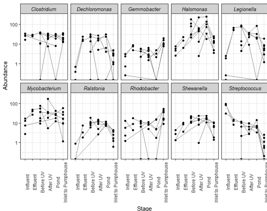
Fig. 8. Significant differentially abundant ( p < 0.01 ) bacterial genera (top 10) from treatment at Mid-Atlantic WWTP1 through transport to, treatment and storage at Mid-Atlantic SI1. The cumulative sum scaling (CSS) normalized counts are depicted on the y axis (Abundance) and the corresponding stage on the x axis.
