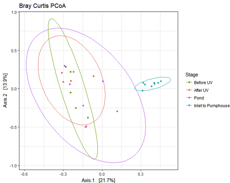
Fig. 7. First two coordinates of the Principal Coordinate Analysis (PCoA) using Bray-Curtis dissimilarity showing samples from the inlet to the pumphouse clustering apart (ANOSIM statistic R: 0.5802 p < 0.01 ) from samples after on-site ultraviolet treatment ("before UV" and "after UV") and on-site open-air storage ("pond"). Axis labels include the percent of the total variance in the data explained by the coordinate.
