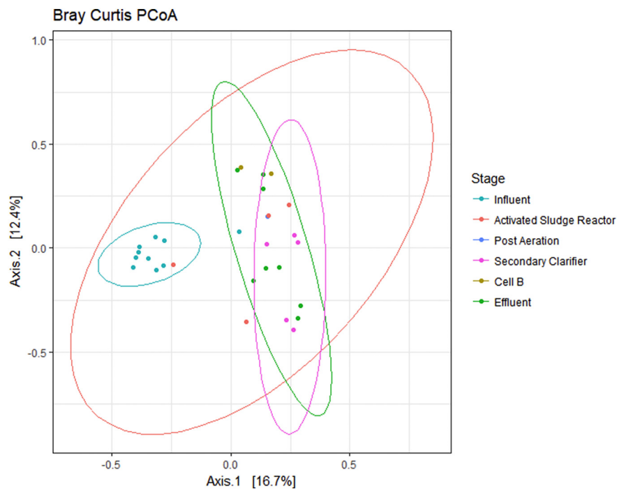
Fig. 4. First two coordinates of the Principal Coordinates Analysis (PCoA) using Bray-Curtis dissimilarity, showing influent samples clustering apart (ANOSIM statistic R: 0.5632, p < 0.01 ) from samples collected from downstream wastewater treatment processes. Axis labels include the percent of total variance in the data explained by the coordinate.
