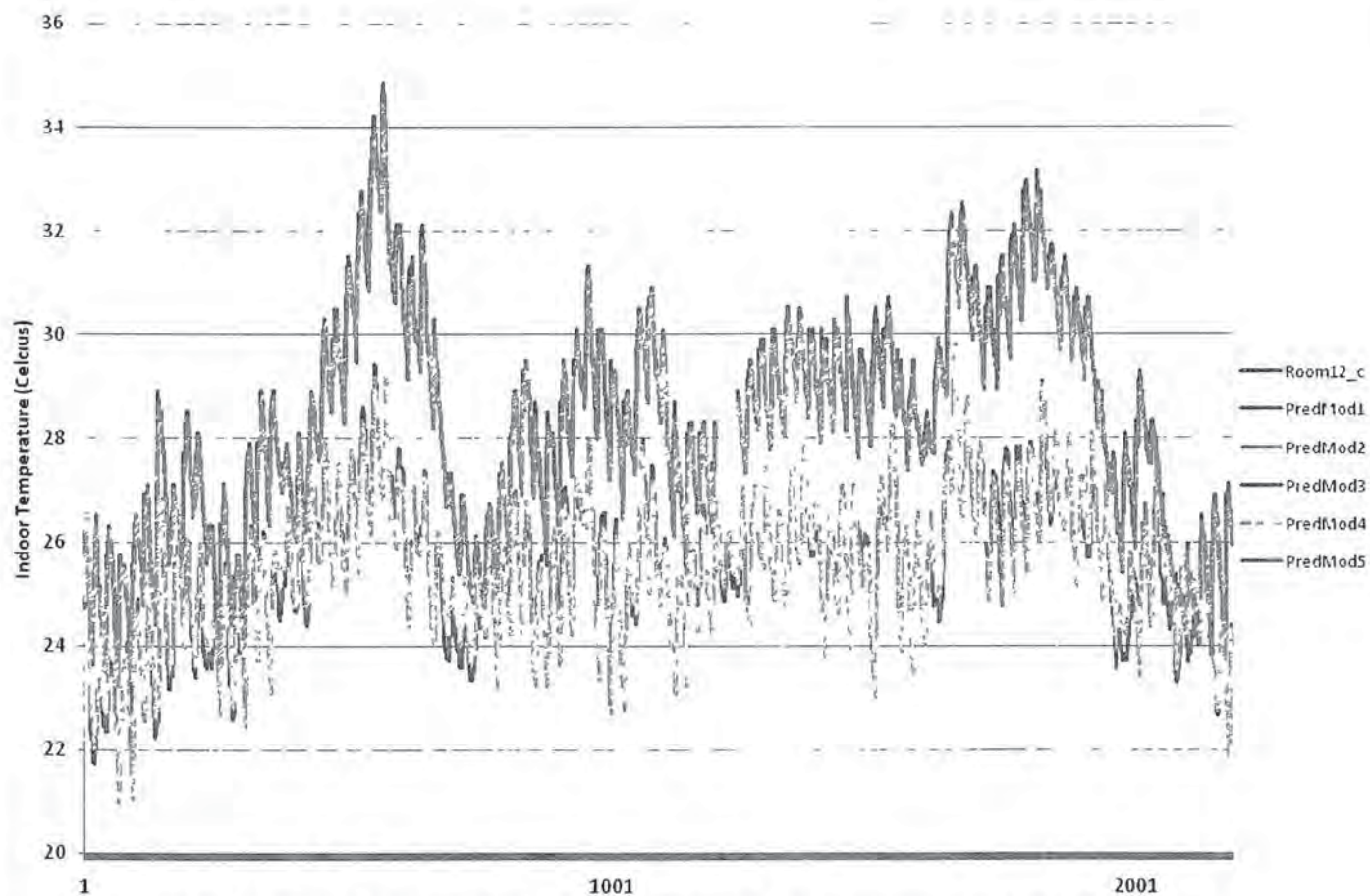
Appendix A2.3: Graph comparing predicted indoor temperatures for Location 8 using prediction modeling equations
