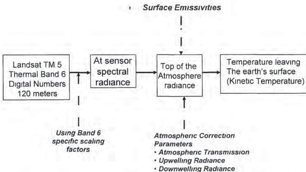
Figure 4-1 Processing method for converting raw satellite images to land surface temperature
