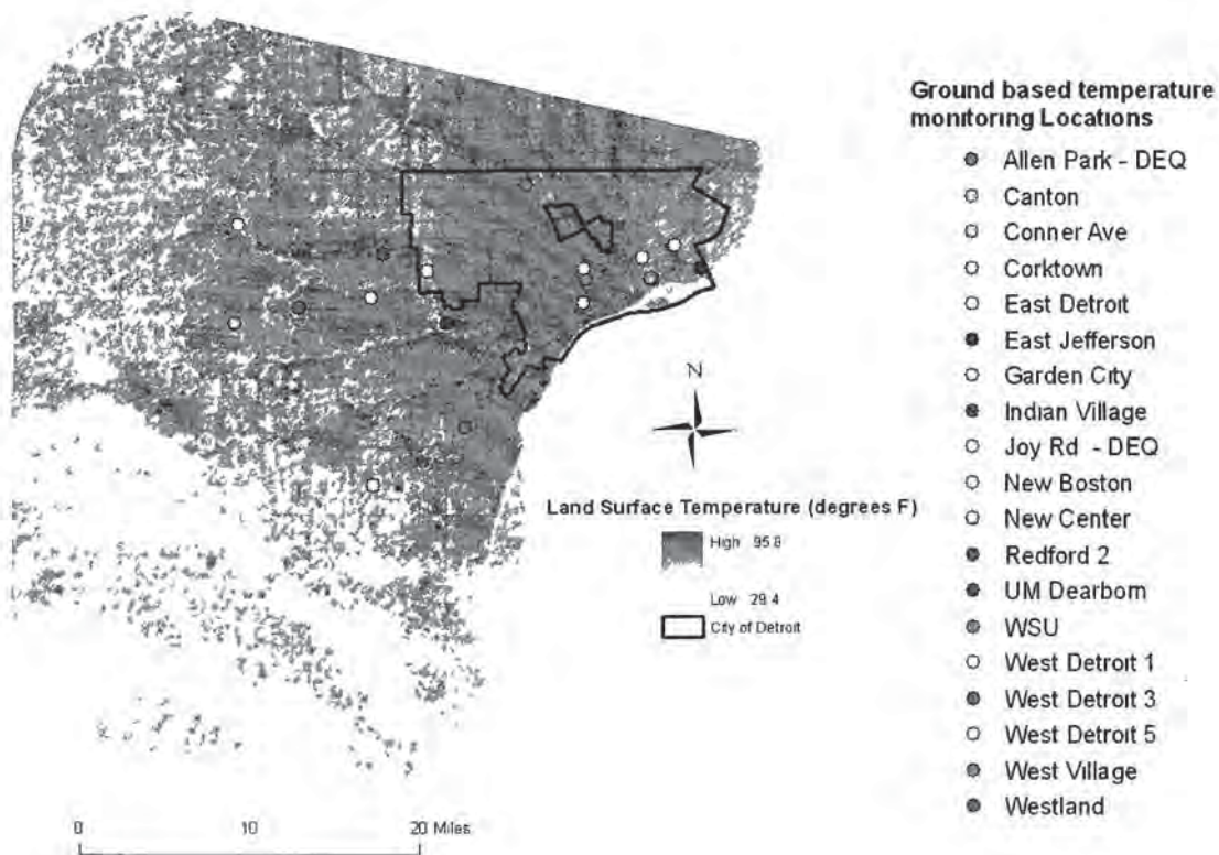
Figure 4-2 The final processed Landsat TM-5 satellite image that displays the satellite derived land surface temperatures (LSTs) for the study area of Wayne County, Michigan. The city of Detroit is outlined. The 19 locations of the ground based temperature monitoring network are also displayed.
