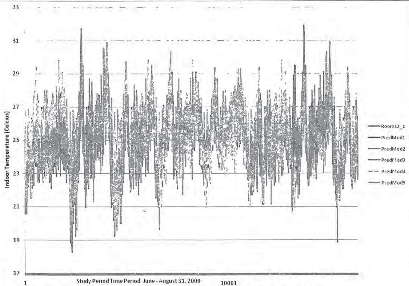
Appendix A2.5 Graph comparing predicted indoor temperatures for locations constructed of brick using prediction modeling equations
