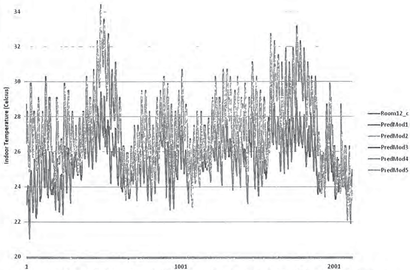
Appendix A2.2 Graph comparing predicted indoor temperatures for Location 13 using prediction modeling equations
