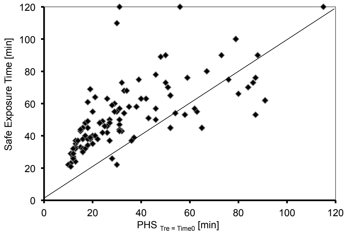
Figure 7. Relationship between PHS_{T_{re} = Time0} and the Safe Exposure Time (SET).
