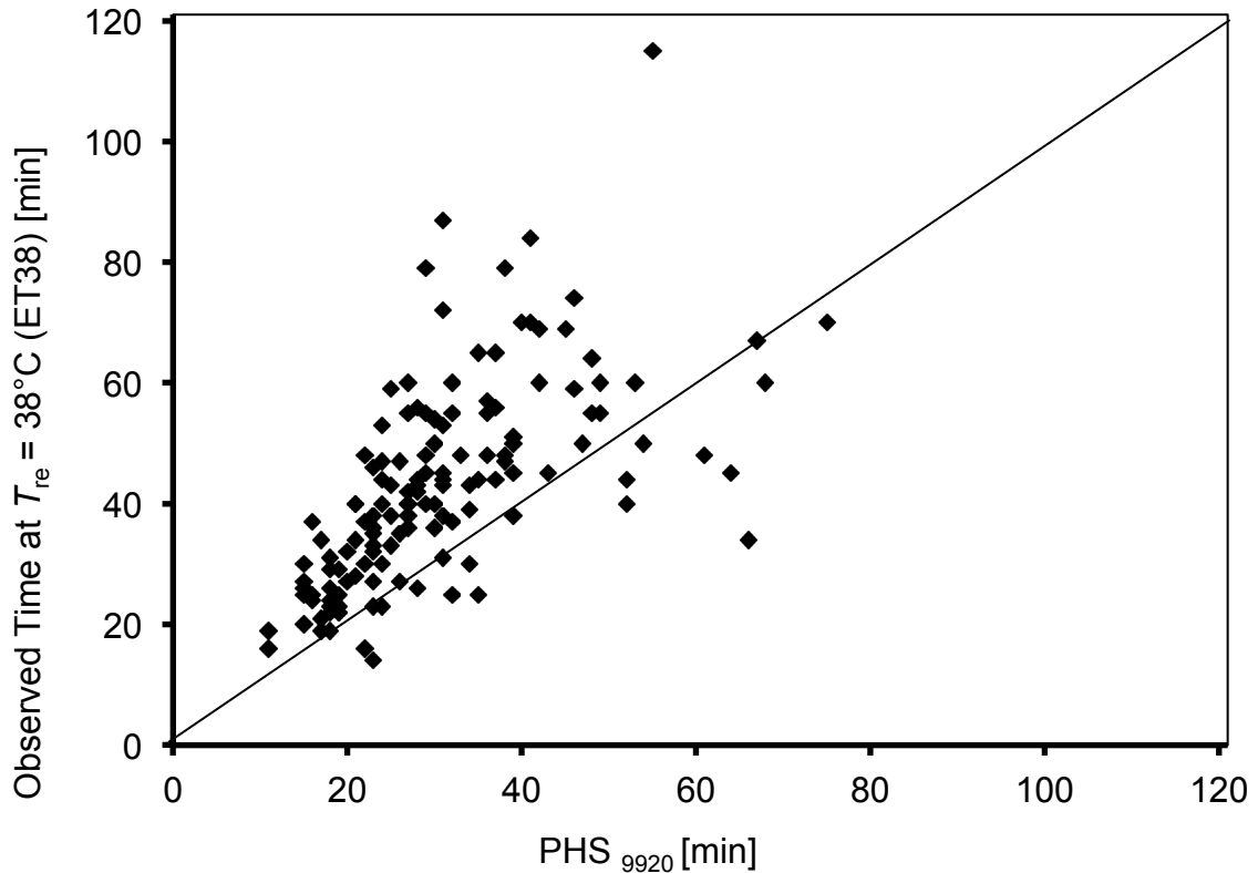
Figure 5. Relationship between PHS Time Limit Based on ISO9920 Methods for Clothing and the Observed Time at T_{re} = 38^{\circ}\text{C} (ET38).
