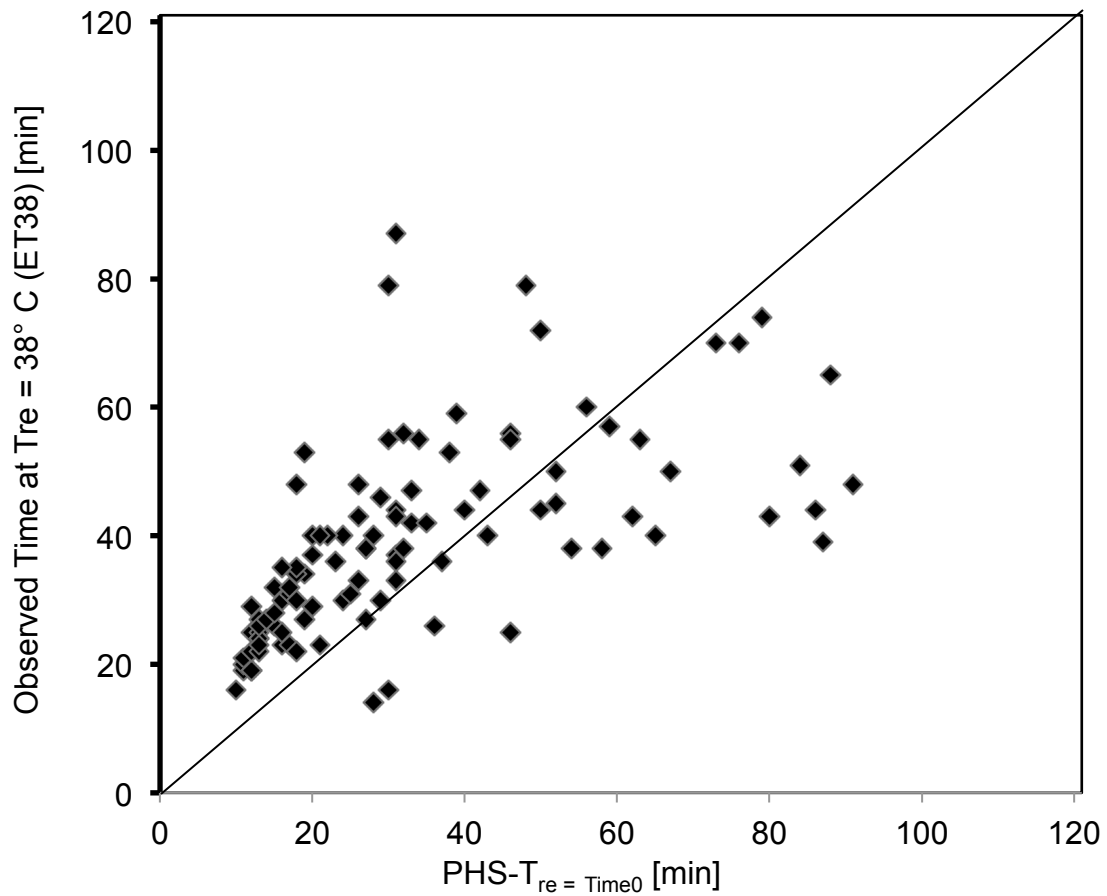
Figure 4. Relationship between PHS Time Limit Based on Initial T_{re} and the Observed Time at T_{re} = 38^{\circ}\text{C} (ET38).
