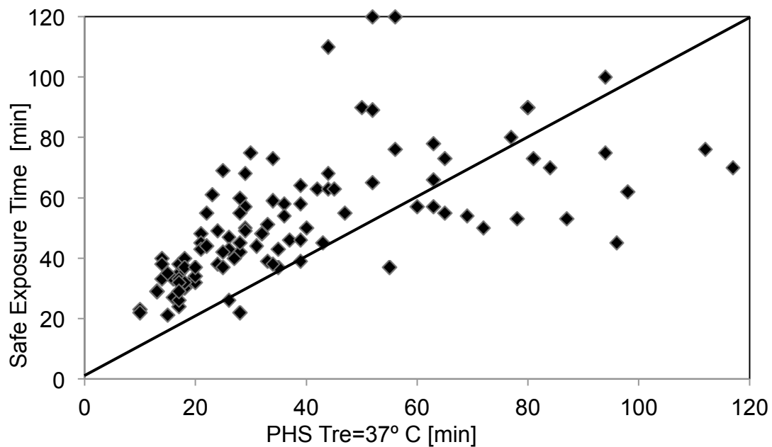
Figure 6. Relationship between \text{PHS}_{T_{re} = 37^{\circ}\text{C}} at Start and the Safe Exposure Time (SET).
