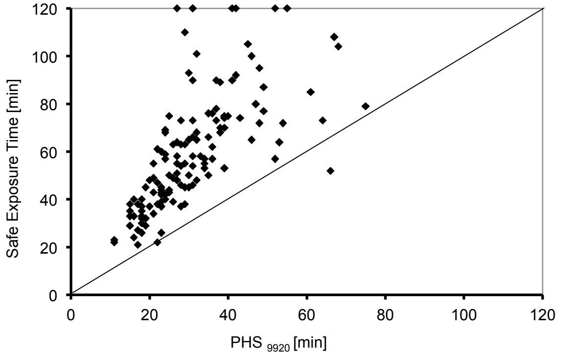
Figure 8. Relationship between PHS Standard modified with ISO 9920 Clothing Values ( PHS_{9920} ) and Safe Exposure Time (SET).
