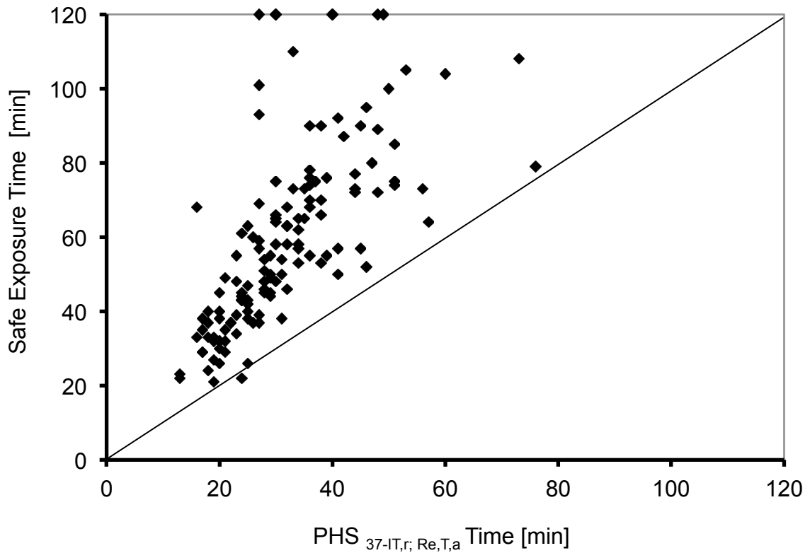
Figure 9 Relationship between PHS37 with I_{T,r} and R_{e,T,a} and Safe Exposure Time.
