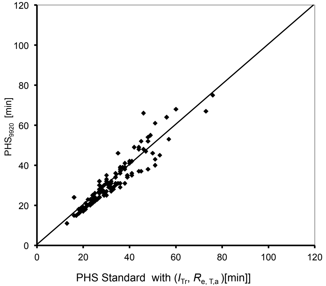
Figure 15. Comparison of PHS standard modified with substituted clothing values from ISO 9920 (2007) to the PHS standard modified with substituted ISO 9920 value for I_{Tr} and R_{e, T,a} from Caravello et.al.
