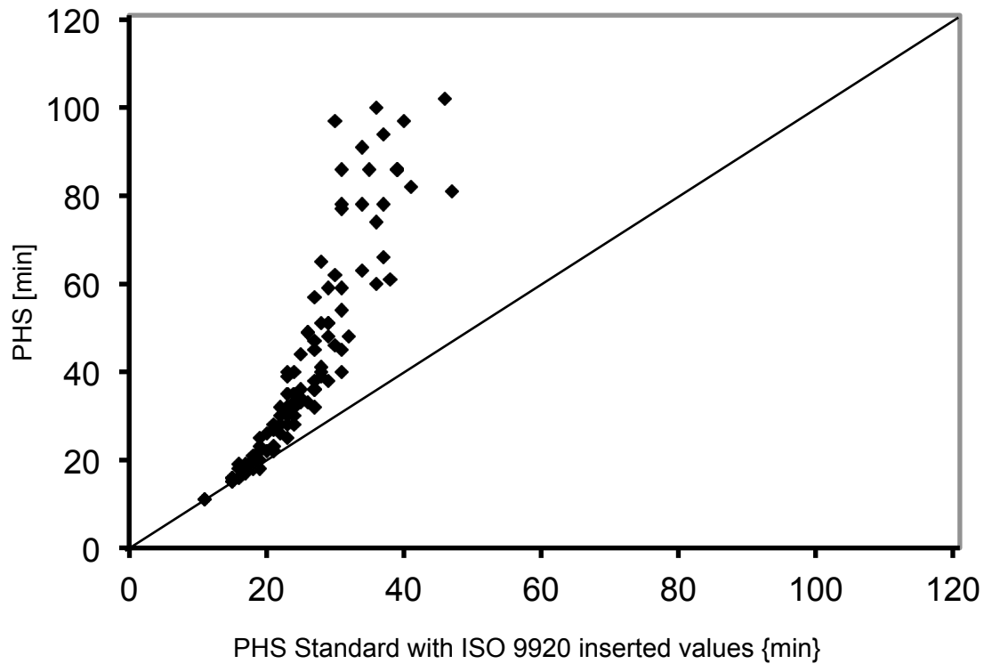
Figure 12. Comparison of PHS Standard modified with inserted value of ISO 9920 values ( PHS_{9920} ) compared to the PHS Standard Model ( PHS_{Std} ).
