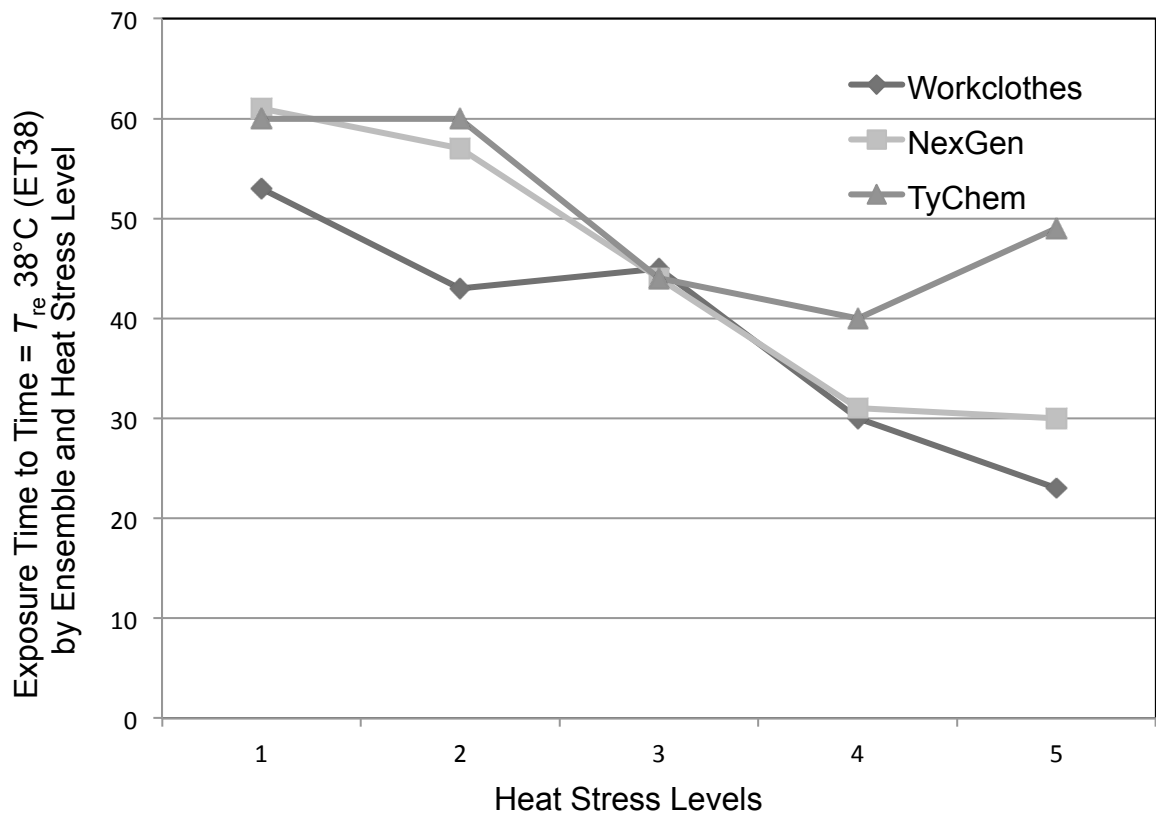
Figure 2. Exposure Time to T_{re} 38^{\circ}\text{C} (ET38) by Ensemble and Heat Stress Level
