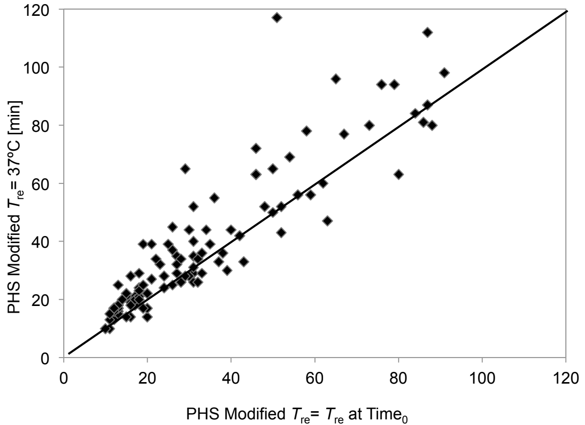
Figure 11. Comparison of PHS Standard modified with an inserted value of fixed T_{re} = 37^{\circ}\text{C} to PHS Standard modified with the actual T_{re} at Time 0 .
