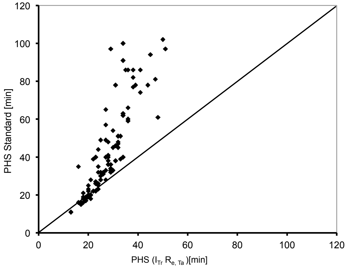
Figure 13. Comparison of PHS Standard model to the PHS Standard modified with inserted clothing values I_{Tr} and R_{e, Ta} .
