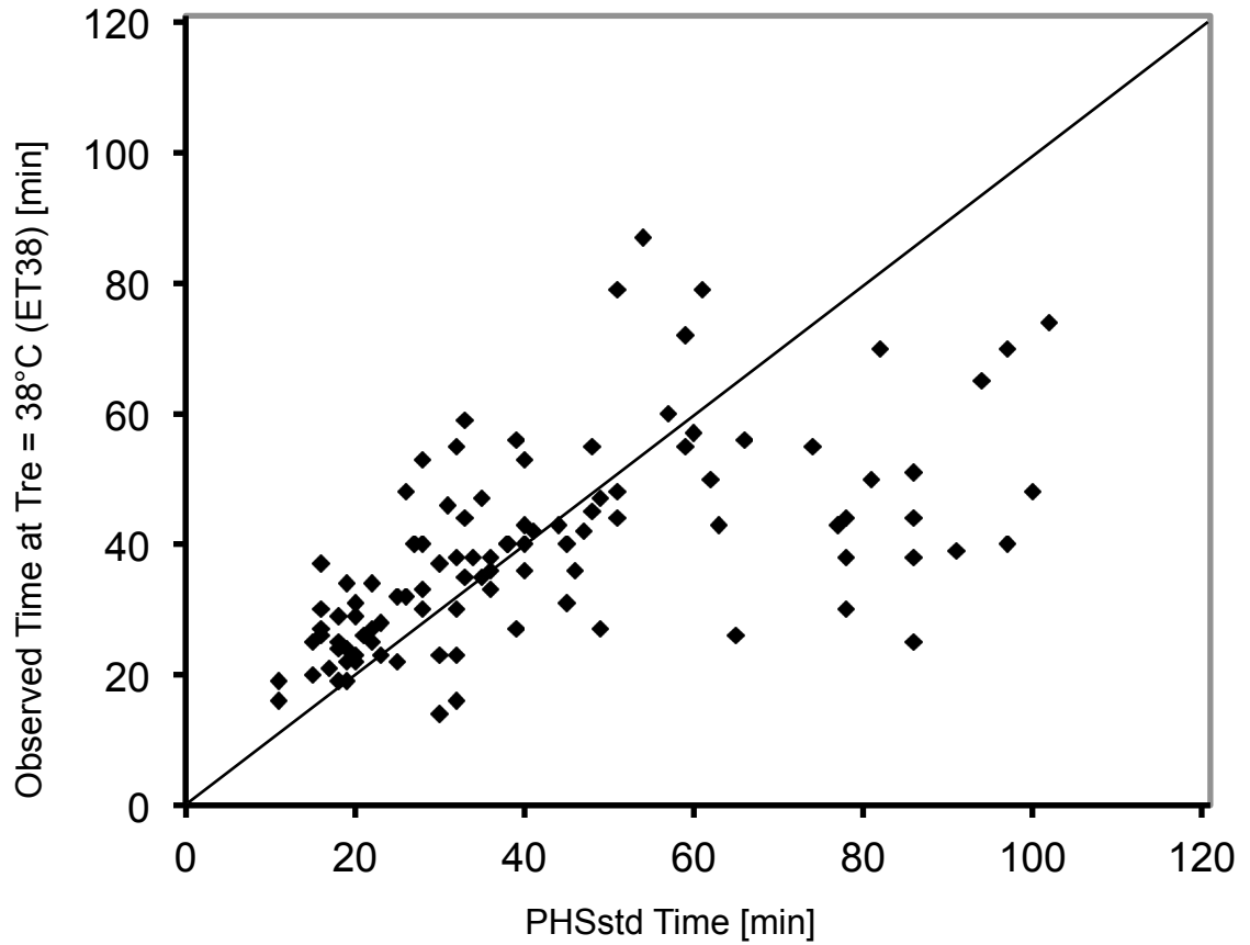
Figure 3. Relationship between PHS Standard Time Limit and the Observed Time at T_{re} = 38^{\circ}\text{C} (ET38).
