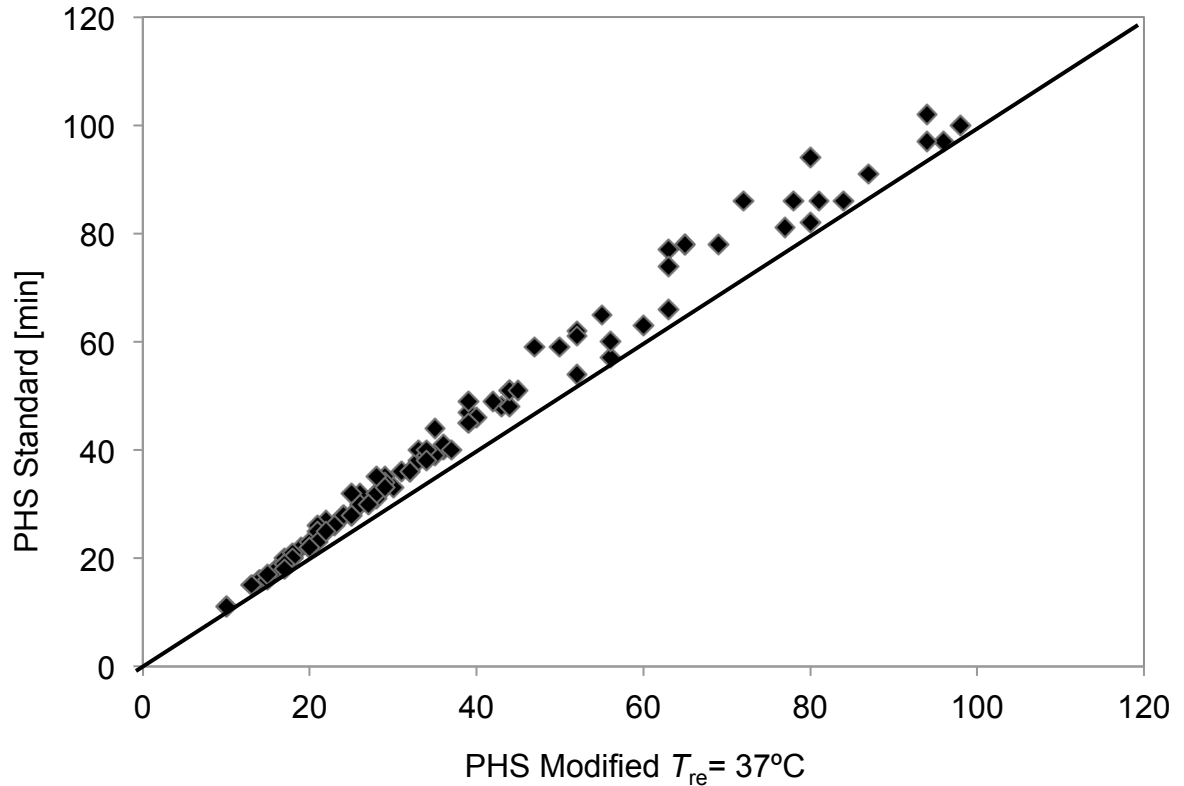
Figure 10. Comparison of PHS Standard (starting T_{re} = 36.8\text{ }^{\circ}\text{C} ) to the PHS Standard modified with a Starting T_{re} = 37\text{ }^{\circ}\text{C} .
