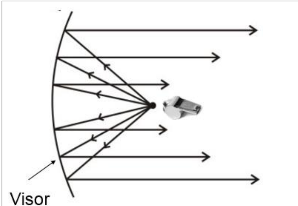
Figure 5.1: Whistle Noise Source Near a Reflective Concave Surface ( www.dronstudy.com )
