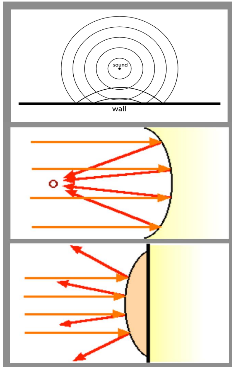
Figure 2.3: Sound pressure wave interactions (top to bottom): a. Sound pressure waves of a sound source near a planar reflective surface ( www.askaudio.com ) b. Sound pressure waves of a sound source near a concave surface c. Sound pressure waves of a sound source near a convex surface ( http://hyperphysics.phy-astr.gsu.edu/2016 )
