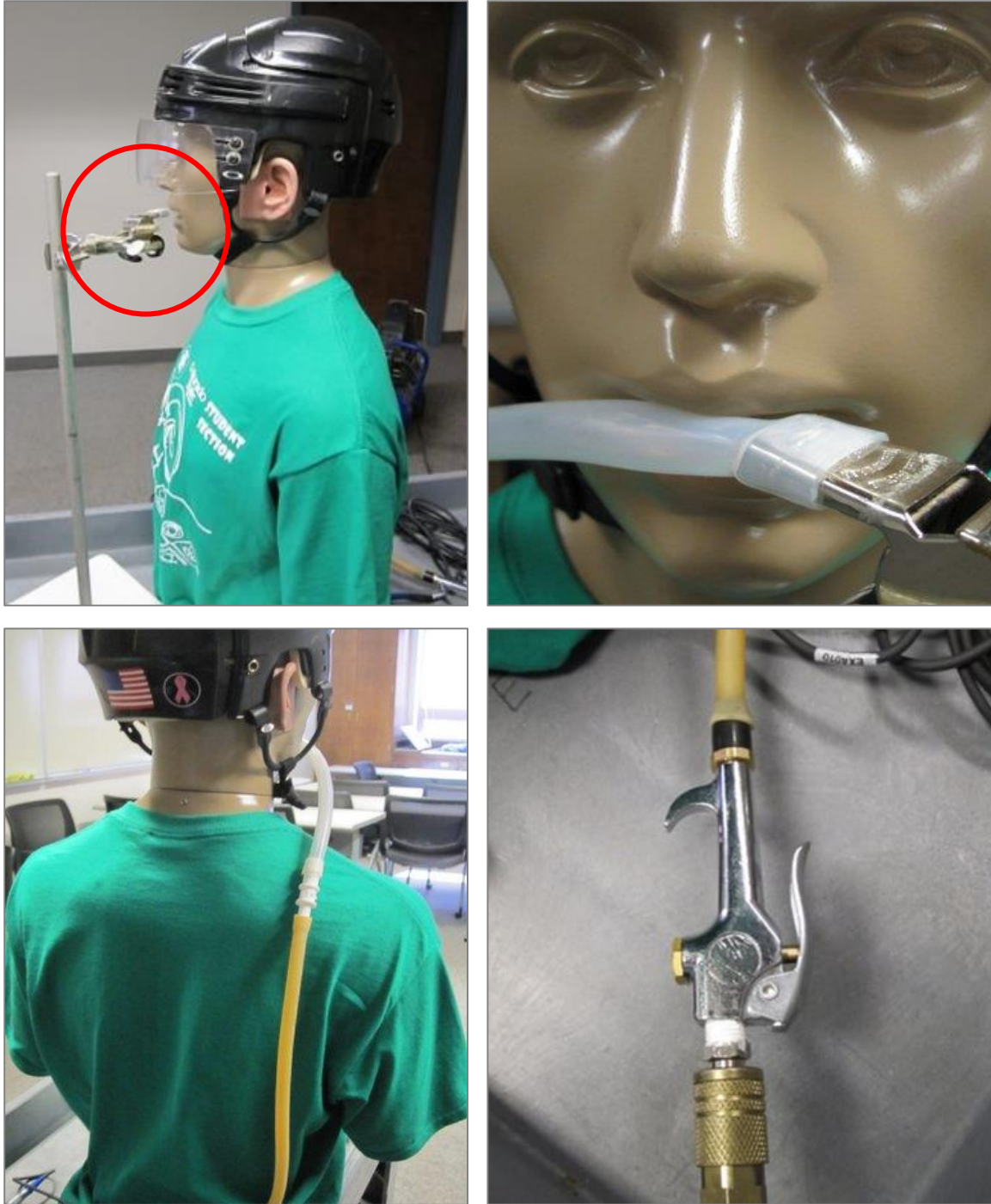
Figure 5.4: KEMAR whistle noise simulator (clockwise from upper left) a. Fox 40 ® Super Force ® finger grip pea whistle mounted on stand and placed near mouth of KEMAR Type 45 BA; b. silicon tubing connecting whistle near KEMAR Type 45 BA mouth to compressed air source; c. blow gun trigger assembly located on cart behind KEMAR Type 45 BA; d. silicon and rubber tubing connecting Fox 40 ® Super Force ® finger grip pea whistle to blow-gun
