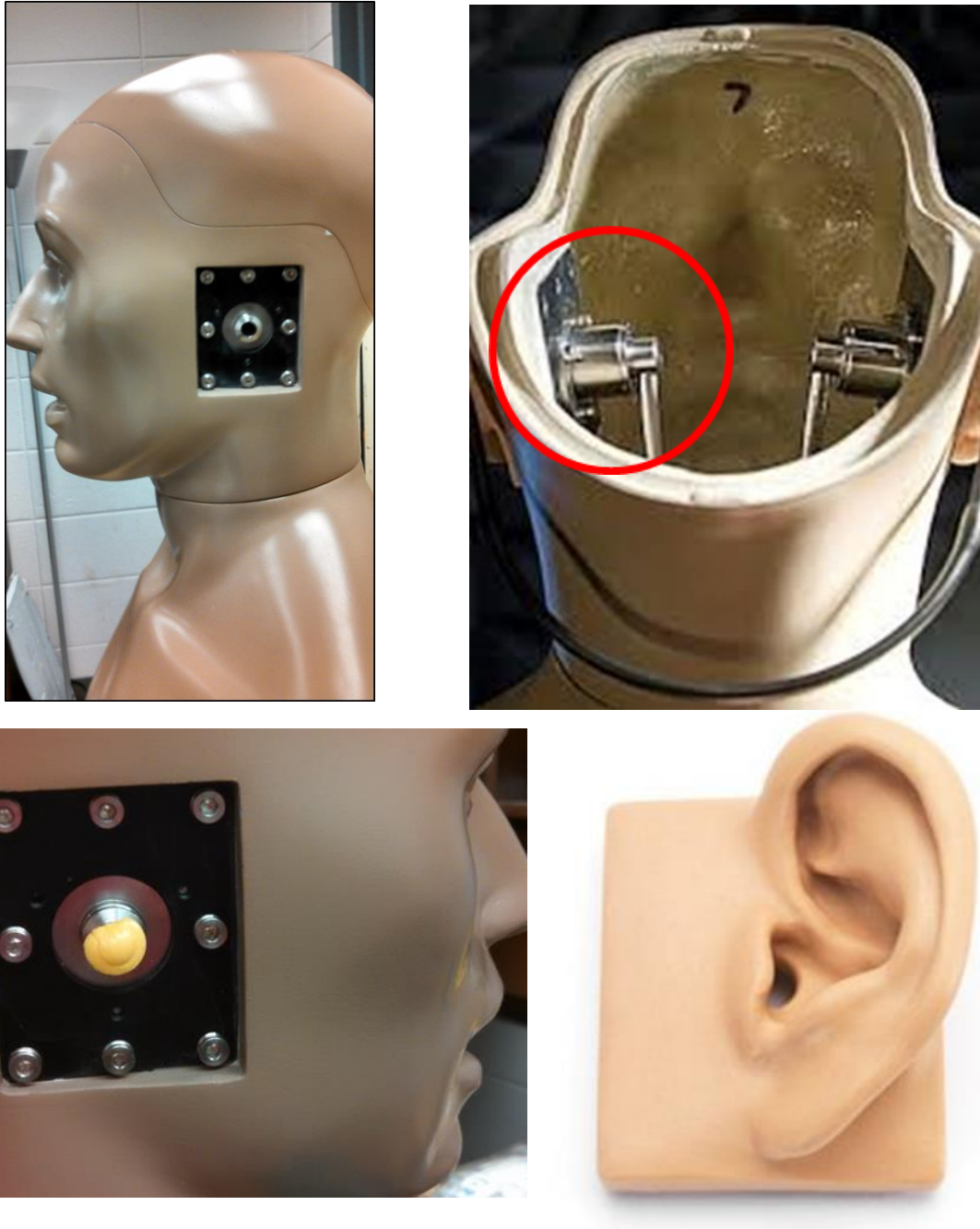
Figure 5.3: KEMAR manikin attributes (clockwise from top left) a. 43 AG left ear simulator for the KEMAR Type 45 BA; b. Type 26 AC preamplifier with an IEC 711 coupler for the KEMAR Type 45 BA; c. left ear pinna for the KEMAR Type 45 BA; d. right ear simulator of KEMAR Type 45 BA occluded with foam ear plug for duration of monitoring ( www.gras.com )
