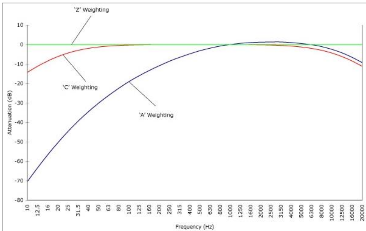
Figure 2.1: A, C and Z frequency weighting curves (NoiseNews®, 2016)
