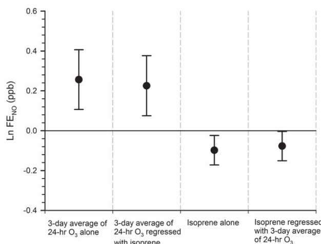
Figure 2. Per cent changes of natural log transformed FE NO in relation to concurrent isoprene and to the three-day average of 24 h average outdoor O 3 : single predictor and two-predictor models. All models are adjusted for splines of three-day average temperature.
