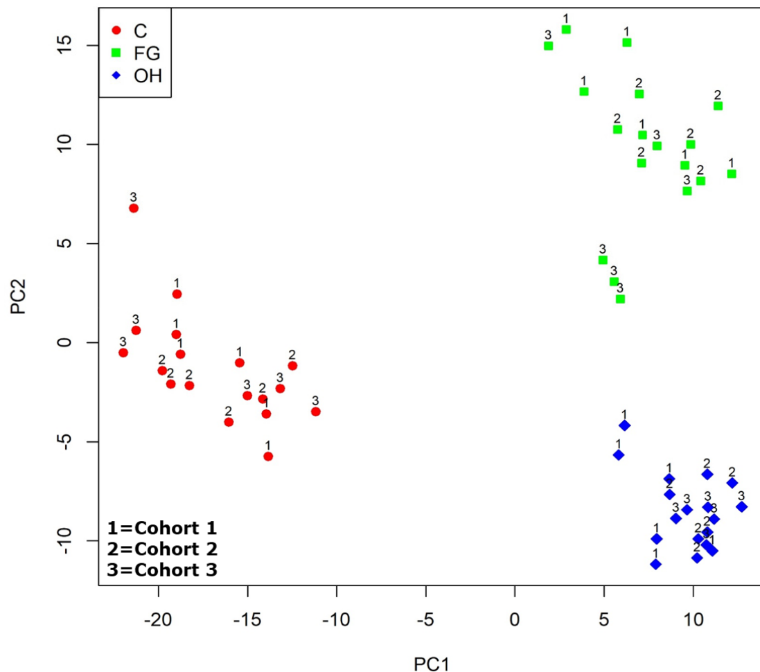
Fig 1. Principal component analysis of control, fireground, and overhaul gene expression data following surrogate variables removal. Principal components 1 and 2 are shown with control samples are represented by circles (red color). The fireground samples are represented by squares (lime color) and the overhaul samples represented as diamonds (blue color). The numeric labels 1, 2, and 3 indicate the cohort.
