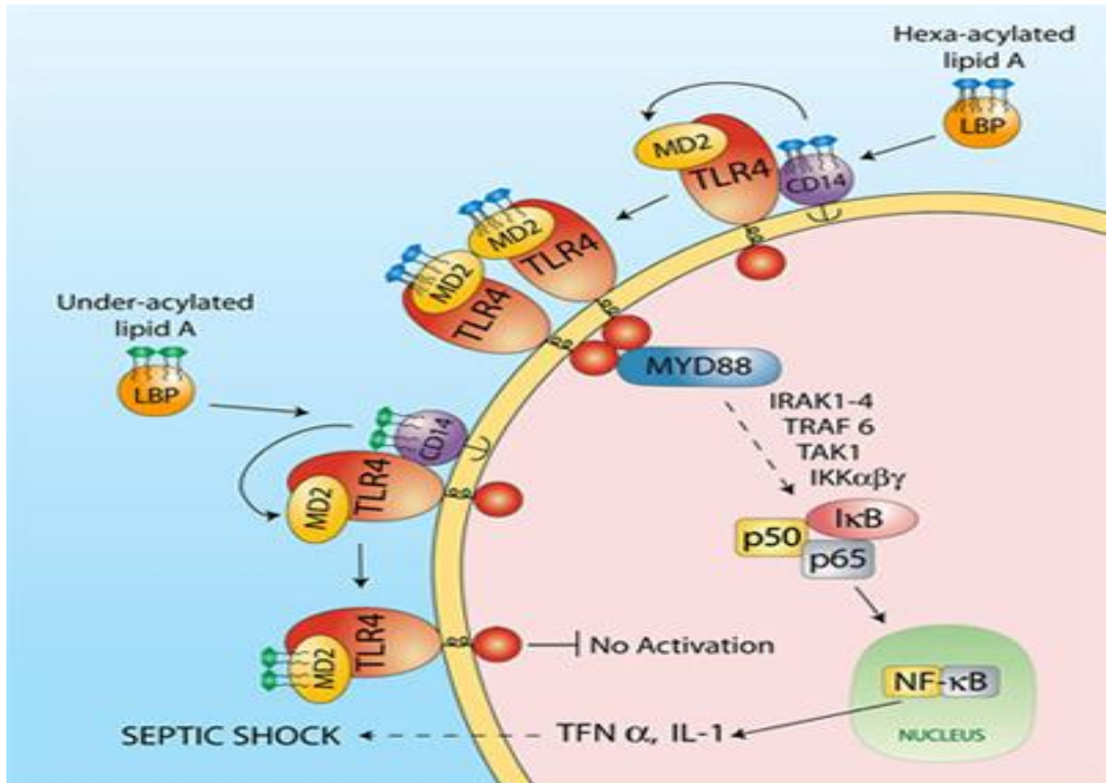
Figure 2.1 Immune response to LPS in human monocyte (58)
