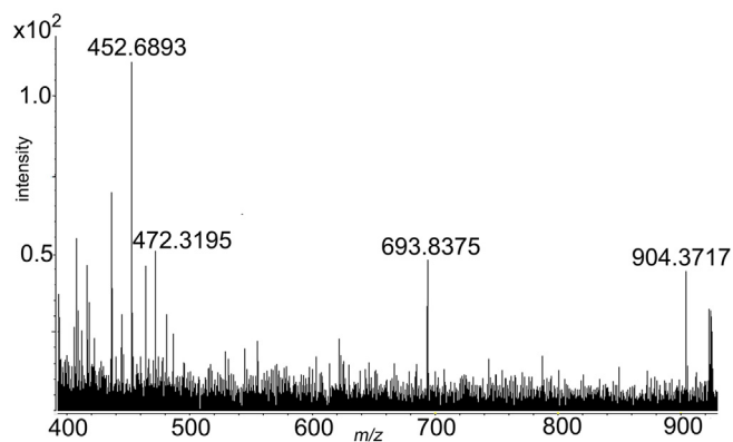
Fig. 4. LC-ESI-TOF mass spectrum of the chromatogram peak with a retention time of 15.11 min. Ions of m/z 904.3717 ( [M+H]^+ ) and m/z 452.6893 ( [M+2H]^{2+} ) correspond to the phosphorylated adduct of the peptide GSQQY 281 R from \beta -tubulin, and confirm the result from MALDI-TOF-MS analysis (see Fig. 2).
