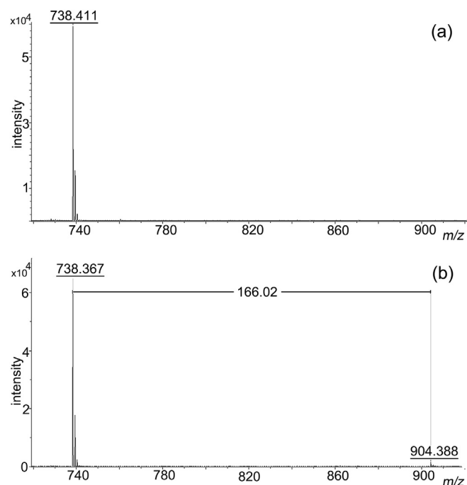
Fig. 2. MALDI-TOF/TOF MS/MS spectrum of the precursor adduct peptide ion at m/z 904.388. Fragmentation shows that profenofos covalently reacted with the Tyr 281 residue in the peptide GSQQY 281 R.
