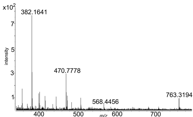
Fig. 5. LC-ESI-TOF mass spectrum of the chromatogram peak with a retention time of 14.16 min. Ions of m/z 763.3194 ( [M+H]^+ ) and m/z 382.1641 ( [M+2H]^{2+} ) corresponded to the profenofos adducted peptide TGT 83 R from \alpha -tubulin.
