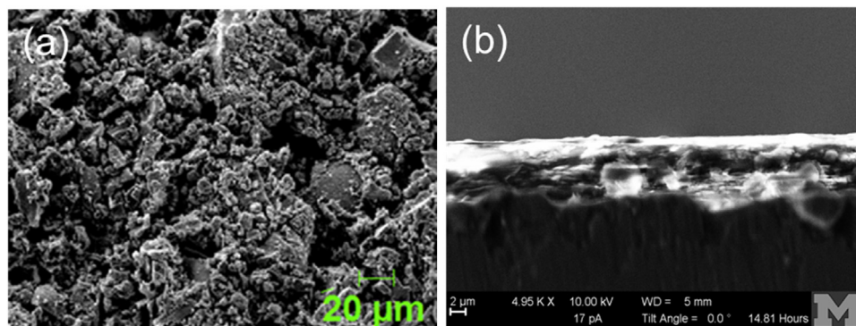
Fig. 2. SEM micrographs of TiNbON: (a) top view, and (b) side view.
