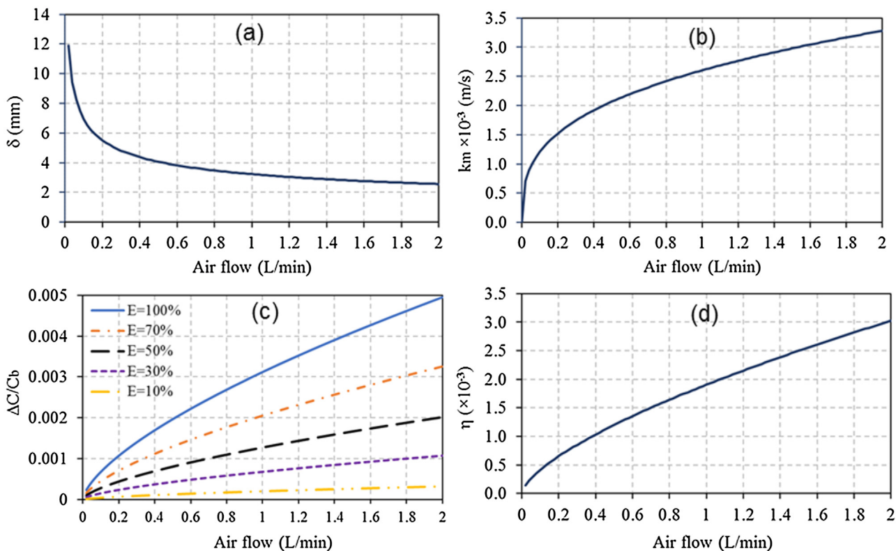
Fig. 5. Influence of air flow in convective mass transfer over PCO materials on: (a) concentration boundary layer thickness; (b) mass transfer coefficient; (c) concentration gradient; and (d) \eta .
