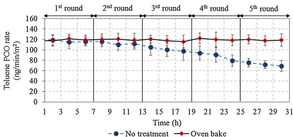
Fig. 8. Stability of TiNbON for toluene removal after 5 6-h test cycles (toluene 3.8 mg/m 3 , 25%RH, 0.2 L/min, LED 95 W/m 2 ).
