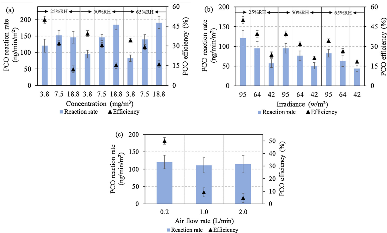
Fig. 4. Influence of operation conditions on the PCO of toluene: (a) Effect of concentration and humidity ( I = 95 \text{ W/m}^2 ); (b) Effect of irradiance and humidity ( C_{in} = 3.8 \text{ mg/m}^3 ); and (c) Effect of air flow ( C_{in} = 3.8 \text{ mg/m}^3 , I = 95 \text{ W/m}^2 ).
