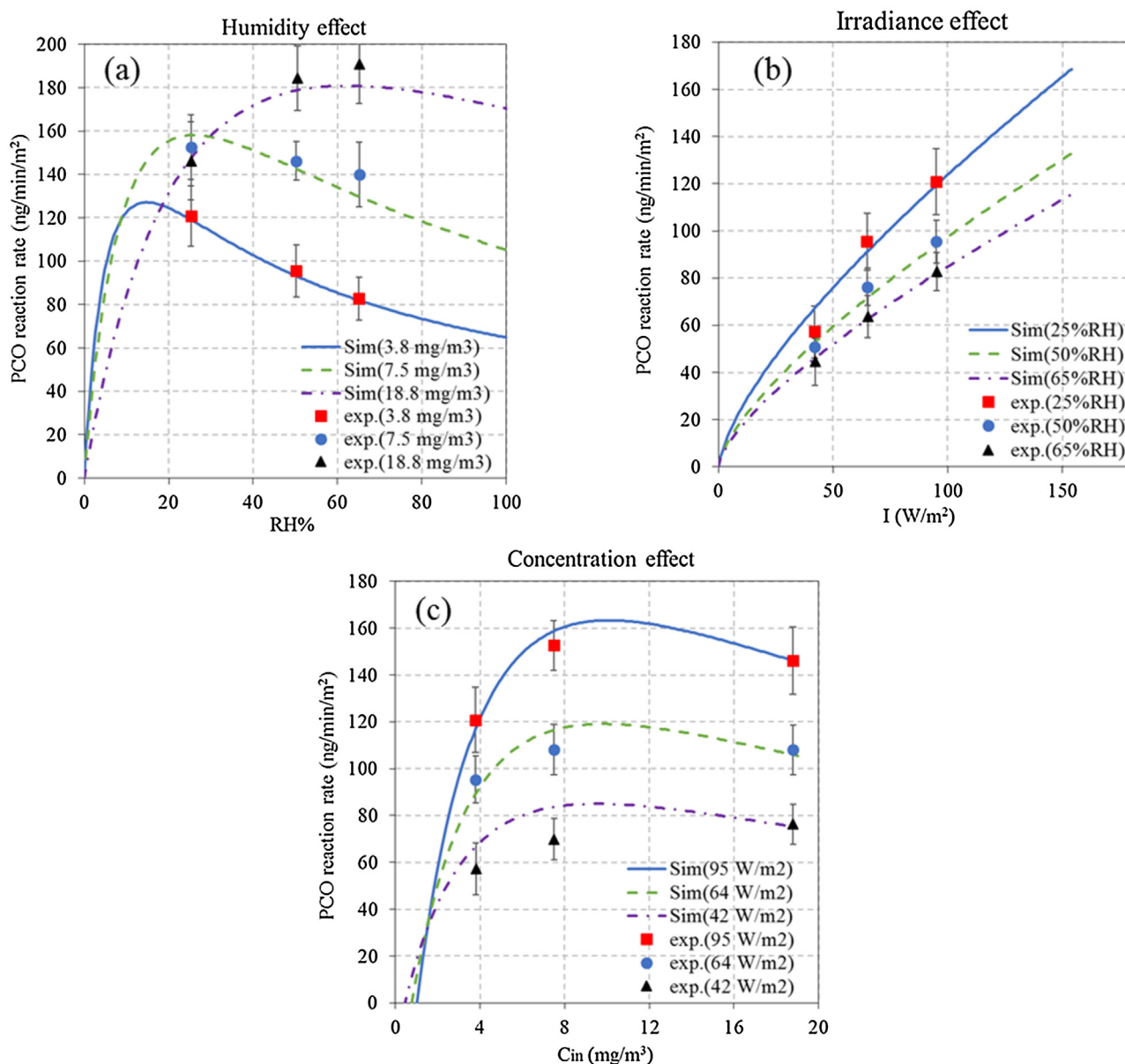
Fig. 6. Simulated and observed effects on the PCO reaction rates for toluene at steady-state: (a) influence of humidity with I = 95 \text{ W/m}^2 ; (b) influence of irradiance with C_{in} = 3.8 \text{ mg/m}^3 ; and (c) influence of inlet concentration with \text{RH} = 25\% .
