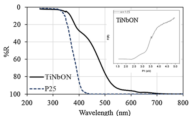
Fig. 3. Diffuse reflectance spectra of TiNbON and P25 catalysts.
