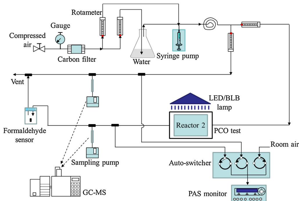
Fig. 1. Schematic diagram of the PCO system. Only 1 reactor is shown.
