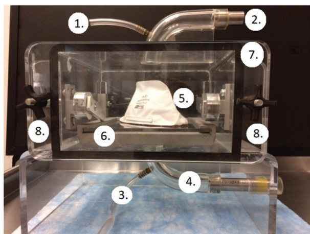
Figure 1. Filter penetration test set-up. A respirator sample was mounted on a Plexiglas plate and positioned inside the test set-up to measure filter penetration at 85 L/min flow rate. Keys: (1) Upstream sampling tube, (2) ambient air inlet tube, (3) downstream sampling tube, (4) vacuum line, (5) A respirator sealed to a Plexiglas plate, (6) Plexiglas plate holder, (7) front door, and (8) nut.
