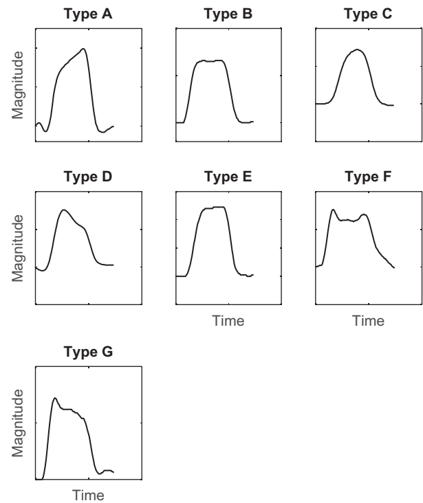
Figure 1. Prototypes used for correlation method of AR detection. Each plot represents time on the horizontal axis and reflex magnitude on the vertical axis. Note that a change in the upward direction represents a decrease in admittance. Prototypes were identified visually during review of AR traces, and the traces plotted in this figure were taken from raw traces.
