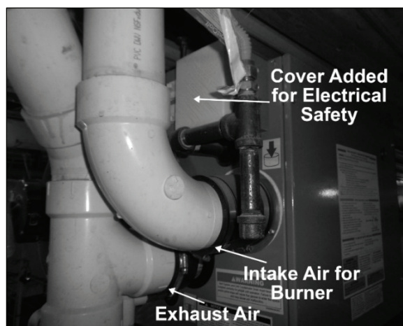
Figure 2. Back of installed vented heater, illustrating intake and exhaust ducts requiring installation.
