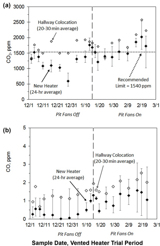
Figure 6. Average (a) CO 2 and (b) CO concentrations from the second winter (cyclone + vented heater testing), averaged over all monitors, including hallway colocation data. Error bars for 24 h data represent data ranges. Vertical dashed lines indicate the date when manure pit fans were activated.
