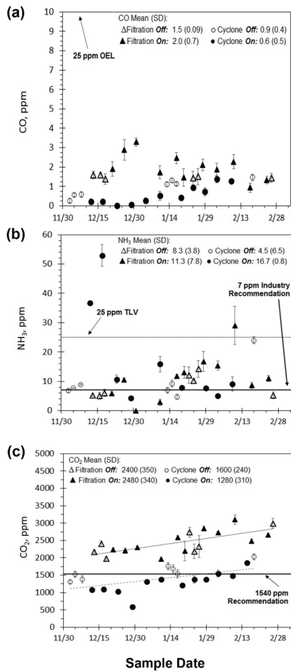
Figure 5. Room-averaged 24 h mean room concentrations of (a) CO, (b) NH 3 , and (c) CO 2 . Error bars indicate the minimum and maximum concentration measured on that day. Horizontal lines indicate recommended exposure limits. Dotted lines in (c) are best-fit regressions for CO 2 between the two test periods.
