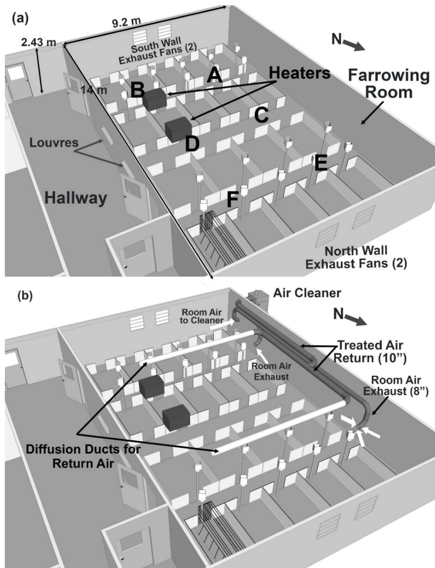
Figure 1. Farrowing room and adjoining hallway: (a) pre-intervention, with fixed area monitoring positions indicated as A-F, and (b) with recirculating ventilation system and air cleaner installed.
