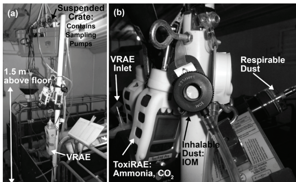
Figure 3. Samplers deployed for 24 h measurements with (a) crate with sampler pumps suspended from the ceiling and (b) sampler inlets and sensors positioned 1.5 m above the floor, as designated by eyebolts on fixed poles to ensure repeatable positioning throughout the study.
