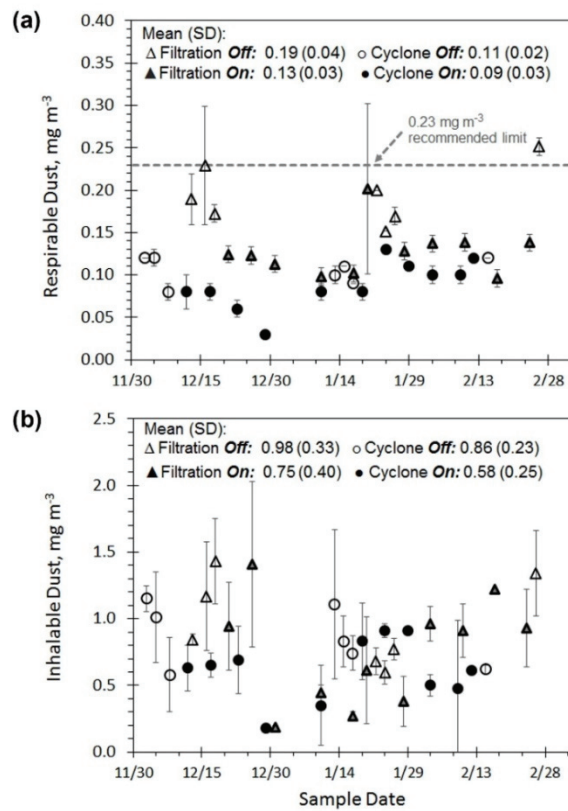
Figure 4. Room-averaged 24 h concentrations measured at locations A, C, and E for (a) respirable dust with recommended exposure limit of 0.23 \text{ mg m}^{-3} and (b) inhalable dust with recommended exposure limit of 2.8 \text{ mg m}^{-3} . Error bars indicate the range of concentrations measured in the room on that sample day.
