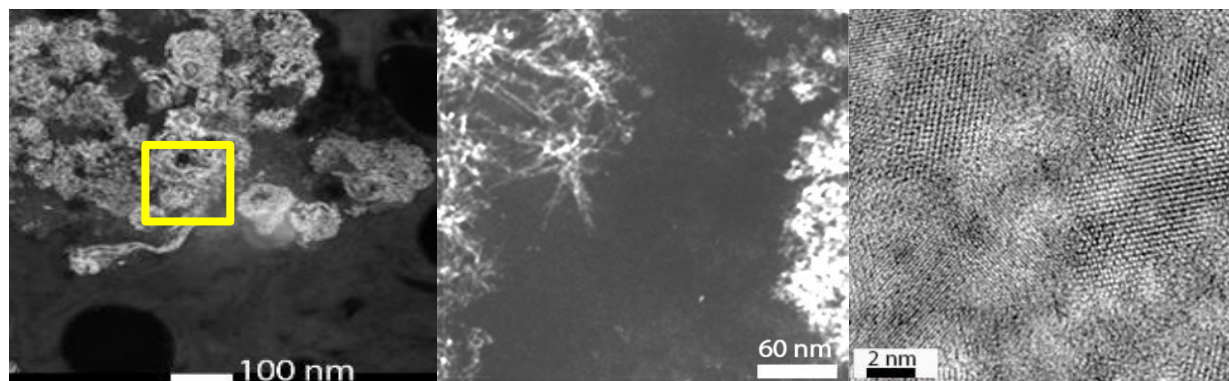
Figure 1. STEM images of (a) in vivo formed nanoparticle agglomerates in lung; (b) self-aligned nano needles from insert; (c) TEM image showing crystalline structures of nanoparticles.
