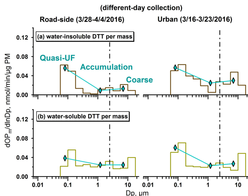
Figure 5. Water-insoluble (a) and -soluble (b) oxidative potential distributions on a per PM mass basis at a roadside site (RS, left panels, March 28–April 4, 2016) and a representative urban site (GT, right panels, March 16–23, 2016) in Atlanta, GA, USA. Average OP per mass for three modes, quasi-ultrafine ( <0.18 \mu\text{m} ), accumulation ( 0.18 \leq D_p \leq 3.2 \mu\text{m} ), and coarse ( 3.2 < D_p < 10 \mu\text{m} ) is also shown (diamonds with line). PM mass on each MOUDI stage was estimated from the sum of measured chemical components. The dotted line is aerodynamic diameter D_p = 2.5 \mu\text{m} .
