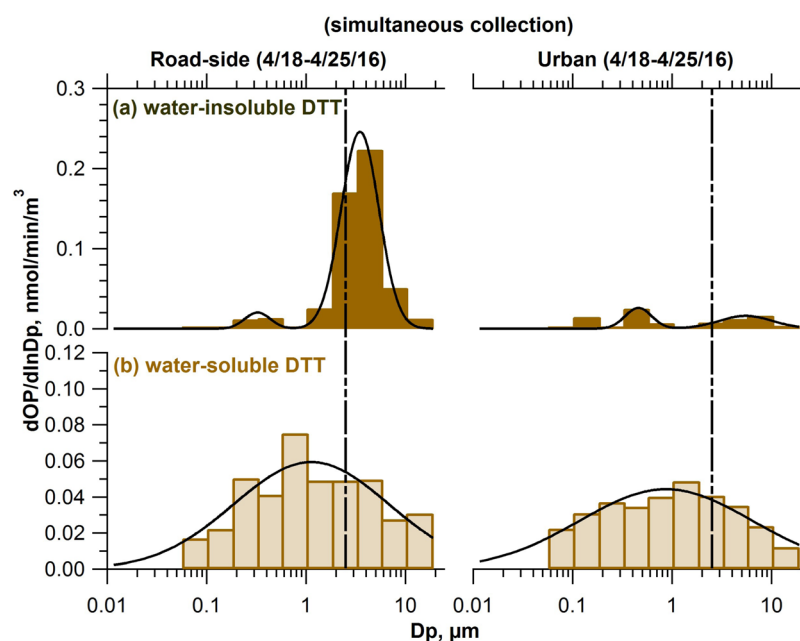
Figure 3. Ambient size distribution of water-insoluble (a) and -soluble (b) oxidative potential from MOUDI samples collected simultaneously at a roadside site (RS, left panels) and a representative urban site (GT, right panels) in Atlanta, GA, USA. The vertical dotted line is aerodynamic diameter D_p = 2.5 \mu\text{m} .
