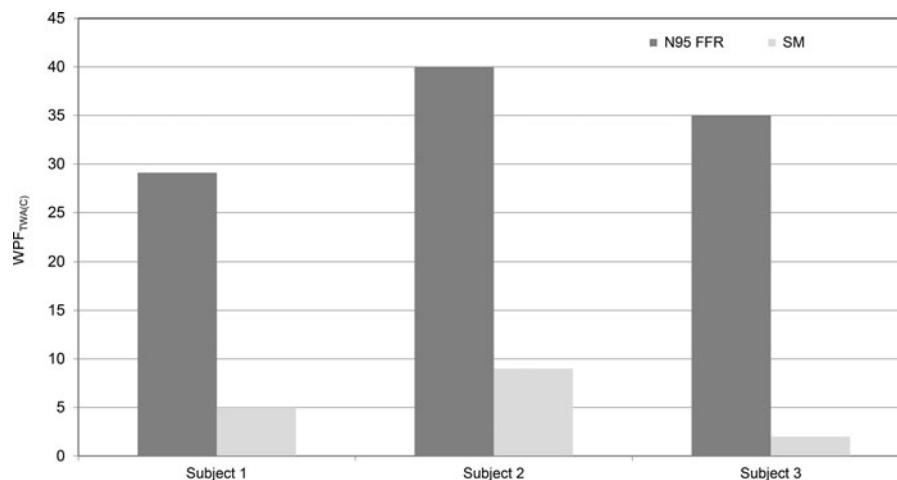
Figure 2. The WPF_{TWA(C)} values time-weighted averaged over the entire test time for three RPD-wearing subjects. Each bar represents a single day measurement.
