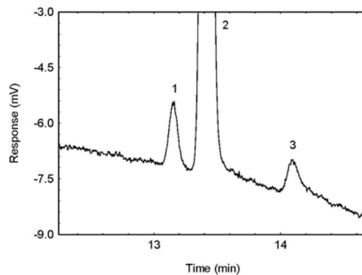
Figure 4.2.2. A chromatogram of the RQL of 2,3-pentanedione. (Key: 1) 2,3-pentanedione; 2) 3-pentanedione; and 3) interferant.)
