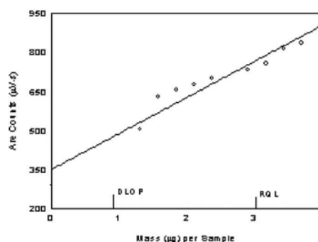
Figure 1.2.1 Plot of data to determine the DLOP/RQL for diacetyl. ( Y=139X+349 )
