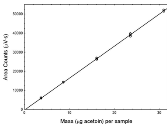
Figure 3.5.2.1. Calibration curve of acetoin. ( Y = 1678X - 389 )
