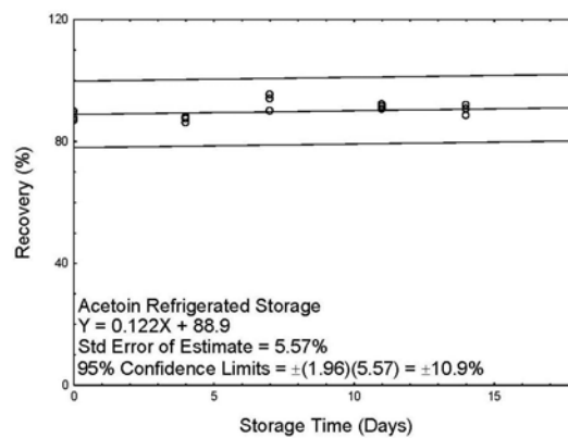
Figure 4.5.2. Refrigerated storage test for acetoin.
