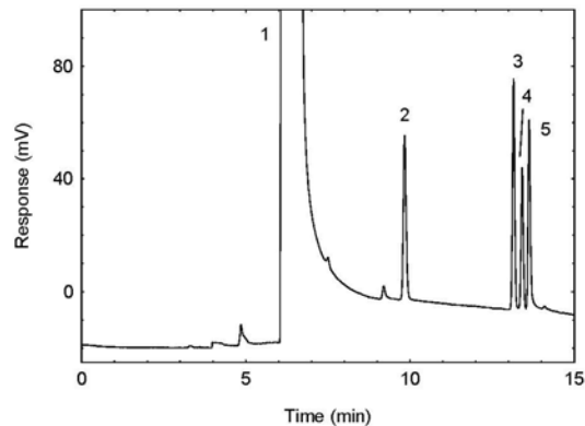
Figure 3.5.1.2. A chromatogram of 20.4 µg/sample 2,3-pentanedione, 15.8 µg/sample acetoin, and 15.6 µg/sample diacetyl. (Key: 1) ethyl alcohol; 2) diacetyl; 3) 2,3-pentanedione; 4) 3-pentanone; and 5) acetoin.)
