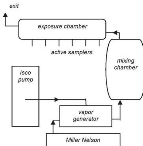
Figure 4.11. The test atmosphere generation and sampling apparatus.
