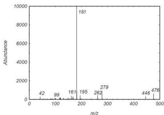
Figure 4.10.2. Mass spectrum of diacetyl-PFBHA derivative.
