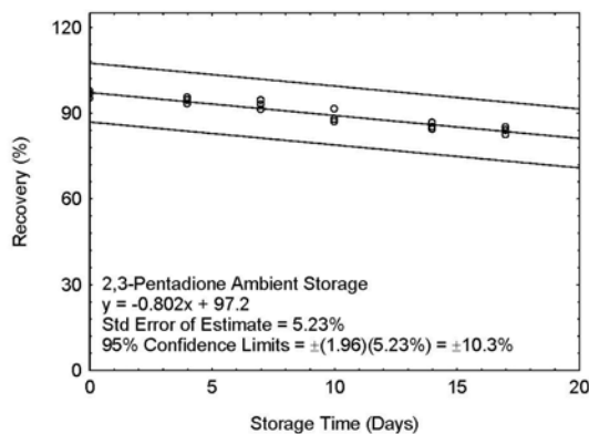
Figure 4.4.1. Ambient storage test for 2,3-pentanedione.
