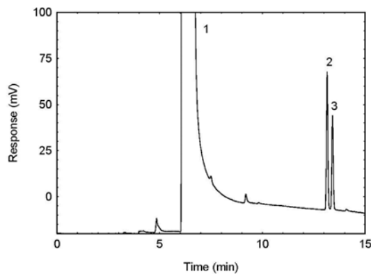
Figure 3.5.1.1. A chromatogram of 20.4 µg/sample 2,3-pentanedione. (Key: 1) ethyl alcohol; 2) 2,3-pentanedione; and 3) 3-pentanone.)
