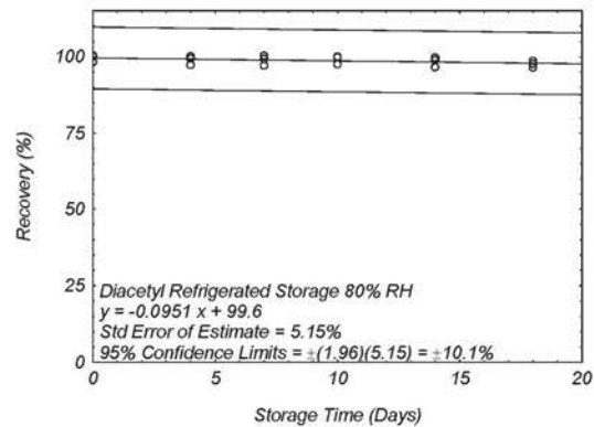
Figure 4.5.4. Refrigerated storage test for diacetyl at 80% RH.
