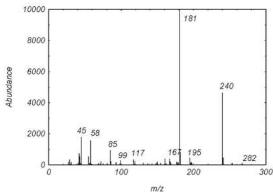
Figure 4.10.1. Mass spectrum of acetoin-PFBHA derivative.
