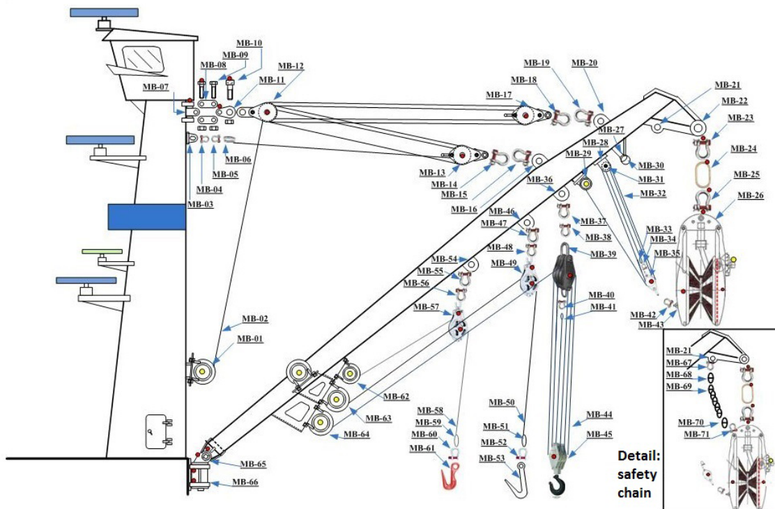
Figure 4 - Schematic of the Maintenance/Inspection Points of the Riggings for one Vessel's Mast and Main Boom
