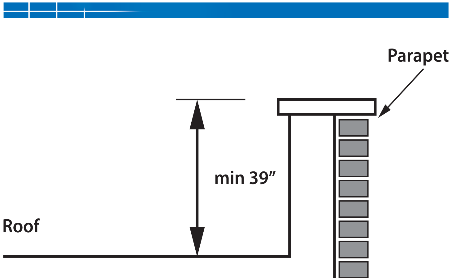
Figure 1. Design of a building using a parapet. (Diagram by Nicholas Tymvios and John Gambatese, Oregon State University)
