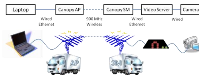
Figure 1. Network configured to transmit video from a remote site subscriber module (SM) to the command center access point (AP).
