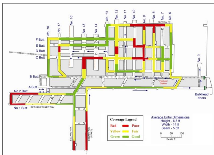
Figure 3. Mine communications coverage map with data generated from the MCM.
