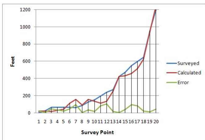
Figure 2. Comparison of surveyed distance from starting point and the tracking system's calculated distance for tags at every other crosscut.
