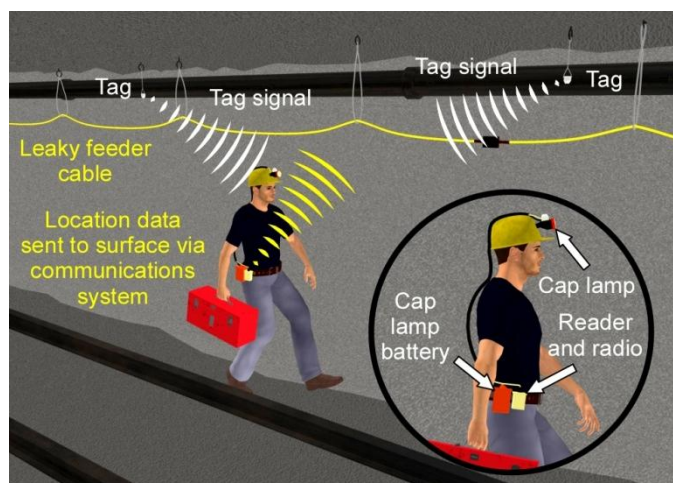
Figure 1. The reverse RFID concept with tags mounted on the mine roof and portable, belt-worn readers.
