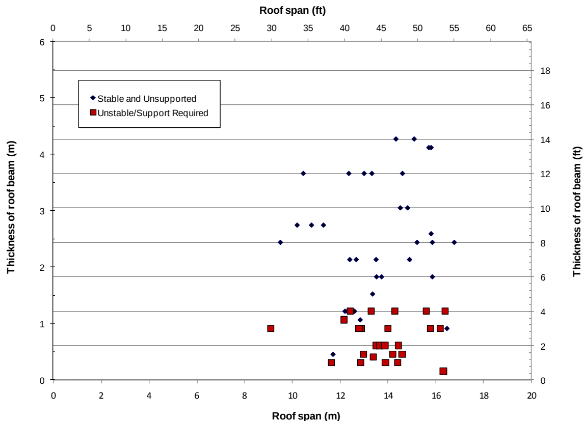
Figure 30. Chart showing the effect of the thickness of the roof beam on excavation stability in mines that did not experience horizontal stress related instability.
