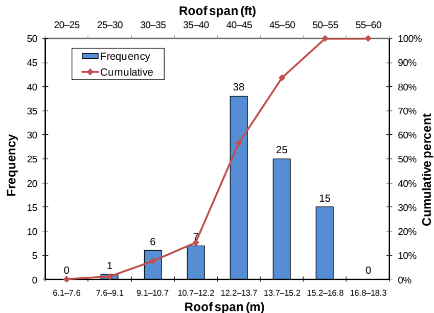
Figure 26. Distribution of roof span dimensions measured at 34 different underground stone mines.
