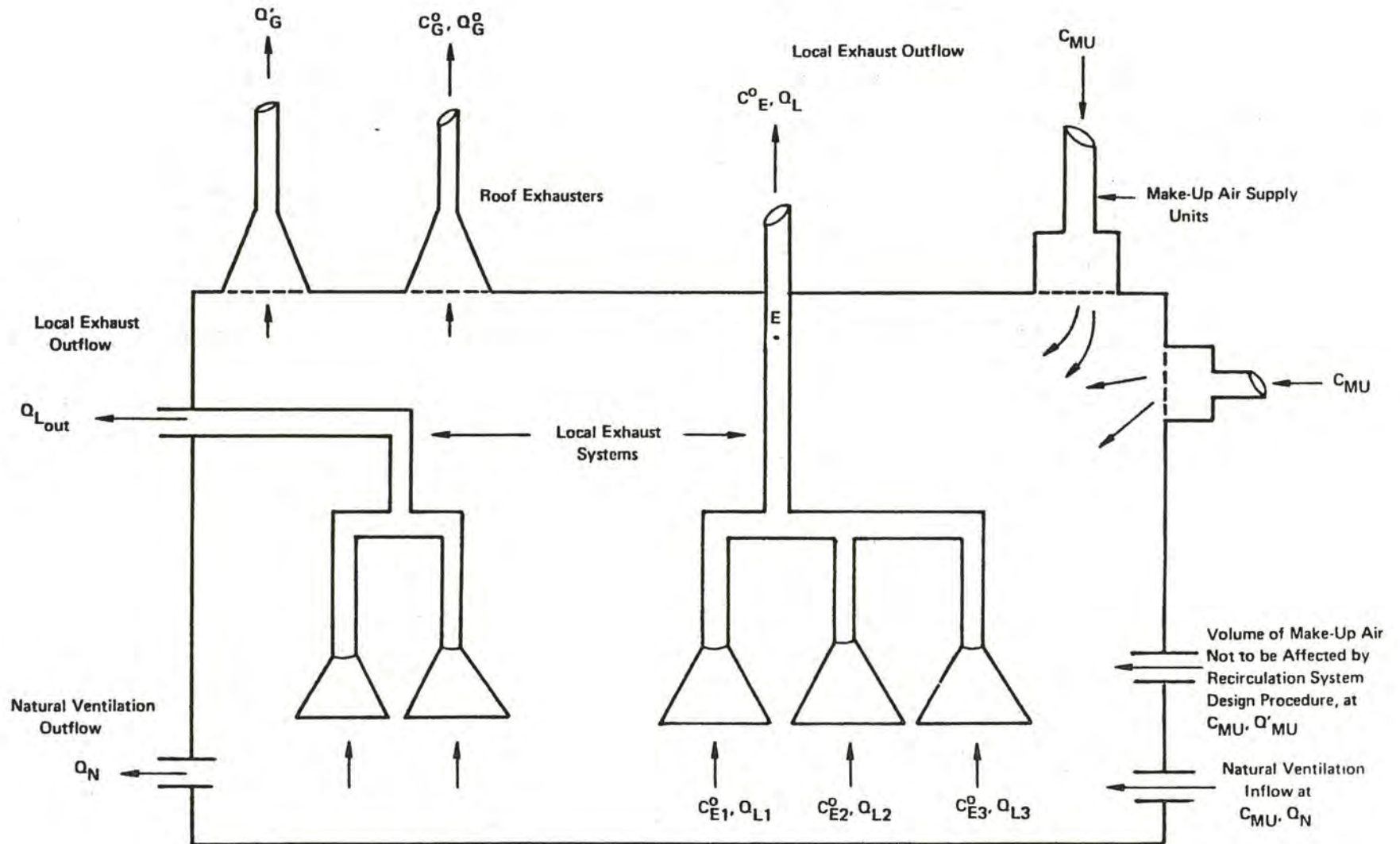
Figure 2. Plant area before recirculation.
