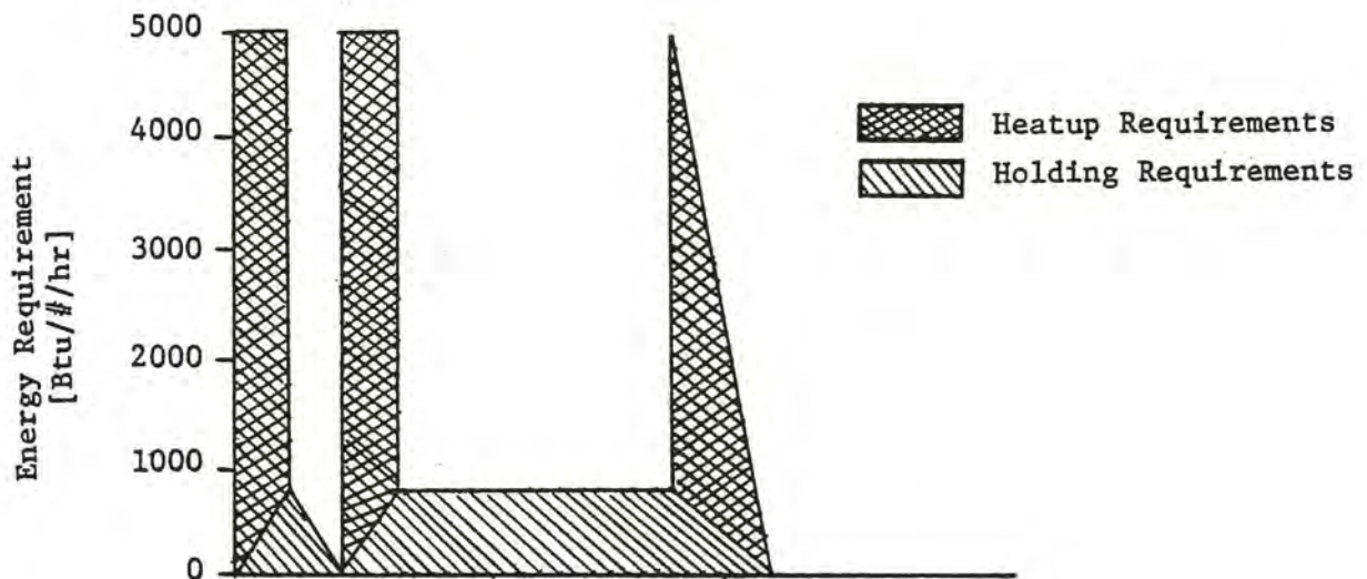
Figure 7. Energy requirements for typical open Beck cycle.
