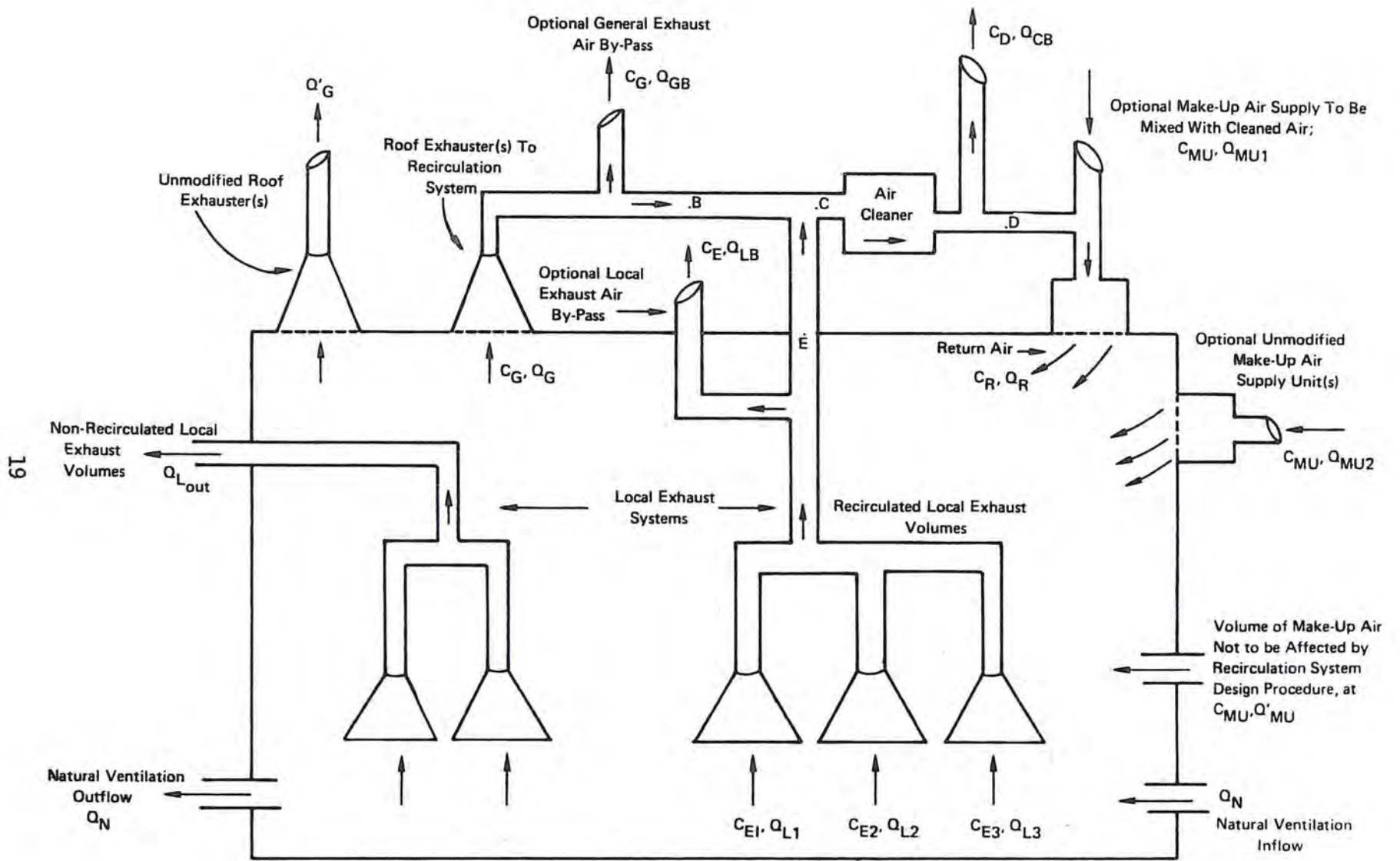
Figure 3. Plant area with recirculation--Model #1.
