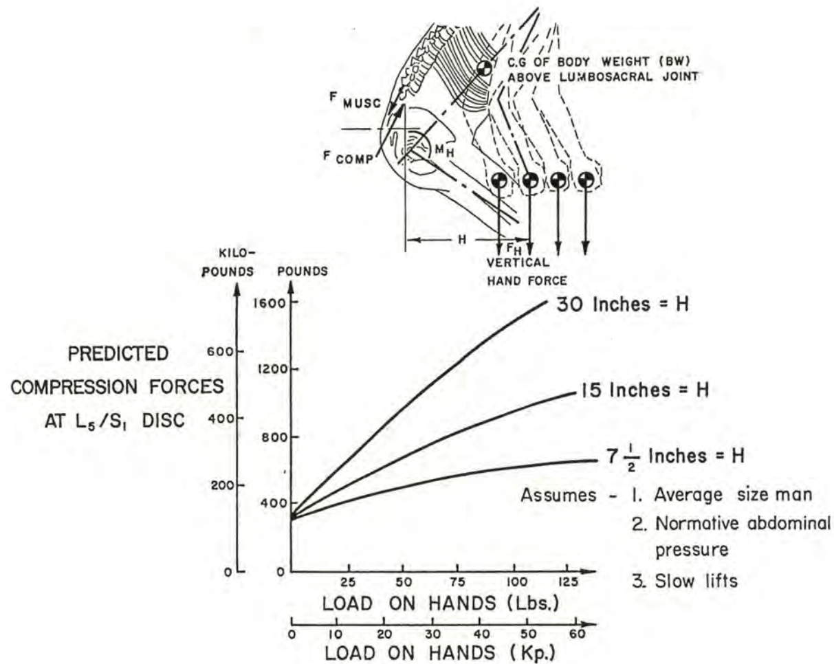
Figure 5: Predicted compression forces acting on L 5 /S 1 disk when lifting loads of various magnitudes
