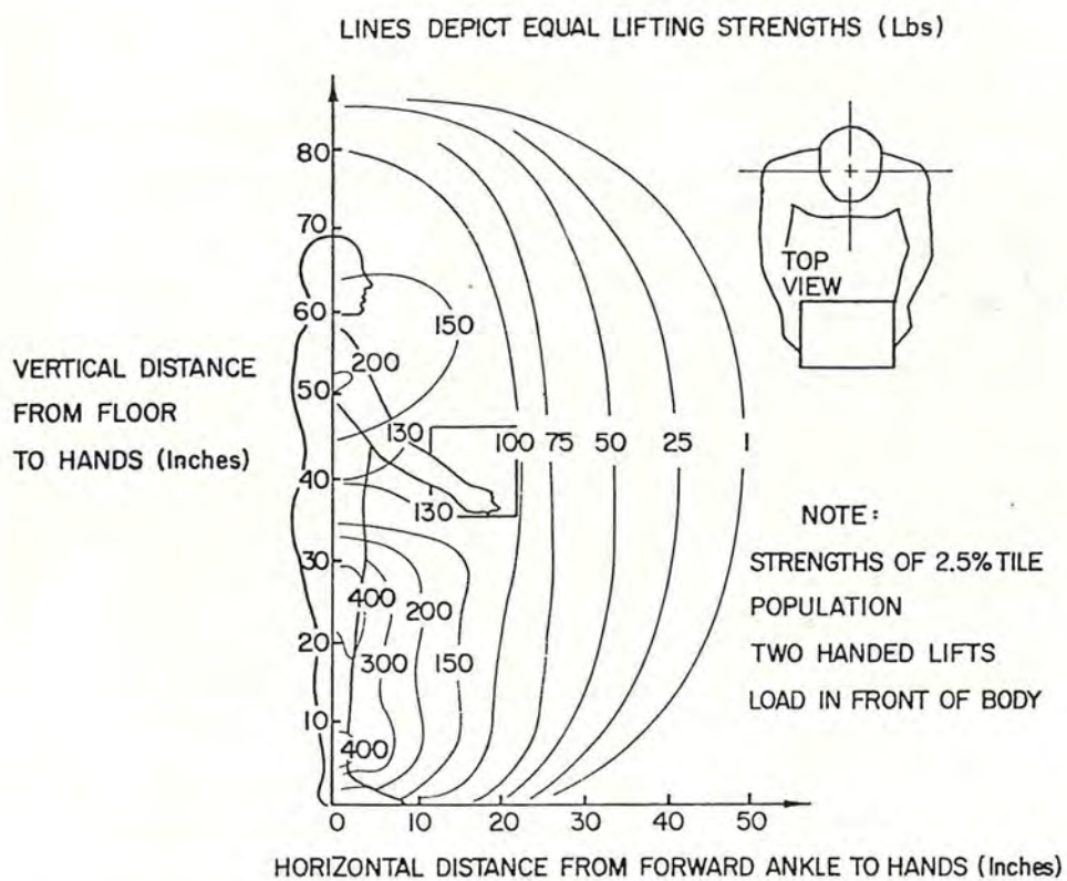
Figure 10: Predicted lifting strengths for all but 2.5% of workmen
