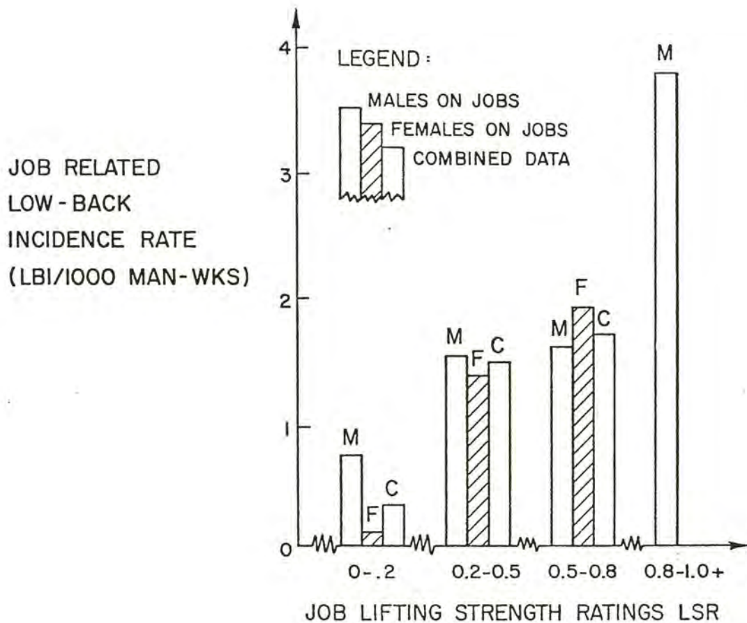
Figure 11: Mean low-back incidence rates for jobs having varying lifting strength requirements
