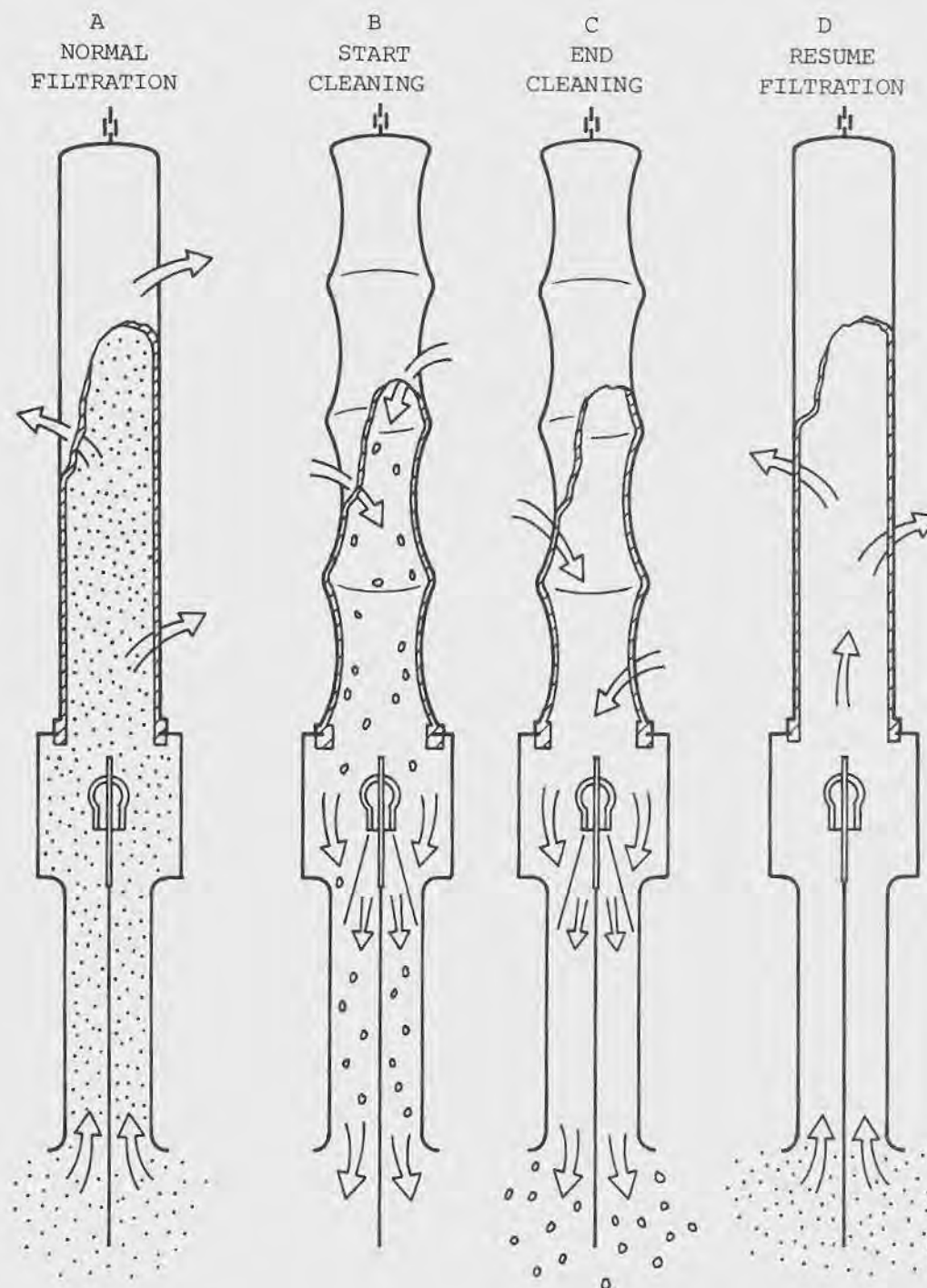
Figure 19. Electrostatically Augmented Fabric Filter operating and cleaning sequence.
