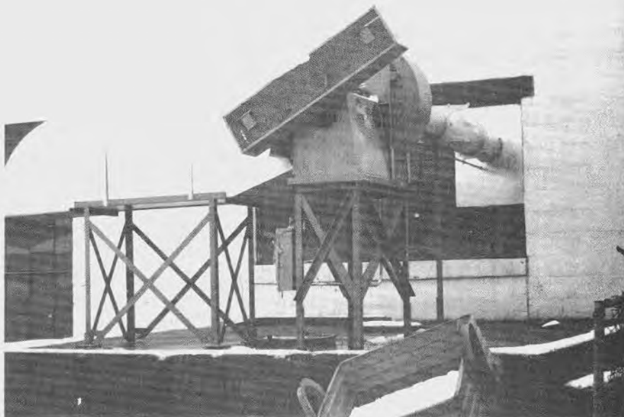
Figure 7. Blower and sound trap.
