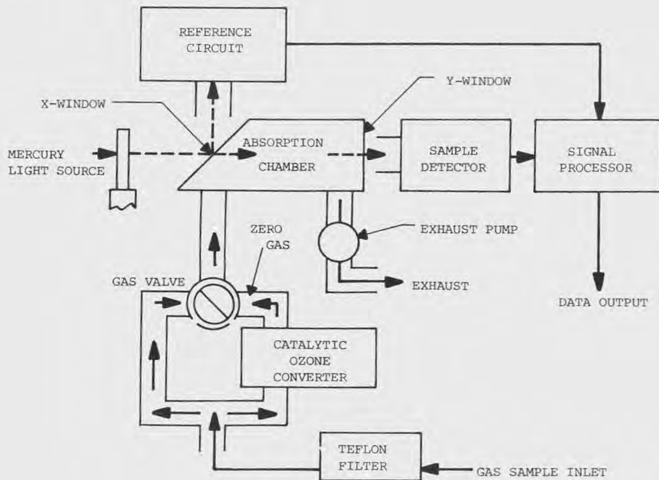
Figure 51. Ultraviolet Ozone Monitor schematic diagram (from manufacturer's instruction manual).
