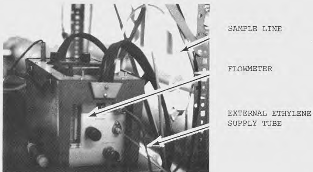
END VIEW
