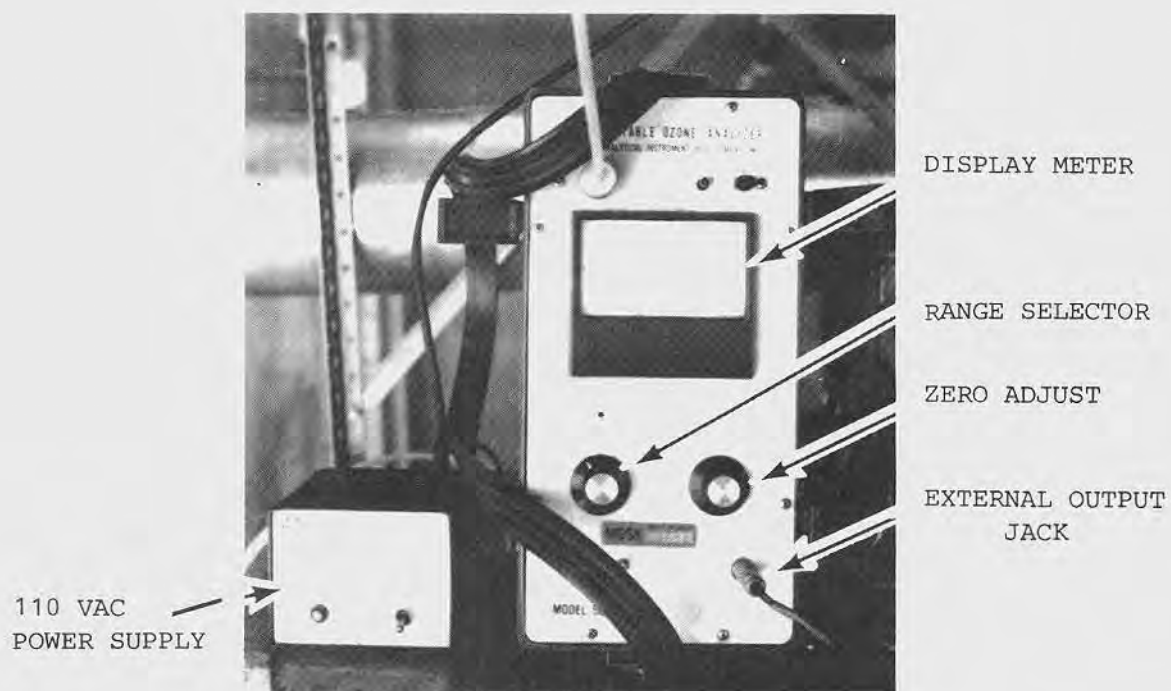
FRONT VIEW
