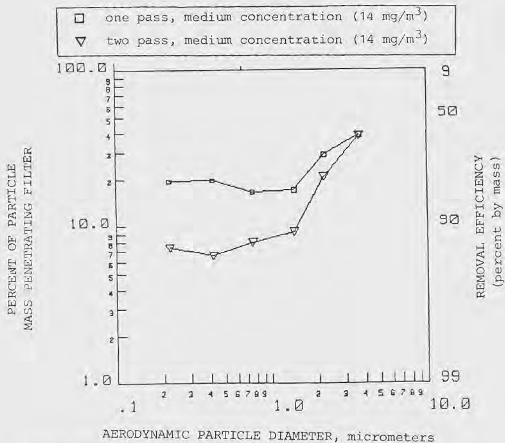
Figure 14. Electrostatic Precipitator fractional penetration.
