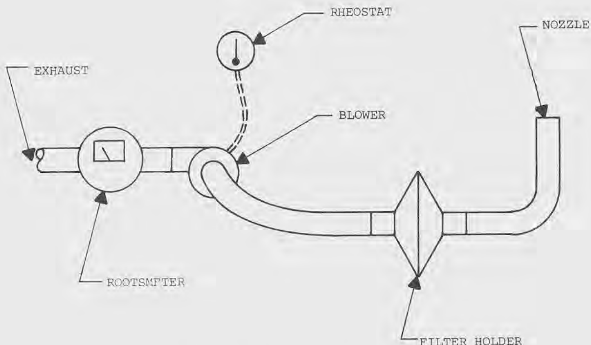
Figure 9. High volume sampling train.
