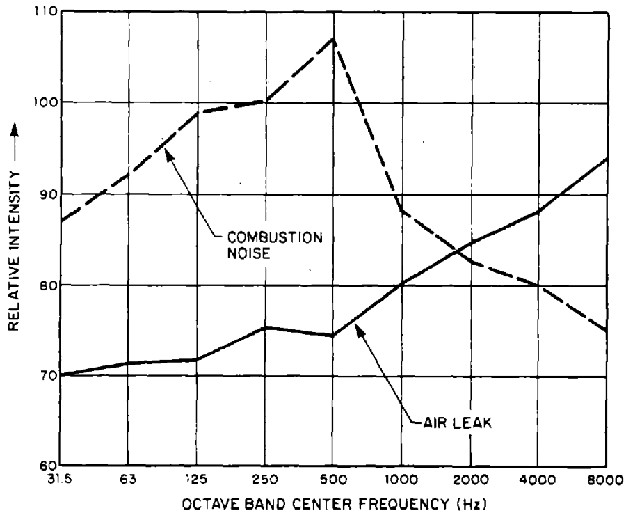
Figure 2.3. Frequency composition of two common industrial sounds.
