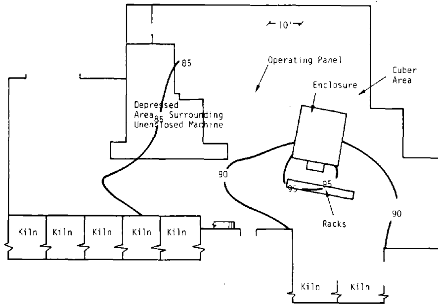
Figure 6.35.4. Plant 2: maximum sound level contours.
