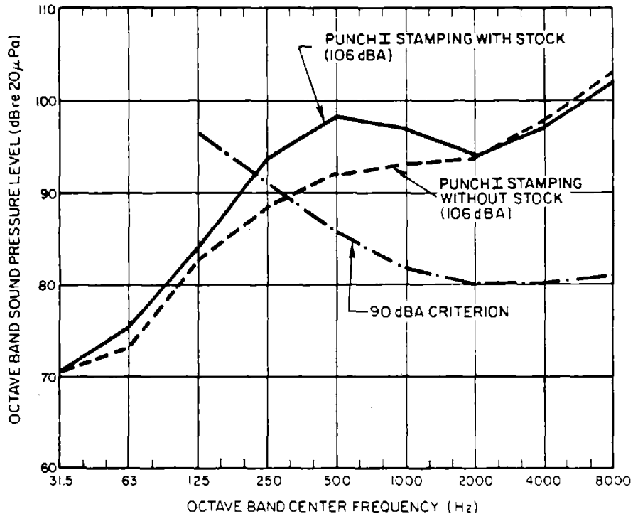
Figure 6.53.3. Sound pressure levels at Punch I.
