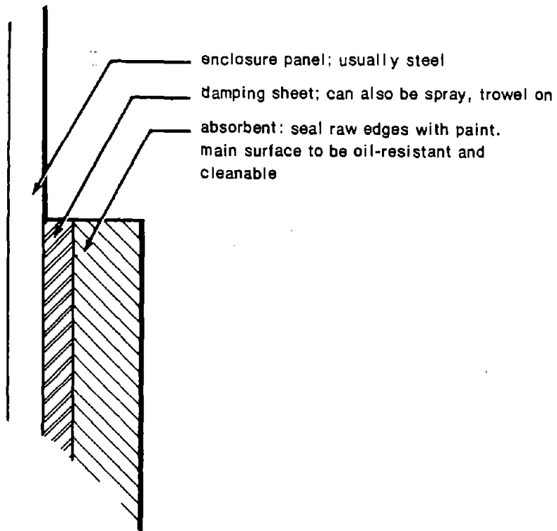
Figure 3.7. Enclosure panel interior treatment.
