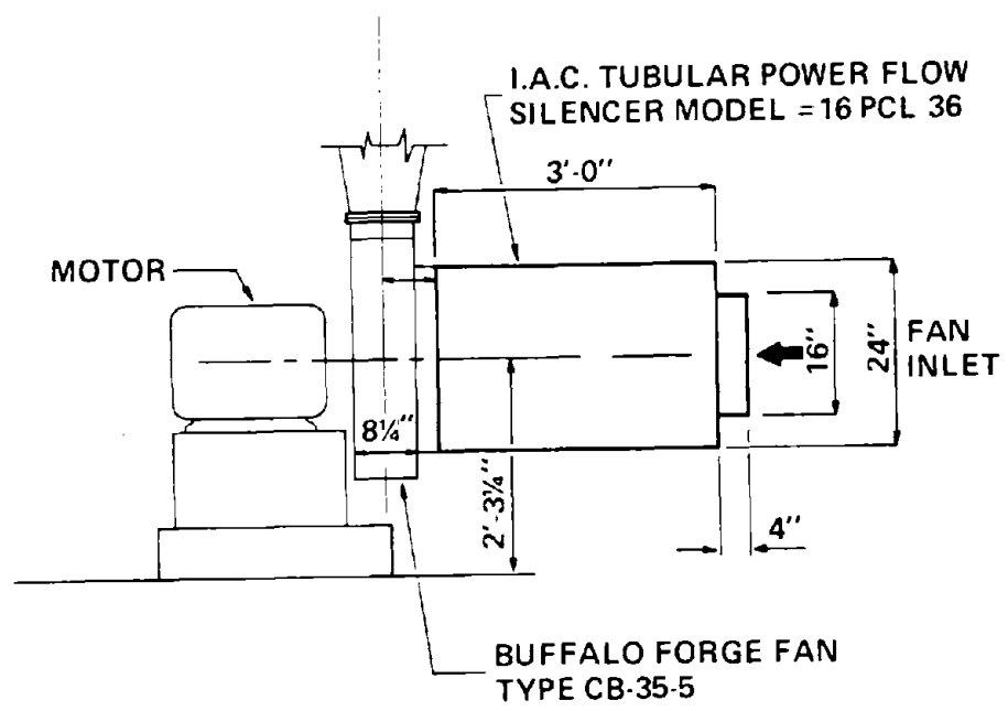
Figure 6.42.1. Elevation drawings showing how two fans at an R.J. Reynolds Tobacco Co. plant in Winston-Salem, North Carolina were quieted by IAC tubular and rectangular Power-FLOW silencing units.
