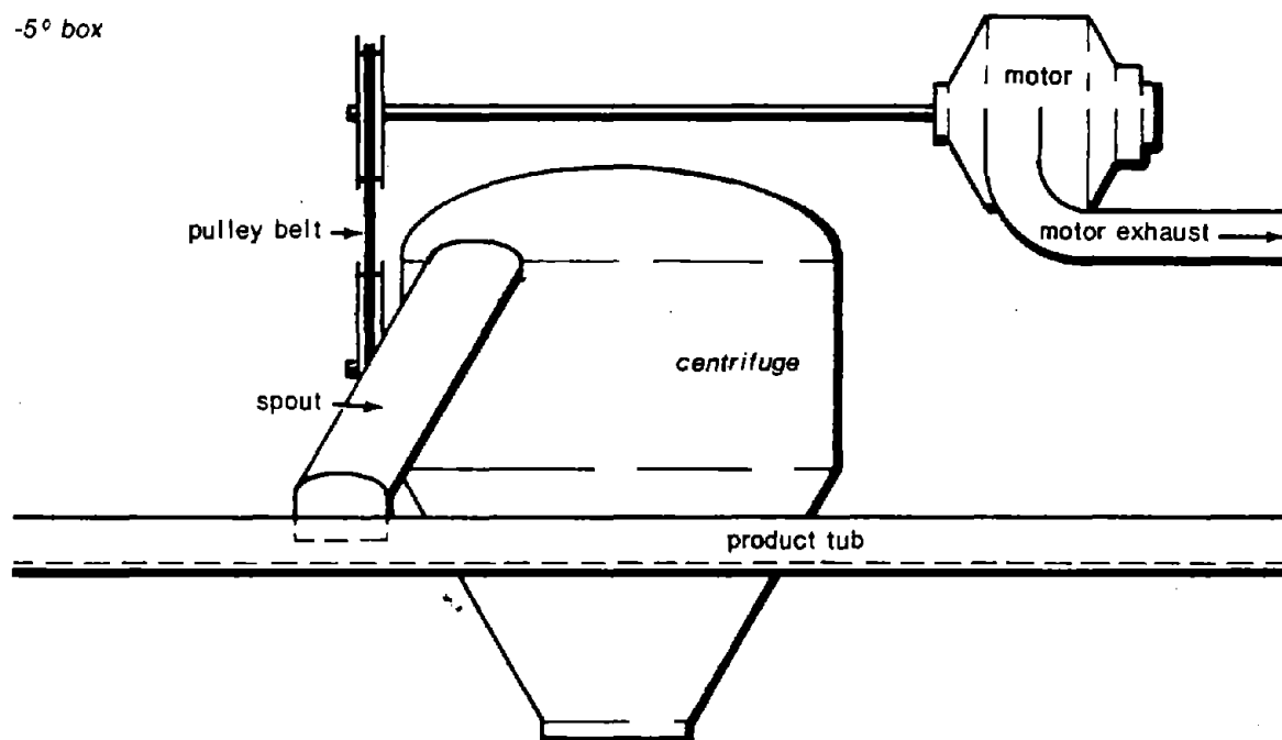
Figure 6.38.1. Sketch of one centrifuge (front view).
