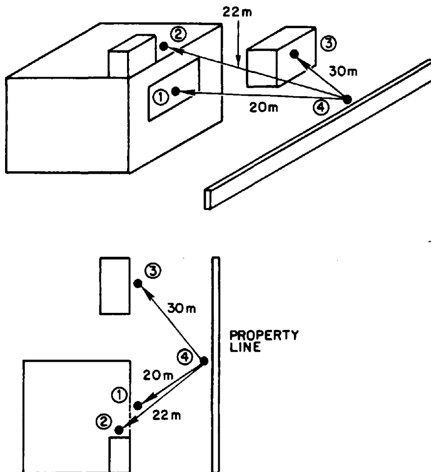
Figure 2.10. Location of noise sources (1-3) relative to property level position (4) for use in example on these pages.
