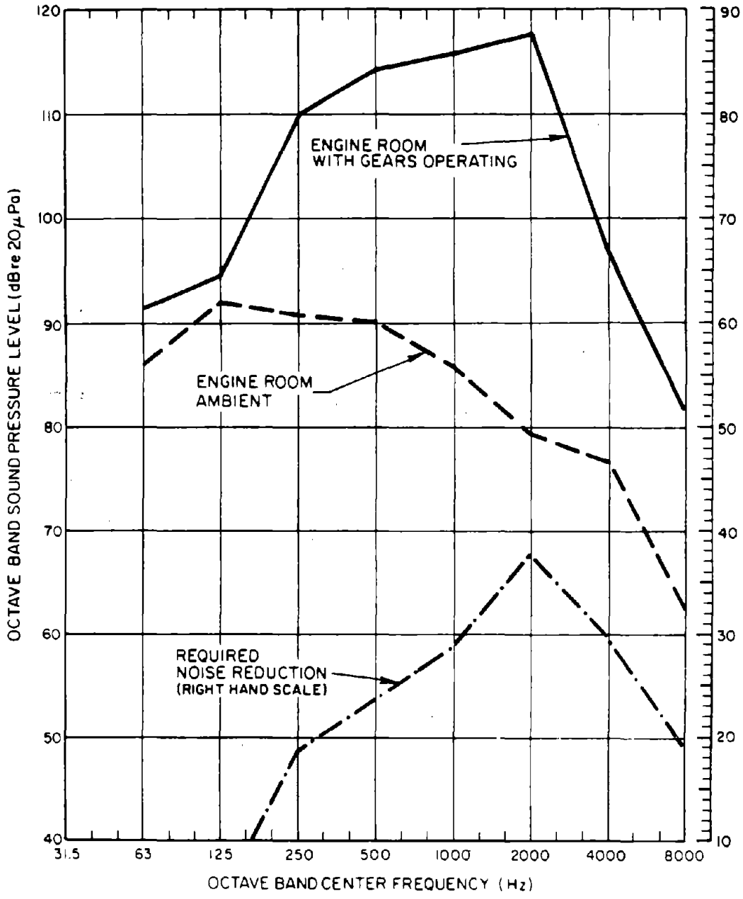
Figure 6.32.1. Engine room sound pressure levels.
