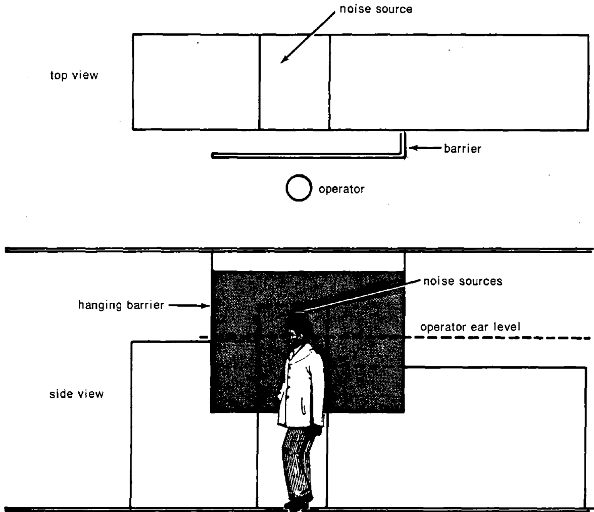
Figure 6.54.4. Sketch of hanging barrier for cut-punch press.
