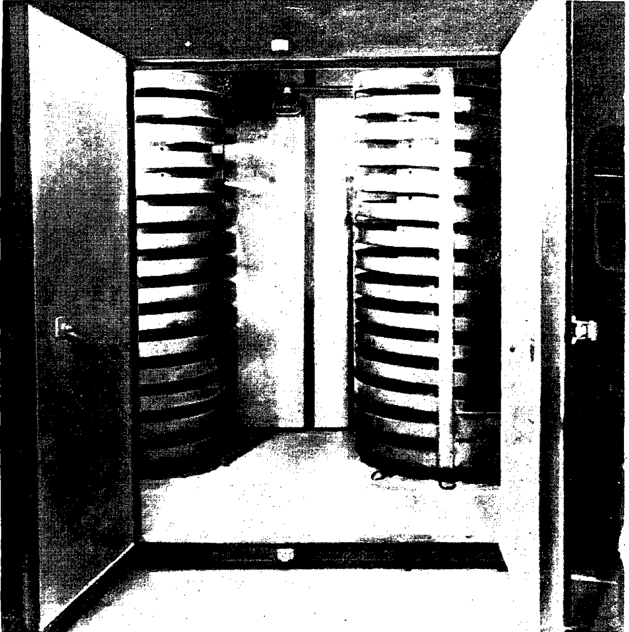
Figure 6.29.1. Detail of acoustic enclosure: doors.
