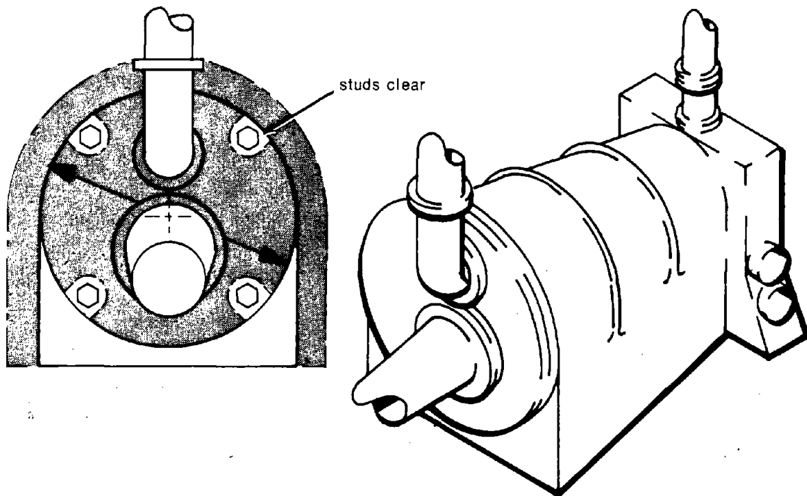
Figure 6.36.1. Noise reduction lagging for Jordan shell.
