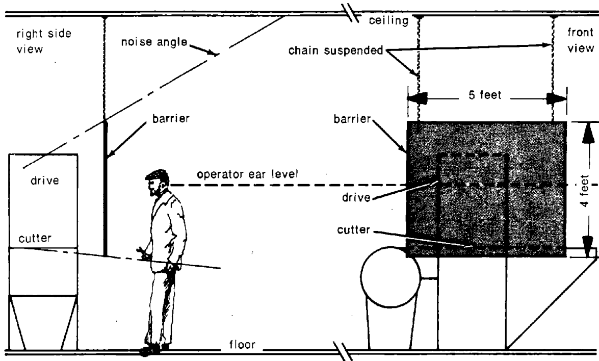
Figure 6.16.5. Barrier wall for straight-and-cut machine.
