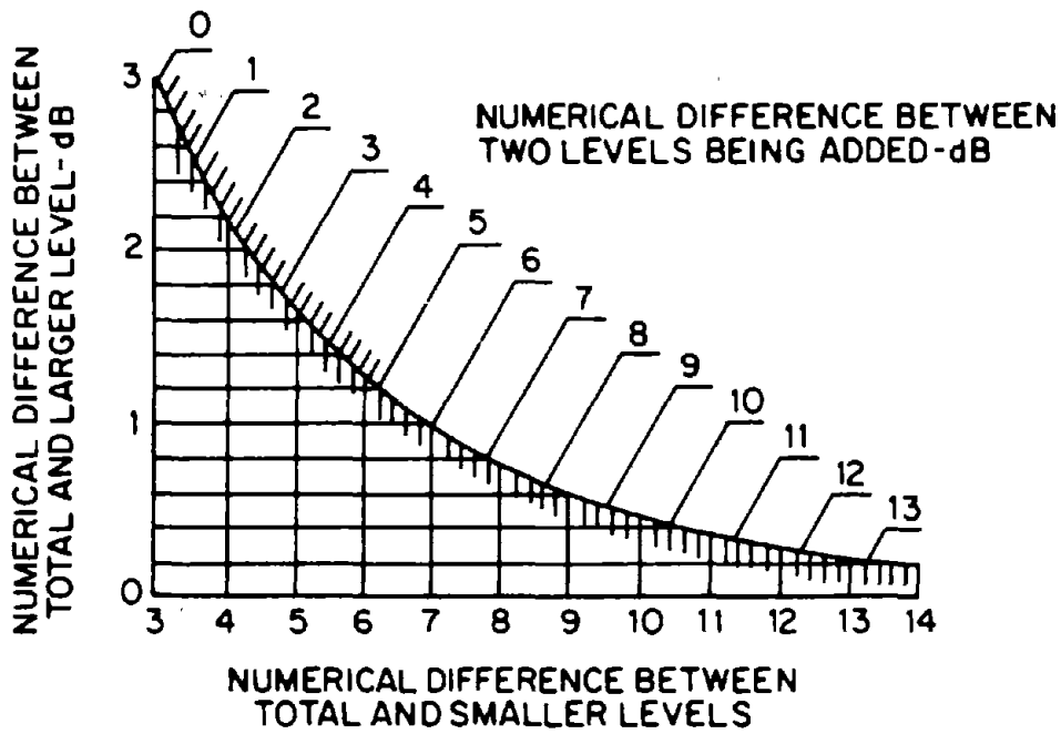
Figure 2.7. Chart for combining decibel levels*.
