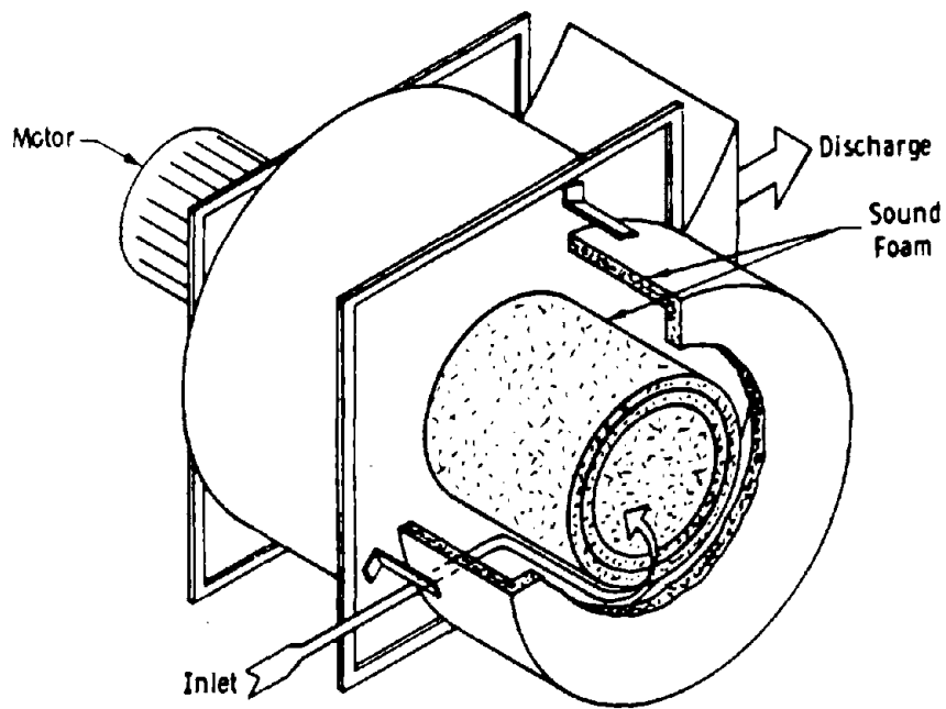
Figure 6.50.2. Essential features of the muffler.
