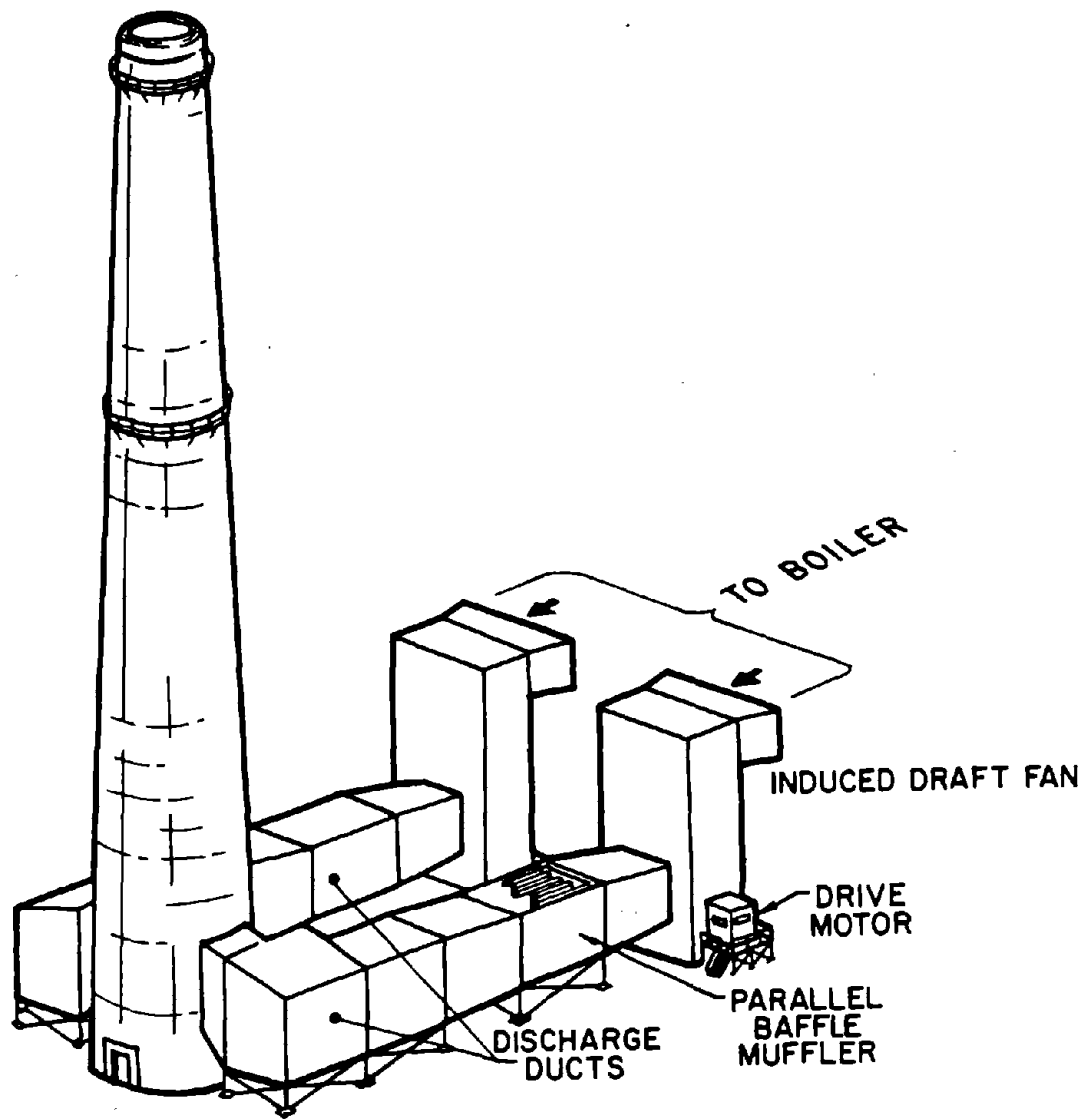
Figure 6.41.1. Induced draft fan system layout.
