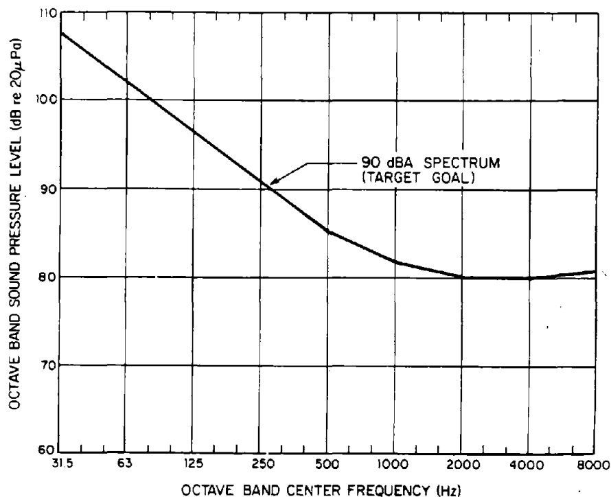
Figure 2.5. Recommended frequency spectrum for OSHA noise problems.
