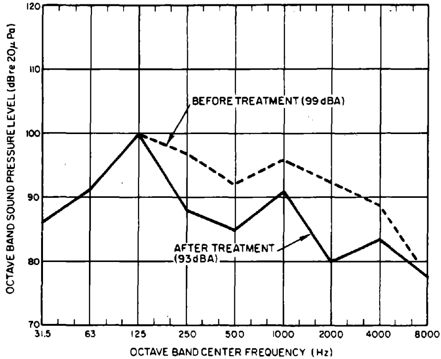
Figure 6.10.2. Quasi-peak readings of blanking press after ram ringing was contained.
