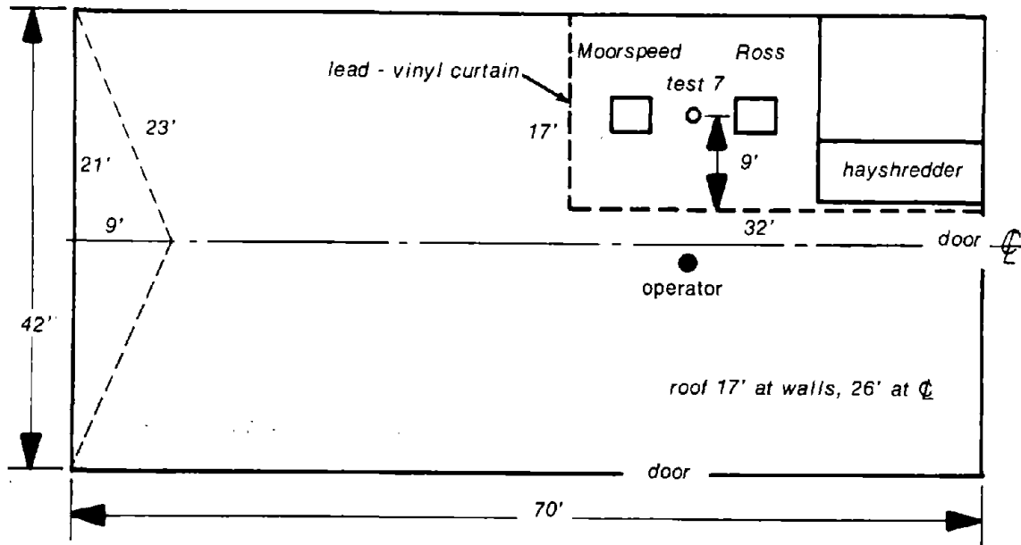
Figure 6.52.2. Floor plan of barley mill.
