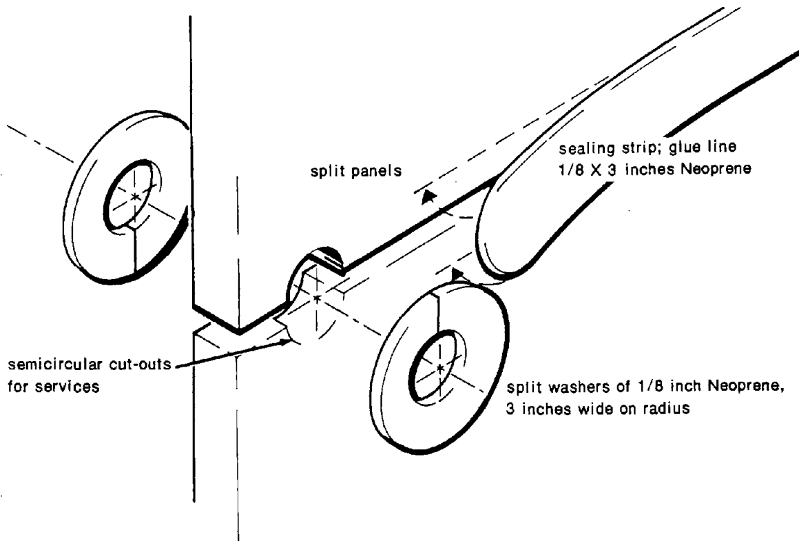
Figure 3.3. Split panels for services.
