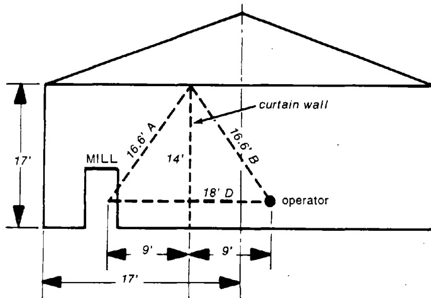
Figure 6.52.3. Sectional view of barley mill.
