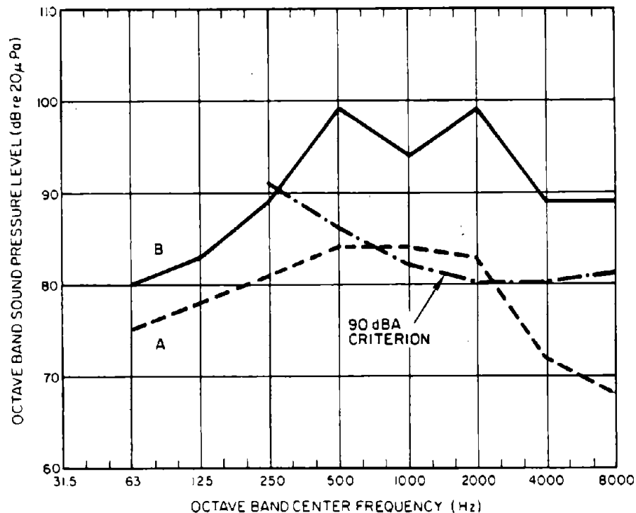
Figure 6.54.1. Cut-punch press operator position sound pressure levels. A, idling; B, punching.
