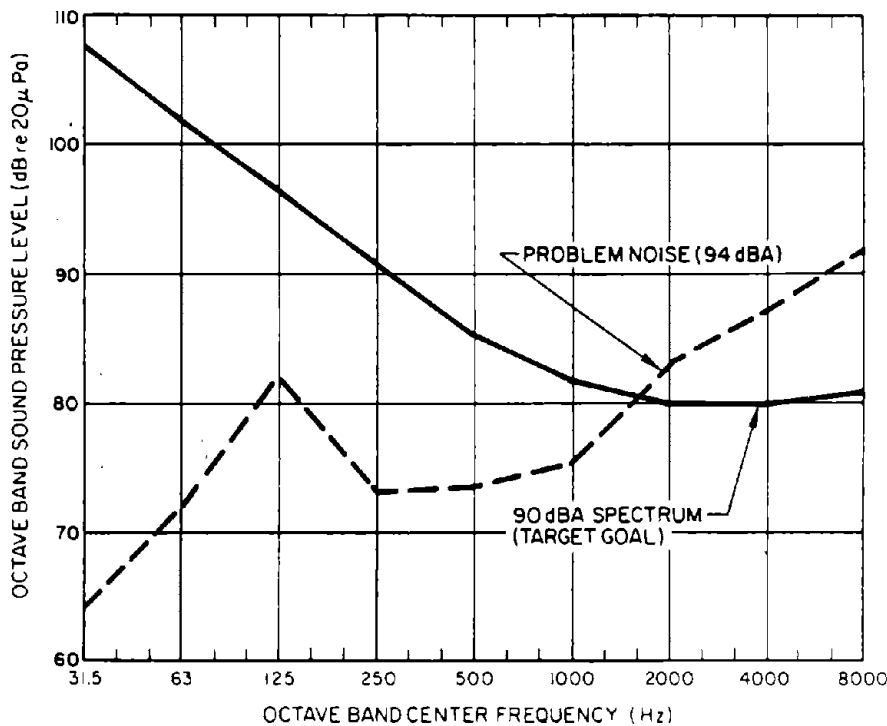
Figure 2.6. Determination of required noise reduction.
