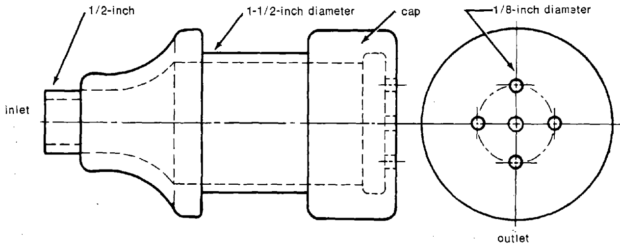
Figure 6.53.5. Design of nozzle.
