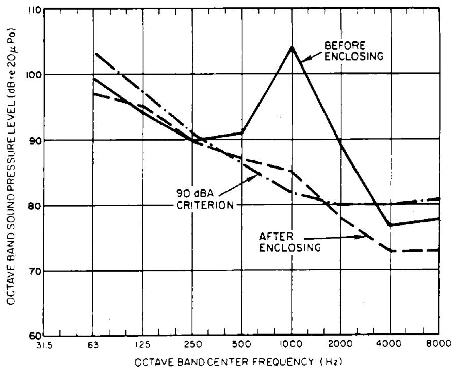
Figure 6.33.1. Measurements near boiler feed pump.
