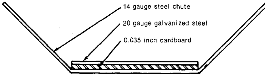
Figure 6.6.1. Chute for conveying cartridge cases.
