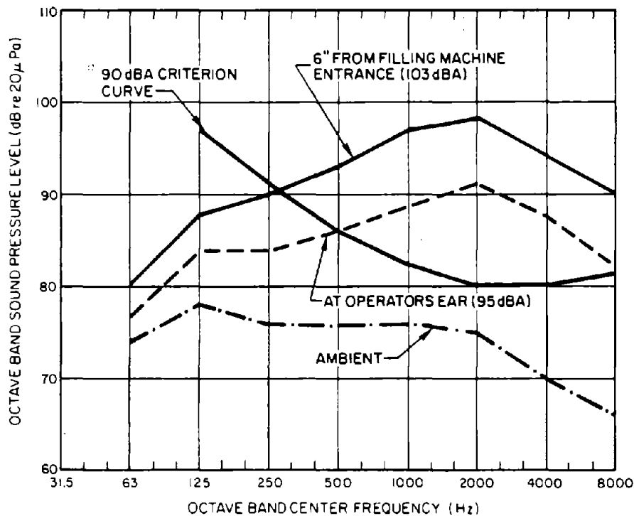
Figure 6.31.3. Sound pressure levels in filling machine room.
