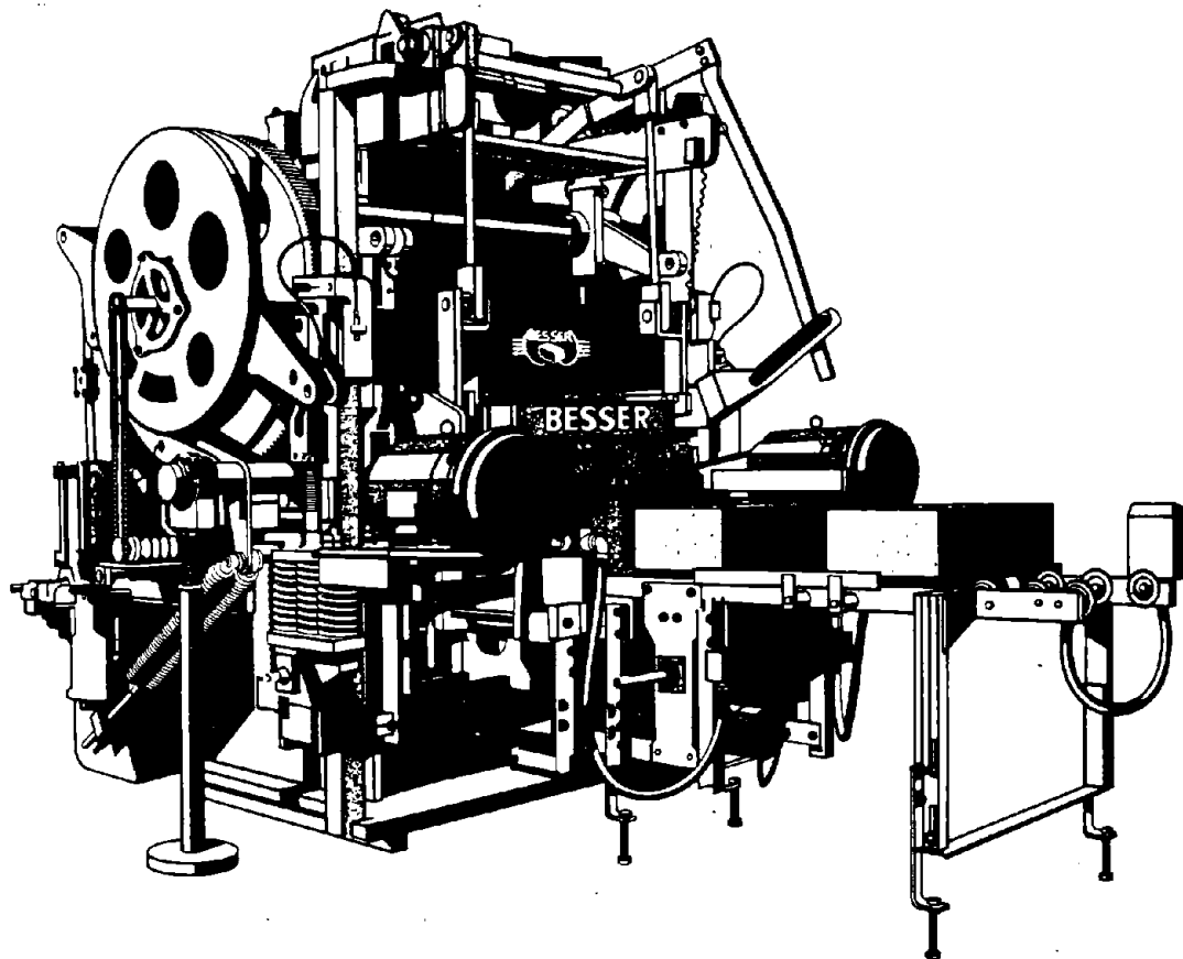
Figure 6.35.1. Typical concrete block manufacturing machine.
