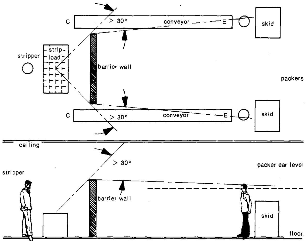
Figure 6.14.1. Air hammer stripper and packer line.
