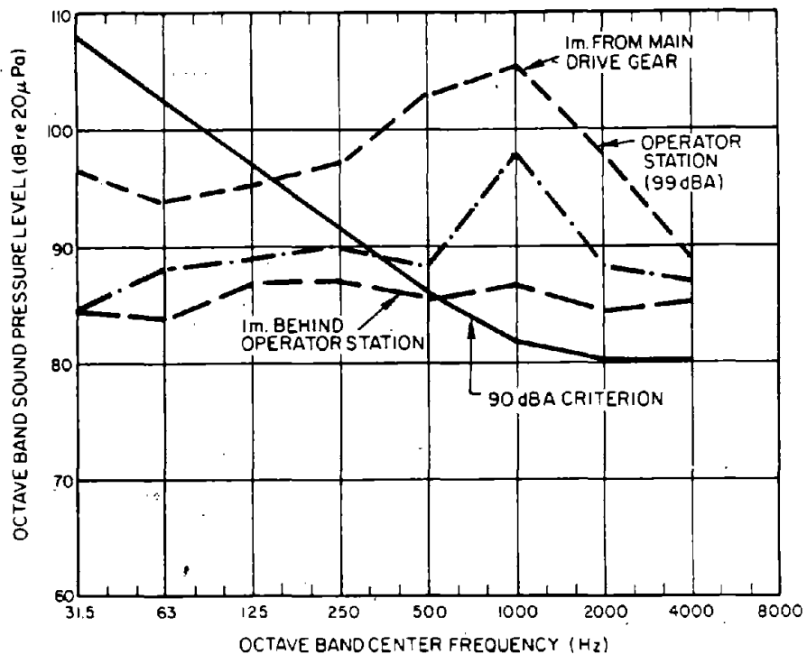
Figure 6.51.1. Sound pressure levels at 8-ft fabric machine.
