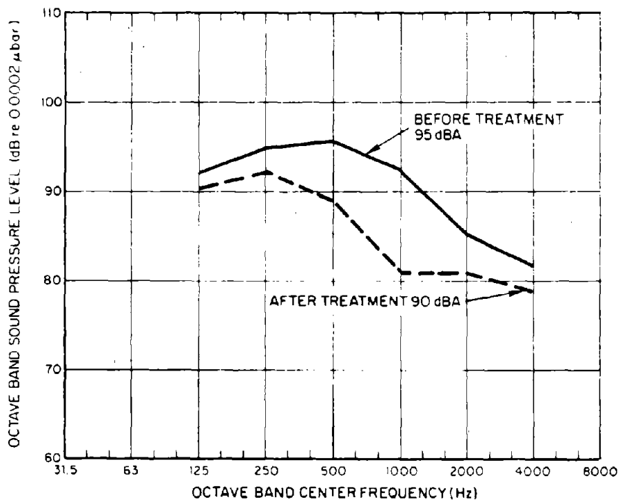
Figure 6.2.1. Reduced aisle sound levels, as predicted.
