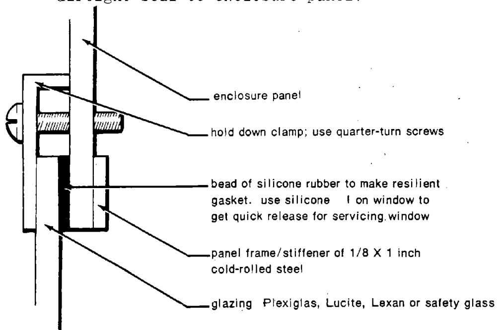
Figure 3.9. Window detail.
