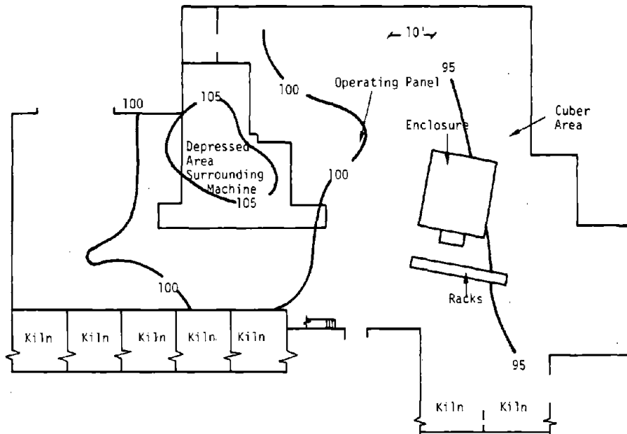
Figure 6.35.5. Plant 2: maximum sound level contours (enclosed machine operating).
