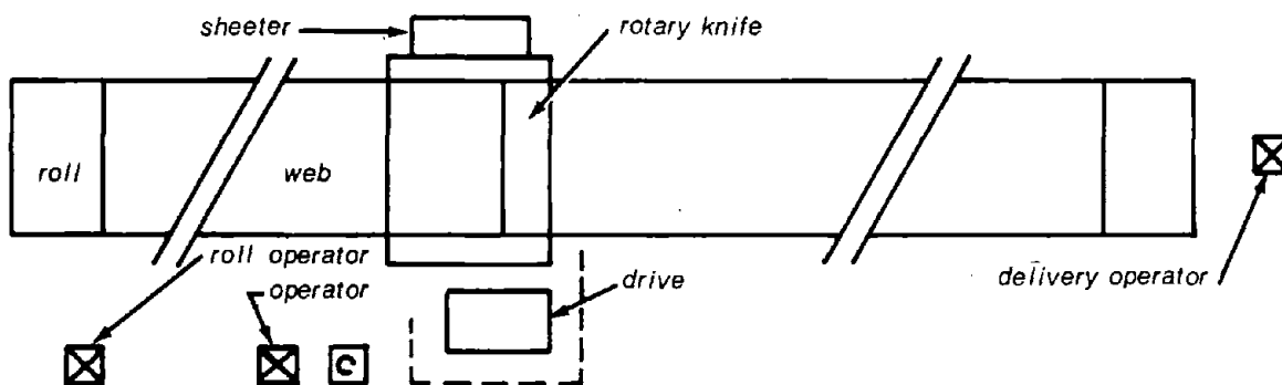
Figure 6.12.3. Layout of sheeter and operators.
