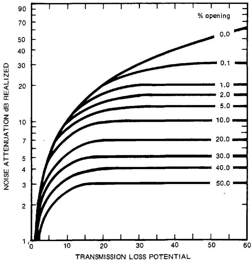
Figure 3.11. Effect of enclosure sound leaks on potential noise reduction.
