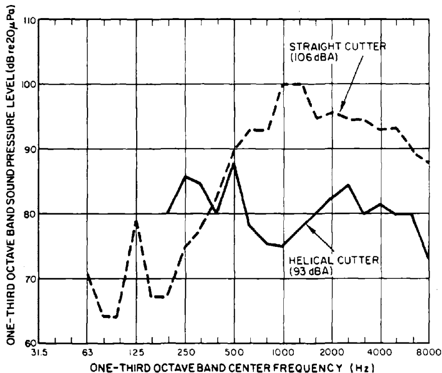
Figure 6.47.1. Before-and-after third-octave-band sound pressure levels for wood planer.
