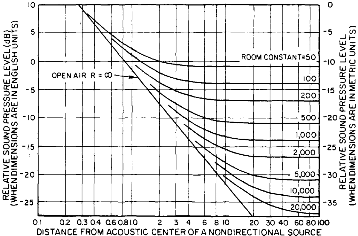
Figure 2.12. Sound level distribution in spaces with various room constants.
