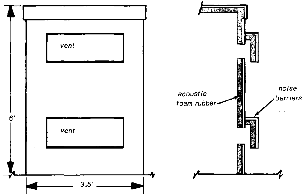
Figure 6.12.2. Sheeter drive box enclosure.
