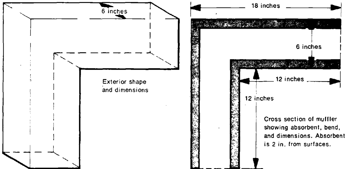
Figure 6.38.4. Motor exhaust muffler.
