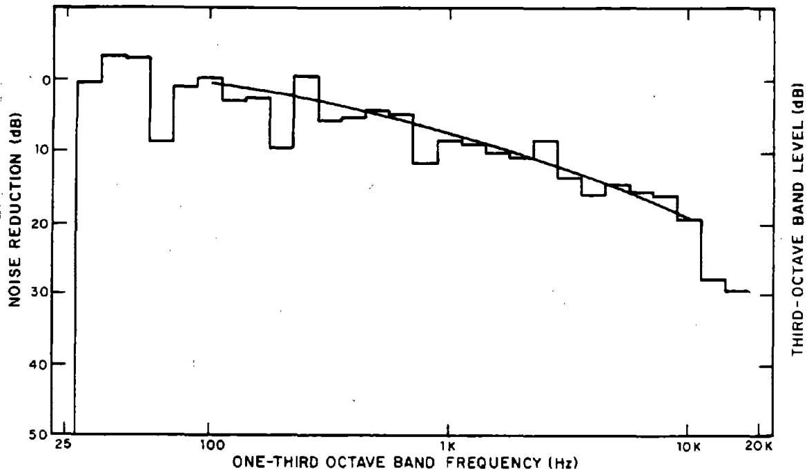
Figure 6.8.2. Noise reduction from damping.
