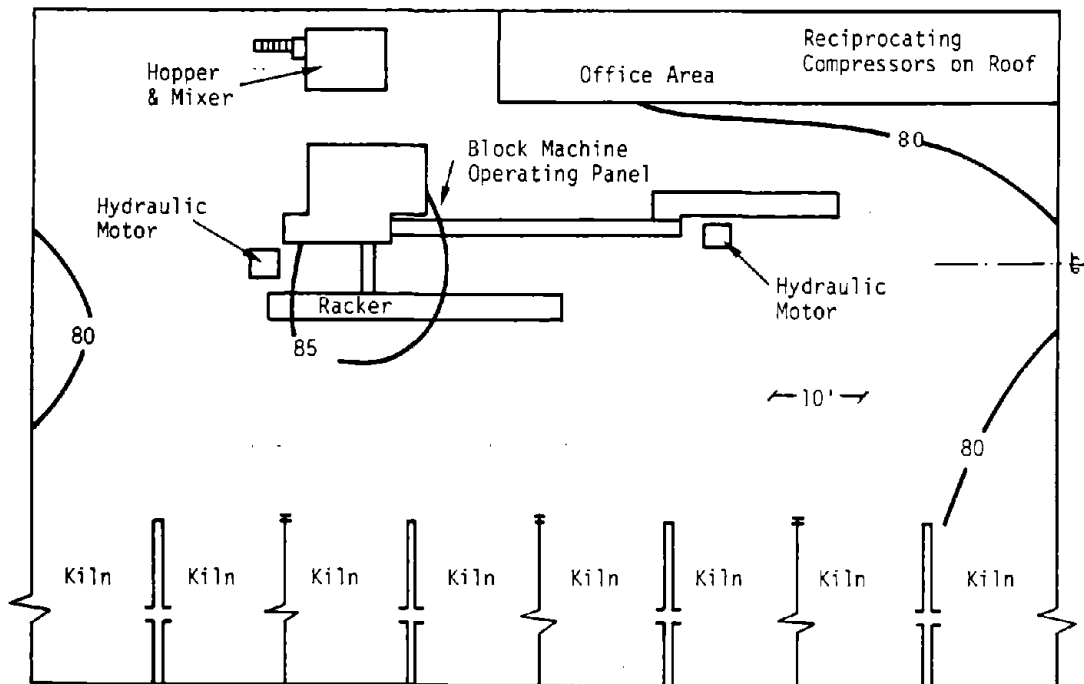
Figure 6.35.6. Plant 3: maximum sound level contours.
