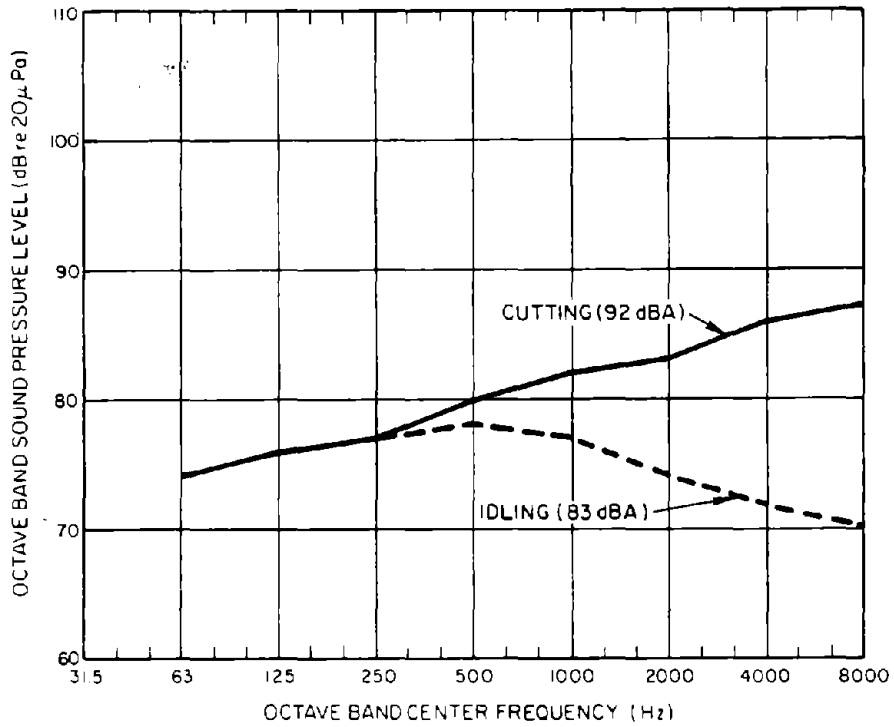
Figure 6.16.3. Straight-and-cut machine: operator's nearfield exposure.
