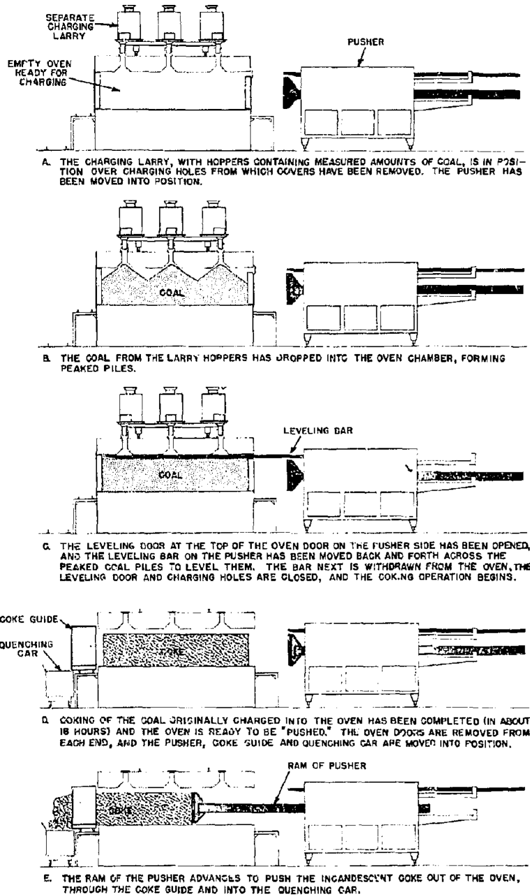
Figure 2. Schematic representation of the sequence of operations in charging, leveling, and pushing in one coking cycle of a by-product coke oven. (Copyright 1971 by United Steel Corporation.) (Used with permission)
