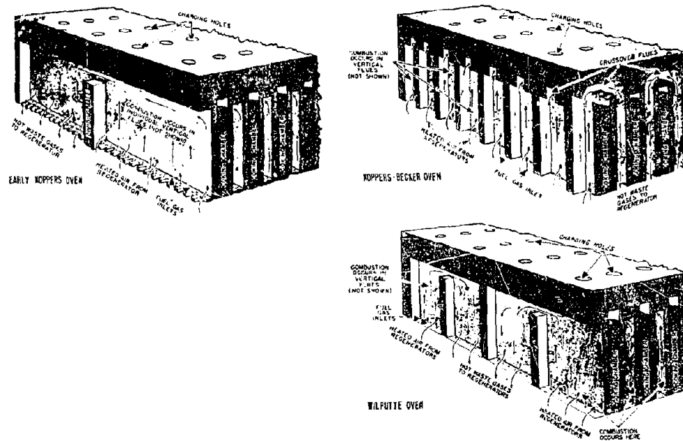
Figure 1. Schematic representation of the differences in firing methods employed in the three most common types of coke ovens. Individual flues are not shown. The firing procedures shown are for a single phase of heating which is reversed at the end of a specified period. (Copyright 1971 by United States Steel Corporation.) (Used with permission)
