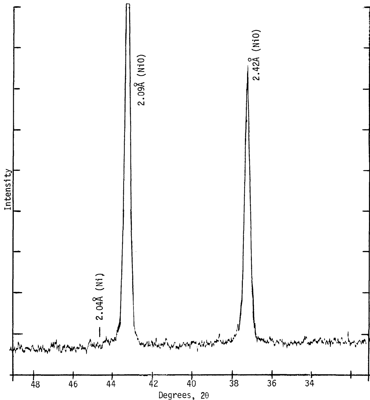
Figure 6. Segment of the XRD pattern of N-21 (nickel oxide) showing no Ni metal peak.
