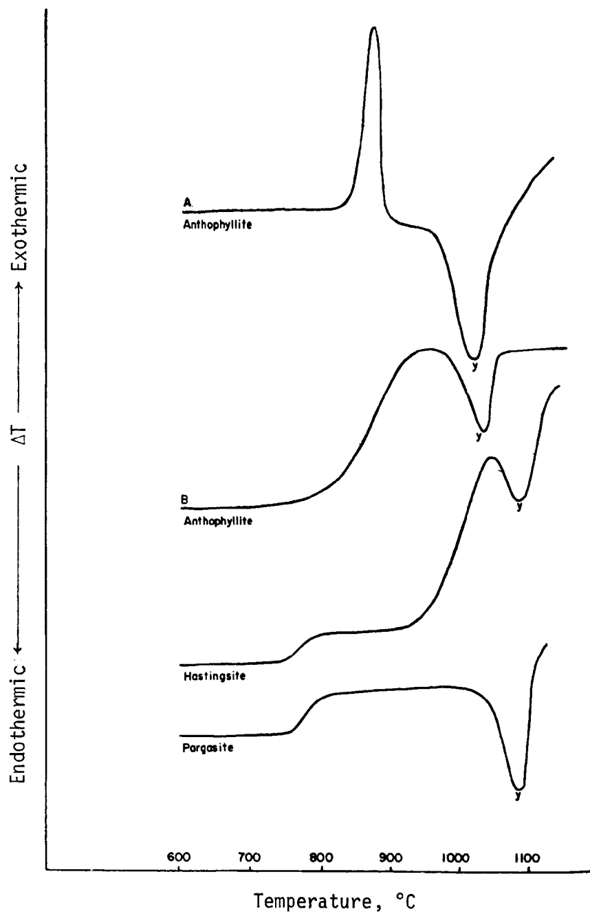
Figure 68. Thermographic curves of amphiboles. 38 (Reprinted with Permission)
