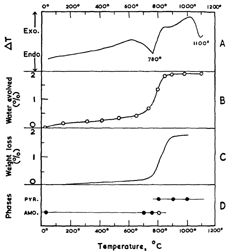
Figure 69. Dynamic heating in argon (amosite specimen PRS 5):
