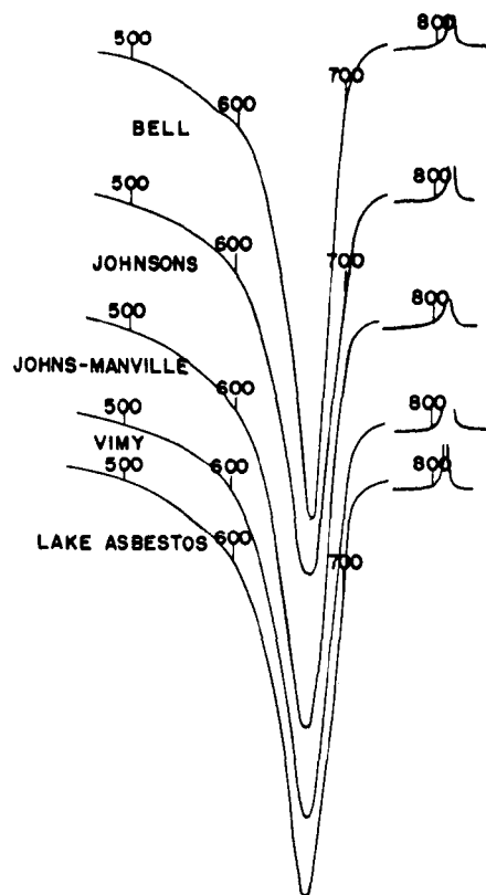
Figure 56. DTA peaks of chrysotile samples from various sources. Samples were prepared following a standard procedure of grinding for 180 sec in Wig-L-Bug. 29 (Reprinted with Permission)
