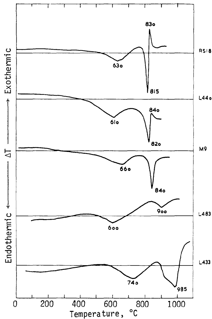
Figure 63. DTA curves of crocidolite in argon:
