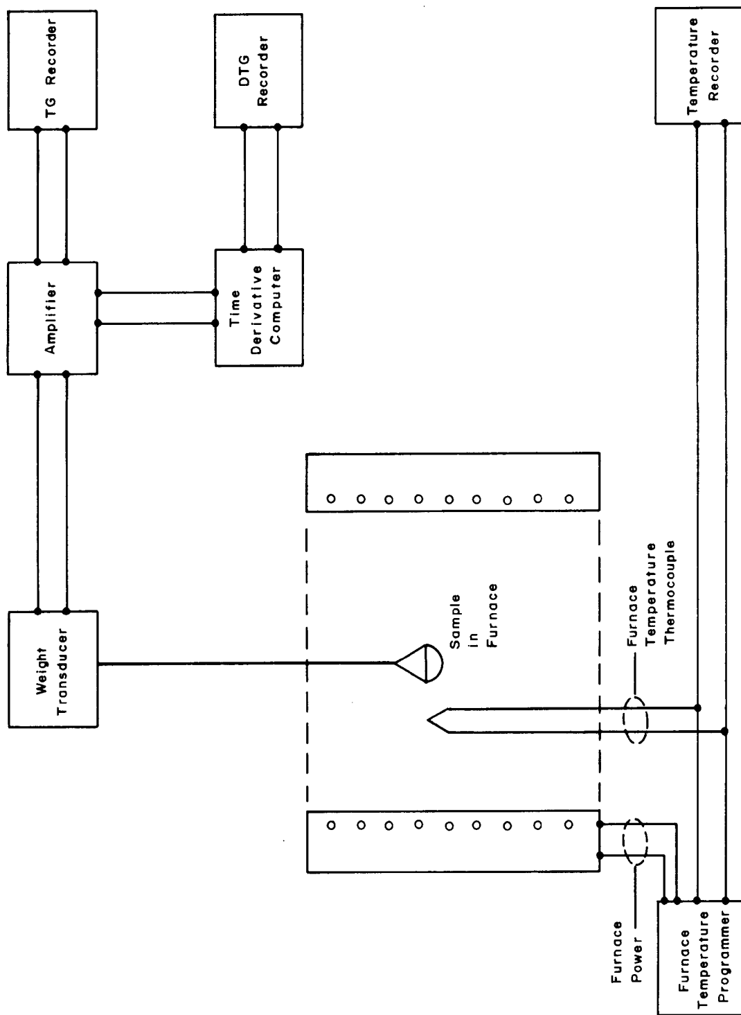
Figure 11. Block diagram of the TGA apparatus.
