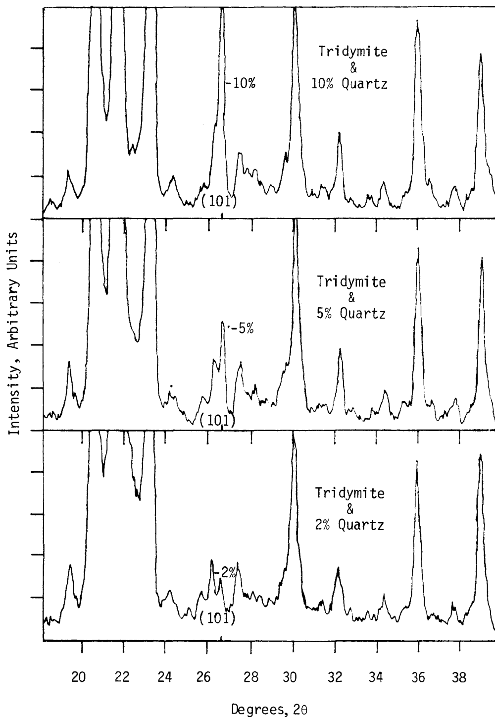
Figure 2. Detectability of quartz in tridymite on basis of (101) peak of quartz. Mixtures are of 10%, 5%, and 2% quartz in tridymite, batch #19, Cu K\alpha , 2^\circ\theta/\text{min} .
