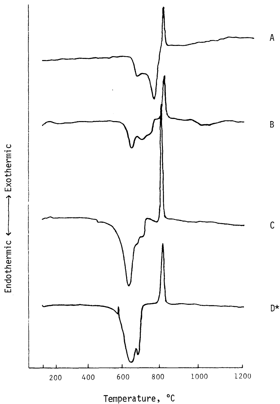
Figure 14. DTA patterns of antigorite samples:
