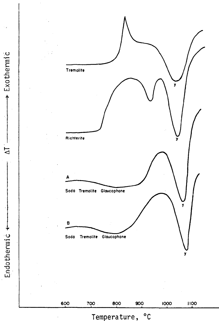
Figure 67. Thermographic curves of amphiboles. 38 (Reprinted with Permission)
