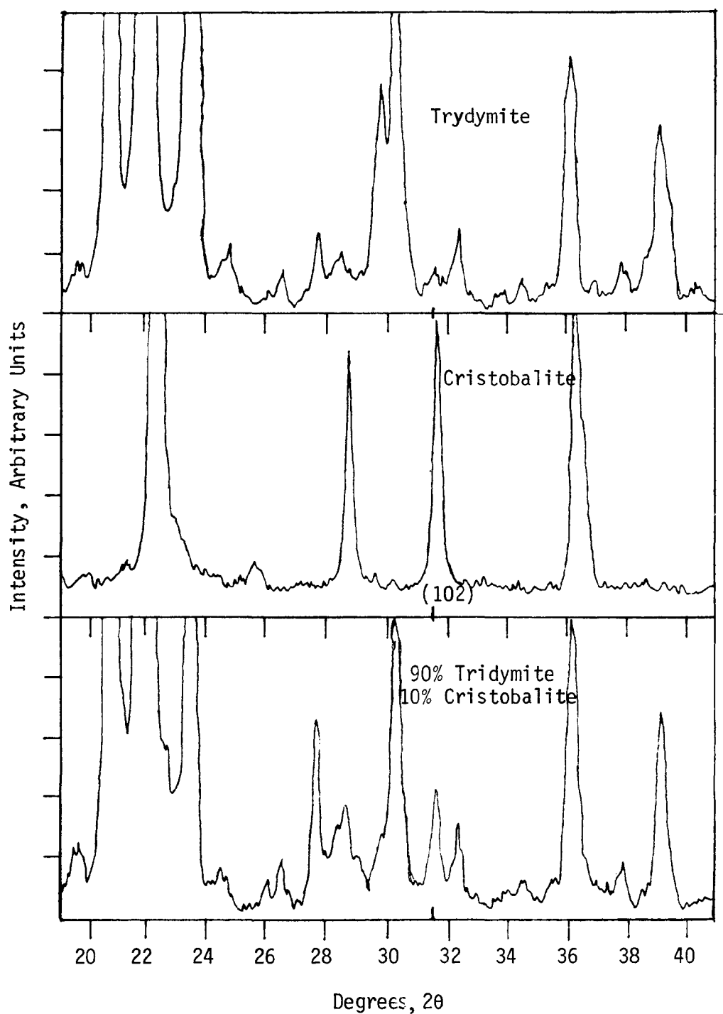
Figure 3. Detectability of cristobalite in tridymite based on the use (102) peak of cristobalite at 31.49^\circ 2\theta .
