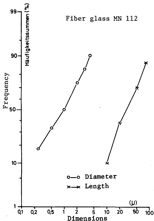
FIGURE 17-2. DISTRIBUTION OF DIAMETER AND LENGTH OF FIBROUS GLASS MN 112
