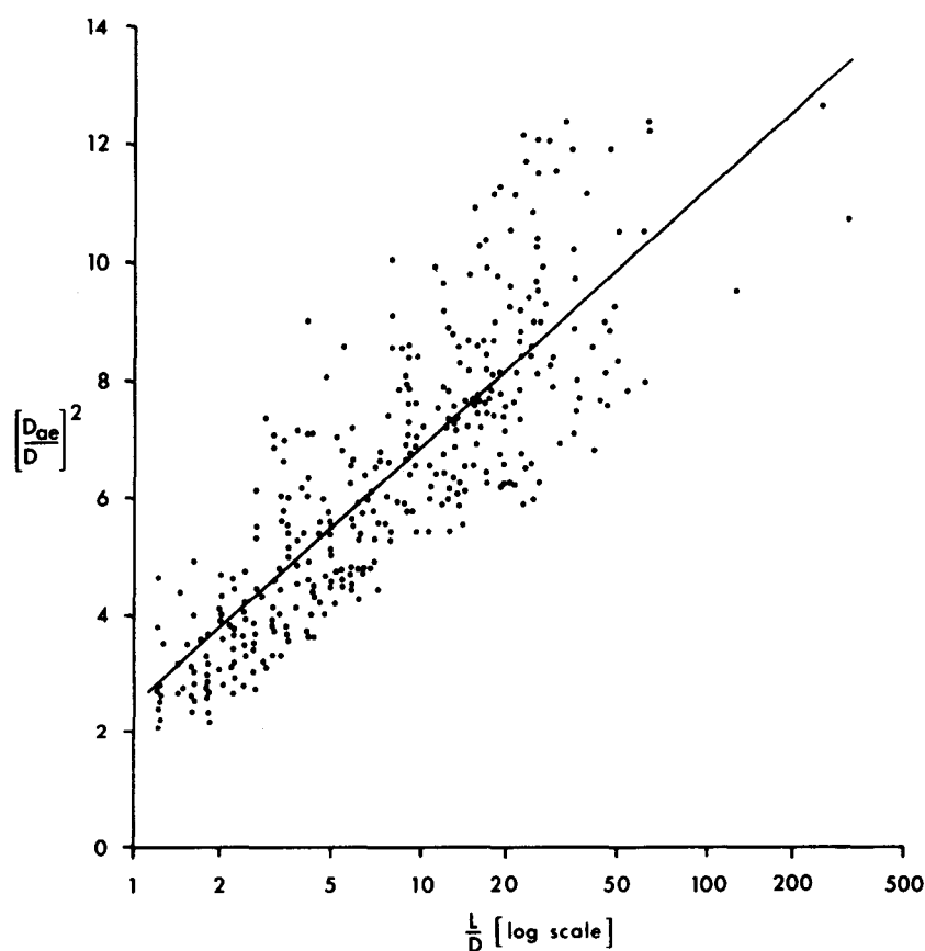
FIGURE 4-3. RELATION BETWEEN LENGTH AND AERODYNAMIC DIAMETER OF GLASS FIBERS (2.25g/cc) IN UNITS OF FIBER DIAMETER
