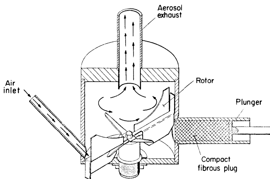
FIGURE 7-1. FIBROUS AEROSOL GENERATOR
