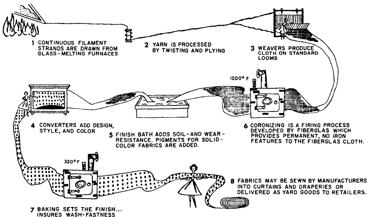
FIGURE 2-5. HOW FABRICS ARE MADE FROM GLASS FIBER YARN
