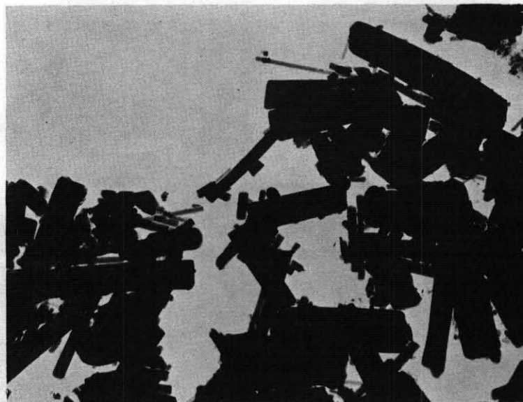
FIGURE 13-2. ELECTRON MICROGRAPH OF FIBERS MILLED TO AVERAGE LENGTHS LESS THAN 20\ (\mu) . MAGNIFICATION X 10,000
