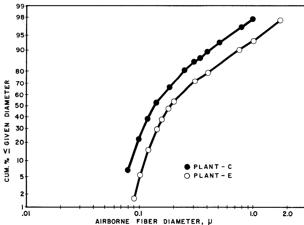
FIGURE 10-3. AIRBORNE FIBER DIAMETER DISTRIBUTION, SMALL DIAMETER FIBER PRODUCTION
