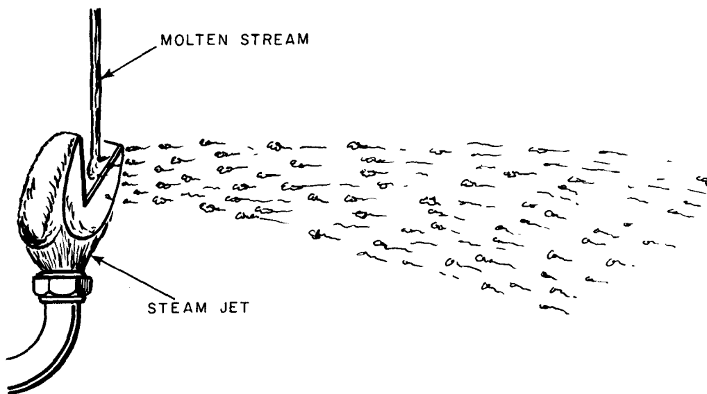
FIGURE 1-2. SHOT PROPELLED FIBERIZATION
