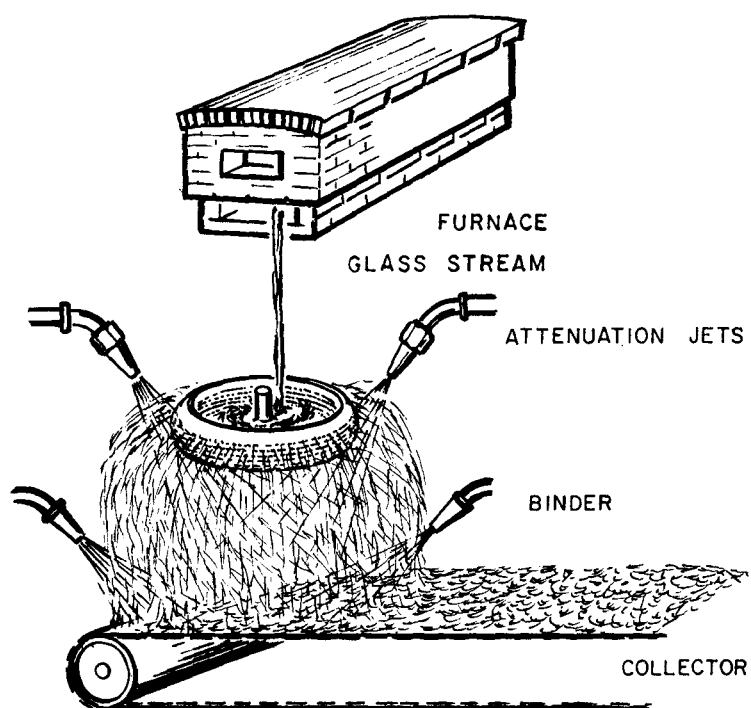
FIGURE 1-8. ROTARY PROCESS
