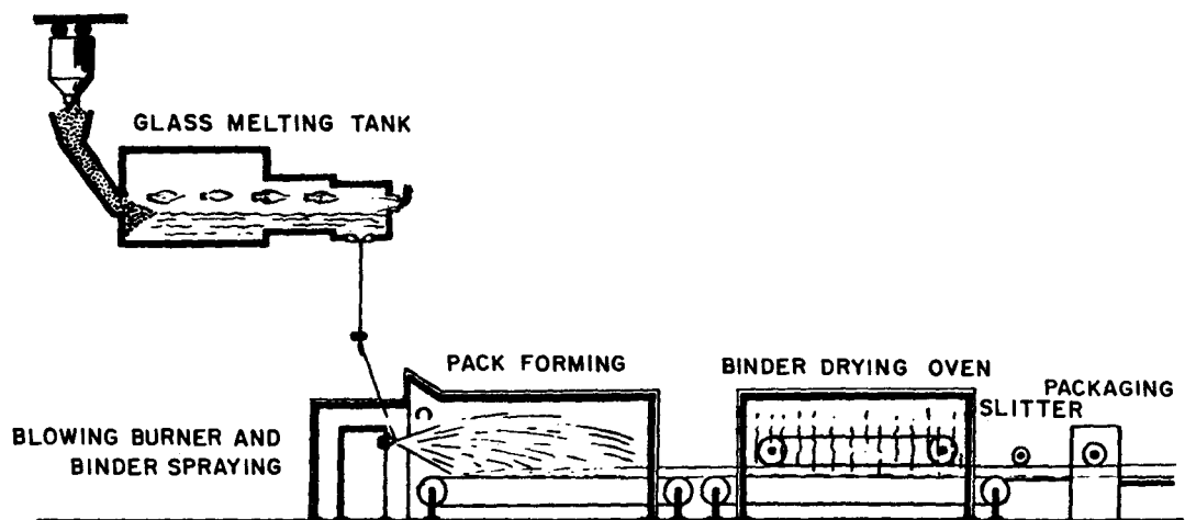
FIGURE 2-2. SUPERFINE WOOL FORMING LINE
