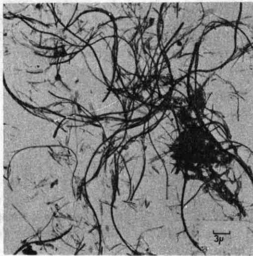
FIGURE 4-5. ELECTRON MICROGRAPH OF CHRYSOTILE ASBESTOS
