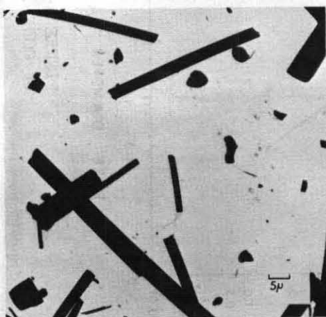
FIGURE 4-8. ELECTRON MICROGRAPH OF CODE 110 GLASS MICRO-FIBER
