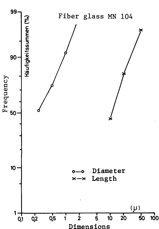
FIGURE 17-1. DISTRIBUTION OF DIAMETER AND LENGTH OF FIBROUS GLASS MN 104
