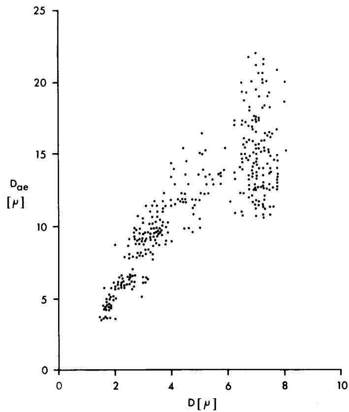
FIGURE 4-2. RELATION BETWEEN DIAMETER AND AERODYNAMIC DIAMETER OF GLASS FIBERS (2.25g/cc)
