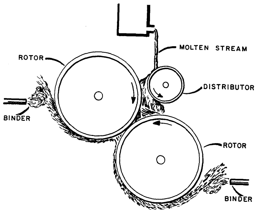
FIGURE 1-3. POWELL PROCESS
