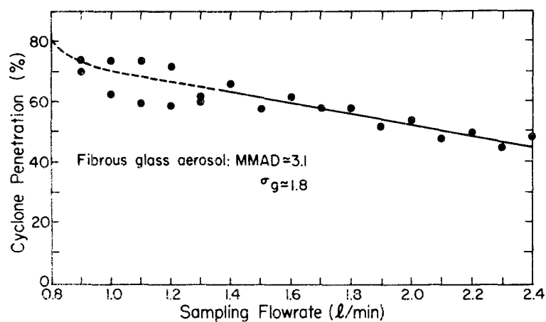
FIGURE 7-5. CYCLONE PENETRATION VS. SAMPLING FLOWRATE: O/C AAA-10 FIBROUS GLASS
