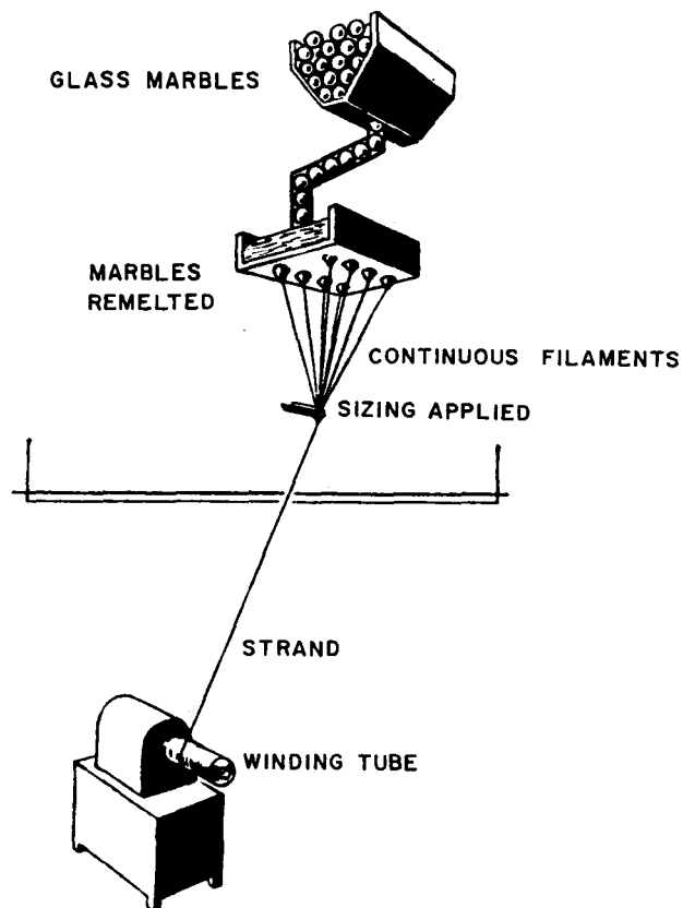
FIGURE 2-4. CONTINUOUS FILAMENT YARNS PROCESS
