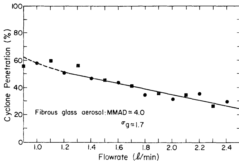
FIGURE 7-6. CYCLONE PENETRATION VS. SAMPLING FLOWRATE: TYPE O/C AA 10 FIBROUS GLASS
