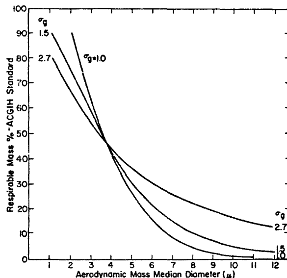
FIGURE 7-3. RESPIRABLE MASS--ACGIH STANDARD--AS A FUNCTION OF AERODYNAMIC MASS MEDIAN DIAMETER FOR POLYDISPERSE AEROSOLS
