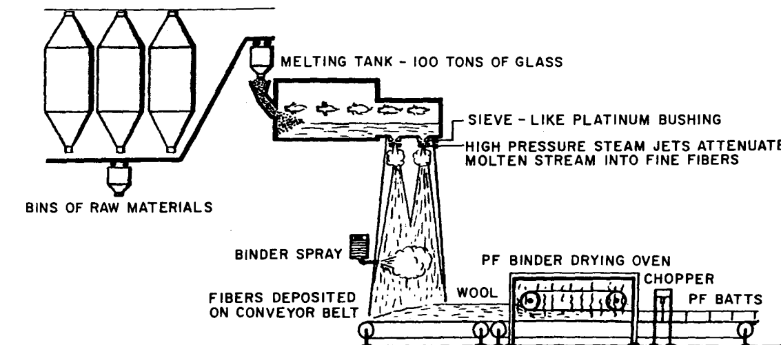
FIGURE 2-1. GLASS FIBER WOOL FORMING LINE
