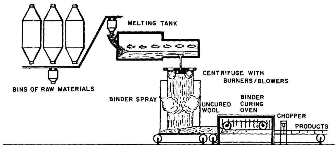
FIGURE 2-3. GLASS FIBER WOOL CENTRIFUGAL FORMING LINE
