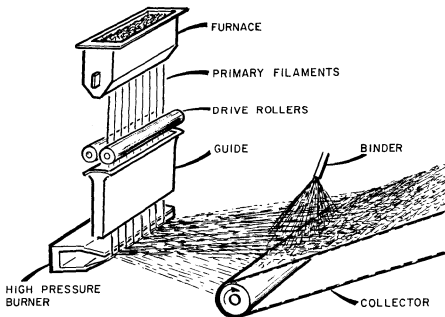
FIGURE 1-9. FLAME-ATTENUATION PROCESS
