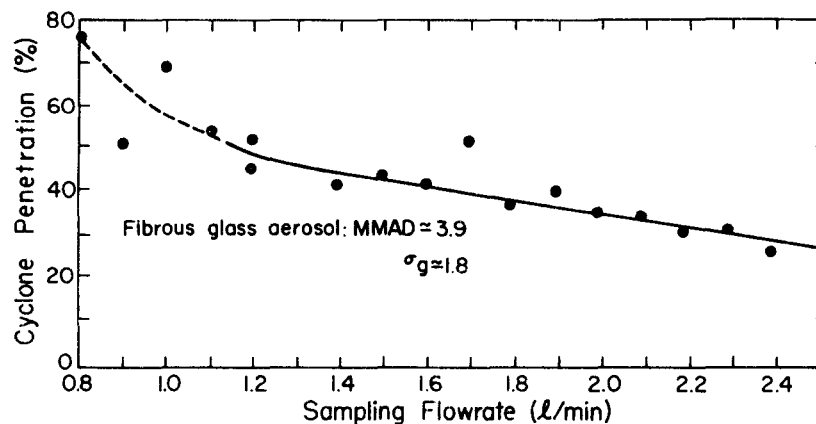
FIGURE 7-4. CYCLONE PENETRATION VS. SAMPLING FLOWRATE: O/C TYPE E, AA-12 FIBROUS GLASS
