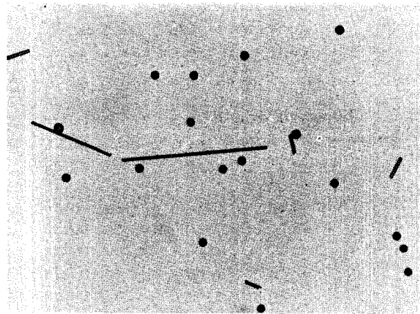
FIGURE 4-1. PHOTOMICROGRAPH OF AEROSOL SPECTROMETER SAMPLE OF SHELLAC SPHERES (1.1g/cc) AND GLASS FIBERS (2.25g/cc) OF THE SAME AERODYNAMIC DIAMETER
