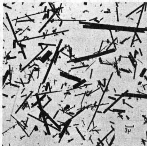
FIGURE 4-6. ELECTRON MICROGRAPH OF AMPHIBOLE (AMOSITE) ASBESTOS
