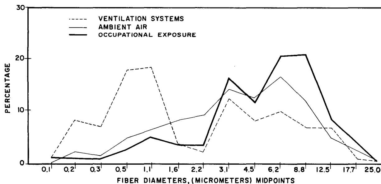
FIGURE 8-1. DISTRIBUTION OF GLASS FIBERS BY DIAMETERS AND SAMPLING LOCATION
