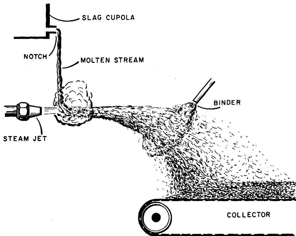
FIGURE 1-1. STEAM JET FIBERIZATION
