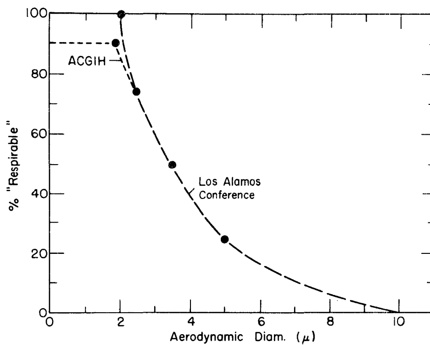
FIGURE 7-2. RESPIRABLE FRACTION AS A FUNCTION OF PARTICLE AERODYNAMIC DIAMETER
