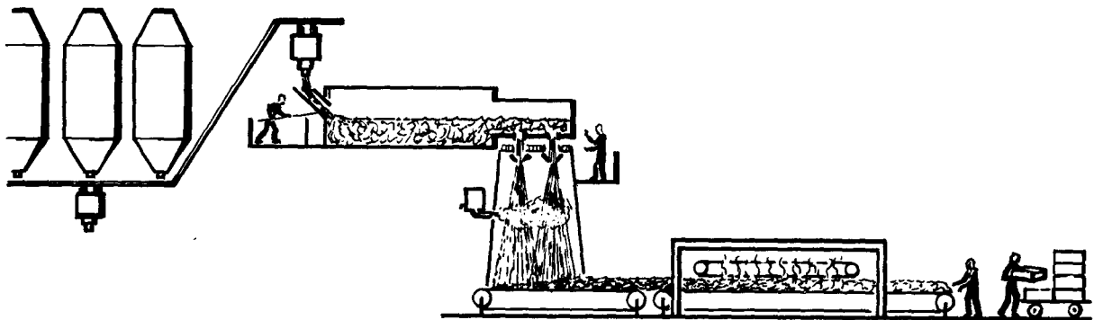
FIGURE 1-7. WOOL MANUFACTURING PROCESS
