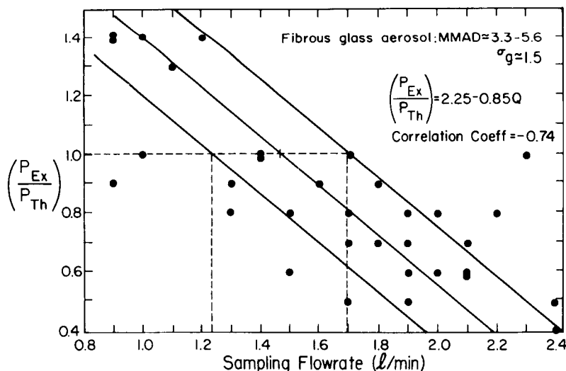
FIGURE 7-7. RATIO OF EXPERIMENTAL TO PREDICTED CYCLONE PENETRATION VS. SAMPLING FLOW RATE: SWEDISH WOOL FIBROUS GLASS
