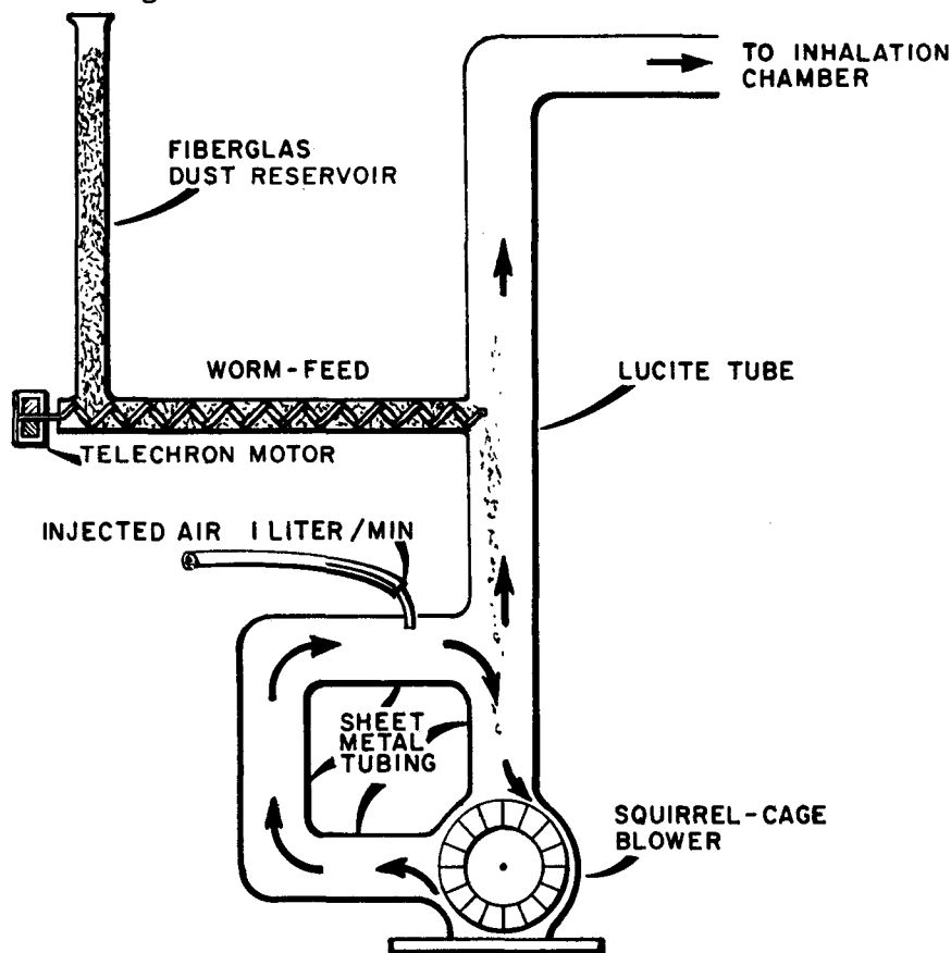
FIGURE 15-1. DIAGRAM OF DUST-DISPENSING APPARATUS
