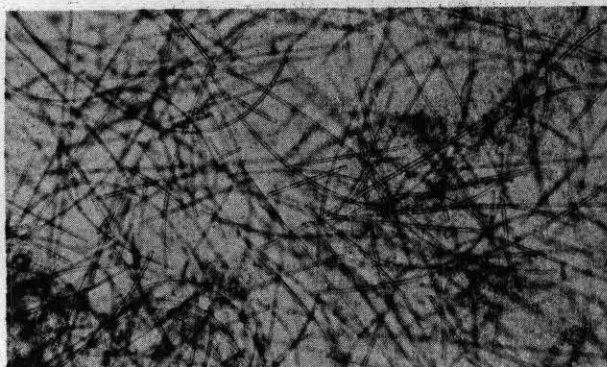
FIGURE 19-3. GLASS FIBERS IN ASH OF COTTON KNIT FABRIC LAUNDERED WITH GLASS FABRIC. (DE, CONTINUOUS DYED, X 126)
