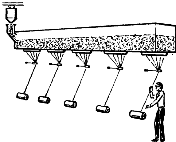
FIGURE 1-5. DIRECT MELT CONTINUOUS FILAMENT TEXTILE PROCESS
