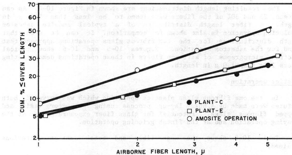
FIGURE 10-4. AIRBORNE FIBER LENGTH DISTRIBUTIONS, SMALL DIAMETER FIBER PRODUCTION.
