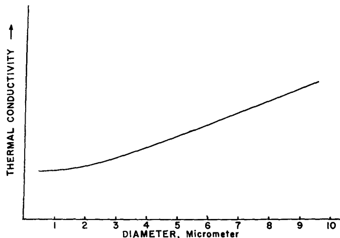
FIGURE 1-10. THERMAL CONDUCTIVITY AS A FUNCTION OF FIBER DIAMETER
