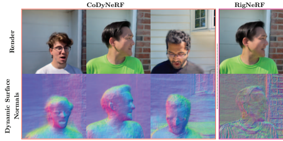
Figure 4. Dynamic Surface Normals. Surface normals directly influence the specularities and shading of the human head. Here we visualise the surface normals given by the density field of CoDyNeRF. As can be seen, the normals are able to capture the dynamic foreground with fine detail without sacrificing accuracy. In comparison, the normals of RigNeRF [3] are noisy and fail to capture the facial geometry accurately.
