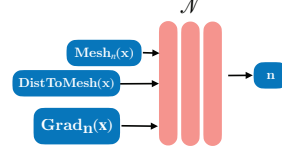
Figure 3. Normals Prediction Architecture. The Normals prediction network takes as input the mesh normals of a given point \mathbf{x} , its distance to the mesh and the normals given by gradient of the NeRF’s density field. The details of the architecture are discussed in Section 3.2.1.
