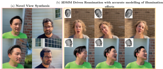
Figure 6. Applications of CoDyNeRF. CoDyNeRF enables the creation of Neural 3D Portraits captured in challenging lighting conditions with the accurate reproduction of illumination effects during novel expression and pose reanimation. In (a), we demonstrate that specularities, especially on the forehead and the nose, change realistically with changing viewing directions. In (b) we demonstrate the realistic reproduction of shading, shadows and specularities when the neural portrait is reanimated with a driving 3DMM (shown as white insets in the top left of each image). We see from results in the top row of (b) that the shading on the forehead and the specularities change realistically. Similarly, in the bottom row of (b) we see the nose being unshaded as the head rotates and the shadow cast by the ear changes realistically.
