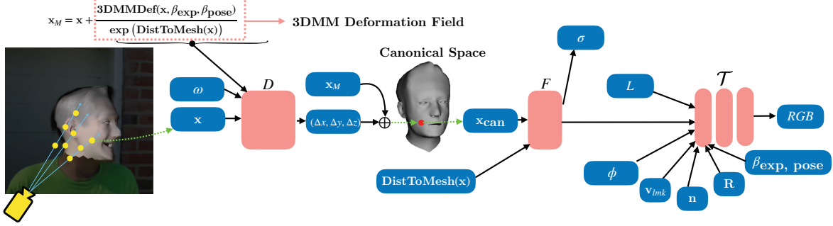
Figure 2. Overview of CoDyNeRF. CoDyNeRF is a deformable NeRF architecture that consists of three learnable MLPs: a deformation MLP D and density MLP F and a dynamic appearance MLP \mathcal{T} . Given an image, we shoot rays through each of its pixels. For every ray, we deform each point on it according to a 3DMM-guided deformation field similar to prior work [3]. Next, the deformed point is given as input to the color MLP, F , which predicts the density and neural features that are passed onto the dynamic appearance MLP \mathcal{T} . \mathcal{T} then takes as input normals, the reflection vector about the normal, the pose and expression deformations along with spherical harmonics shading and head landmark positions to predict dynamic RGB of the point. The final color of the pixel is calculated via volume rendering.
