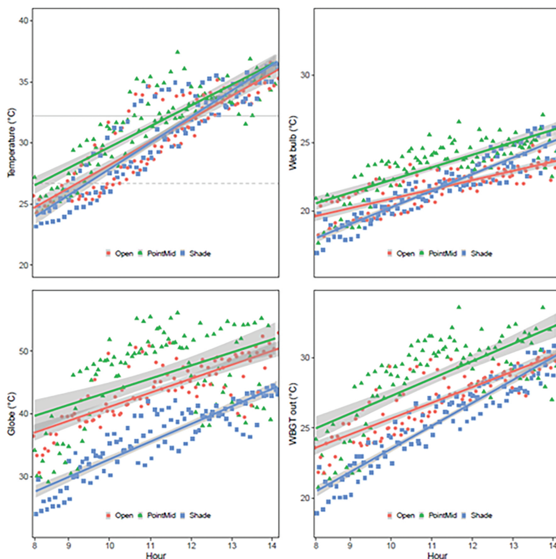
Figure 3. Dry Bulb Temperature, Black Globe Temperature, Wet Bulb Temperature, and WBGT out over time by location in the cherry block.
