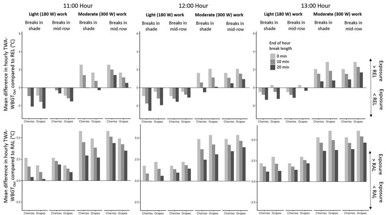
Figure 5. Differences** in hourly WBGT out exposures from NIOSH heat stress RALs and RELs for different break locations, workloads, and break times in cherry and grape fields.
