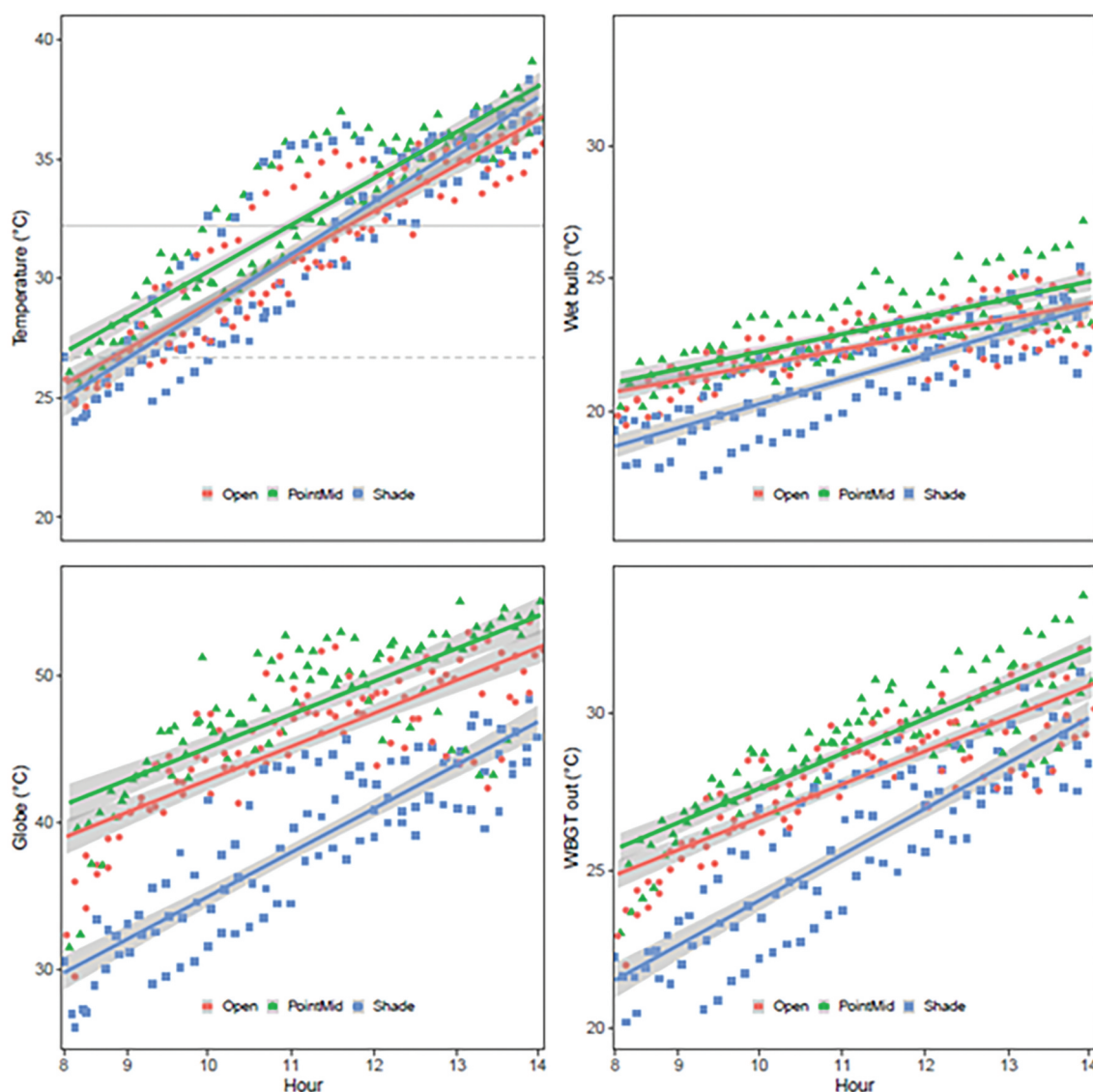
Figure 4. Dry Bulb Temperature, Black Globe Temperature, Wet Bulb Temperature, and WBGT out over time by location in the grape block.
