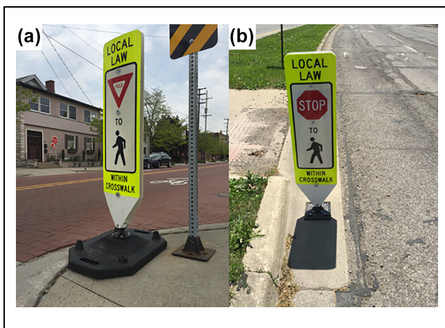
Figure 6. Examples of a (a) curb-top placement of the sign mounted on a temporary base and (b) a gutter-pan placement of the sign installed on a permanent flush mount.
