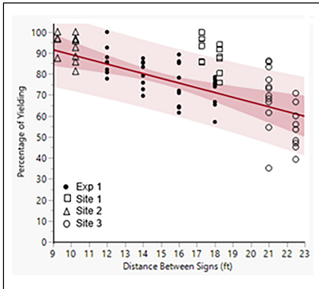
Figure 9. Yielding by distance between signs in Experiment 2 combined with yielding data from Experiment 1. Yielding scores for Sites 2 and 3 appear consistent with the linear relationship identified in Experiment 1. Yielding at Site 1 was higher than expected based on the distance between signs.
