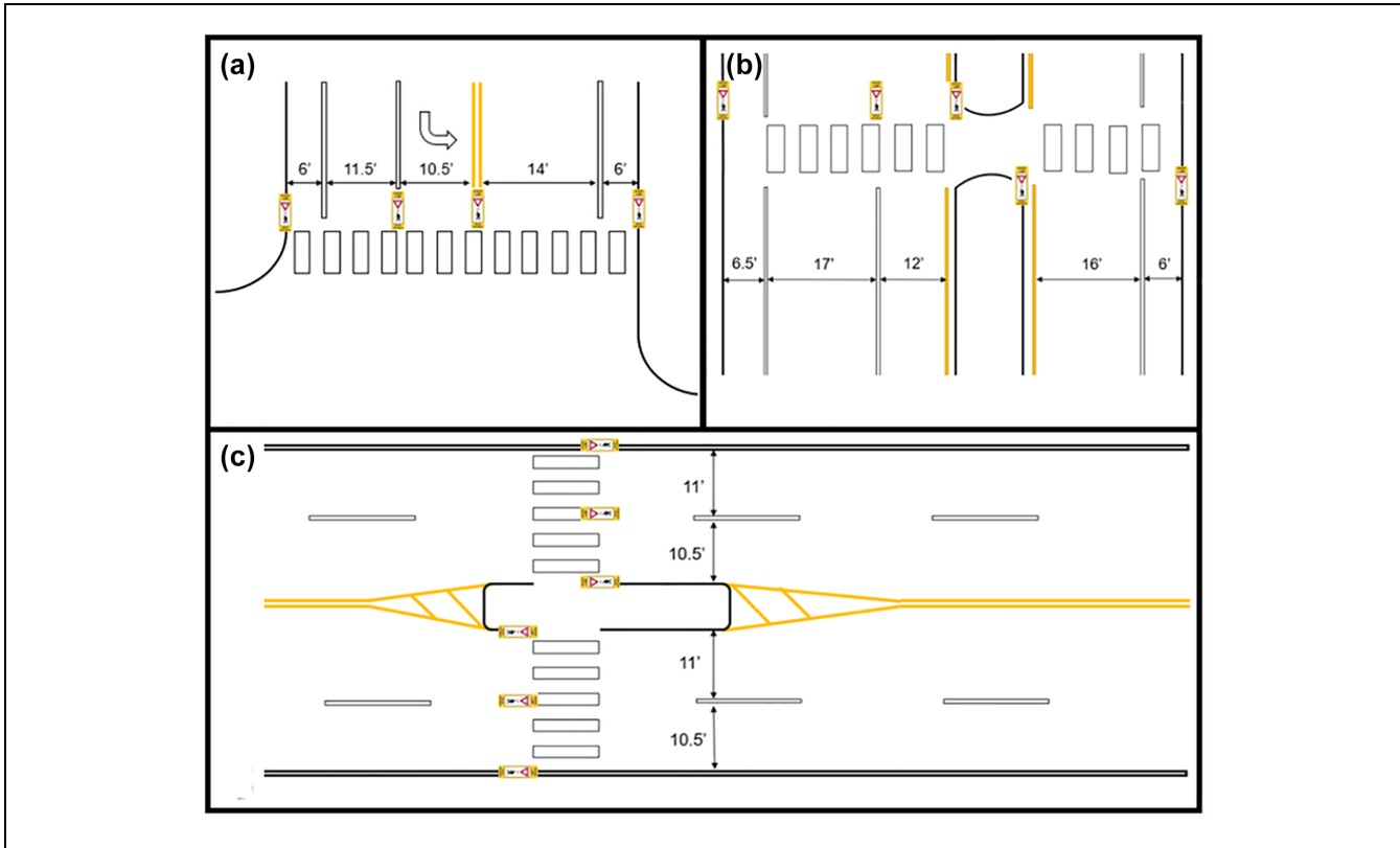
Figure 7. Diagram of approximate baseline lane widths and experimental sign positions for (a) Site 1, (b) Site 2, and (c) Site 3.
