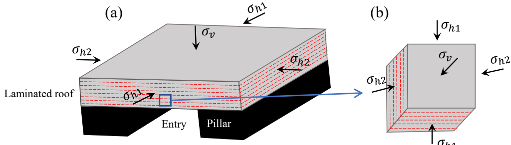
Fig. 3- 8 (a) Stress acting on the roof of an entry (b) a unit near the roof line
