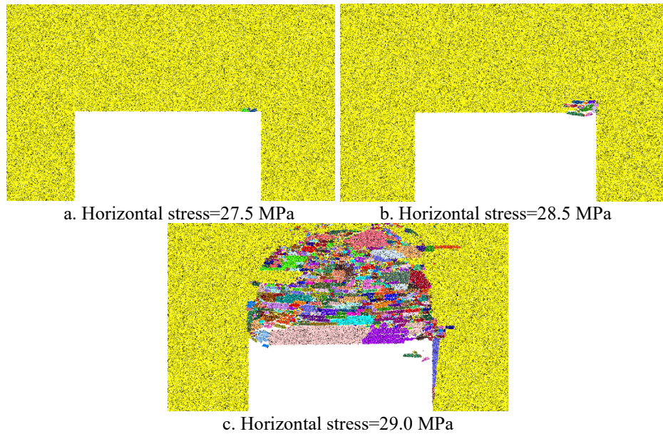
Fig. 4- 6 Failure mode of a laminated model with critical failure stress of 29.0MPa (bedding plane spacing=10cm; falling fragments kept here for illustration)
