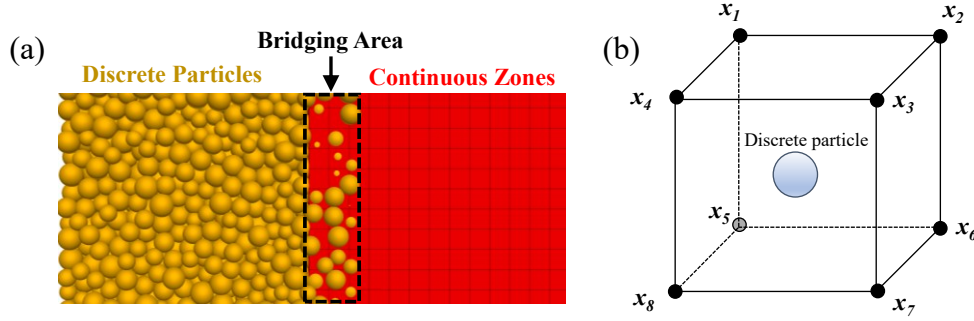
Fig. 6- 2 Depiction of coupling approach (a) and interpolation scheme (b) of ball-zone logic in PFC/FLAC
