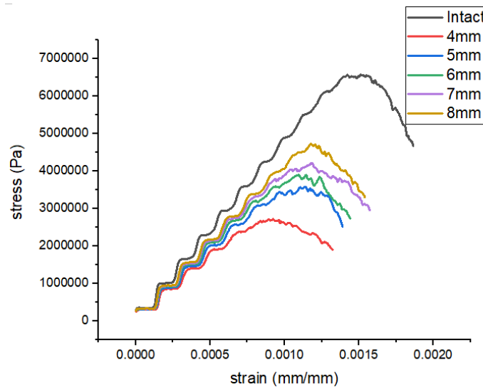
Fig. 5- 13 Stress-strain curves for specimens with different bedding plane spacings
