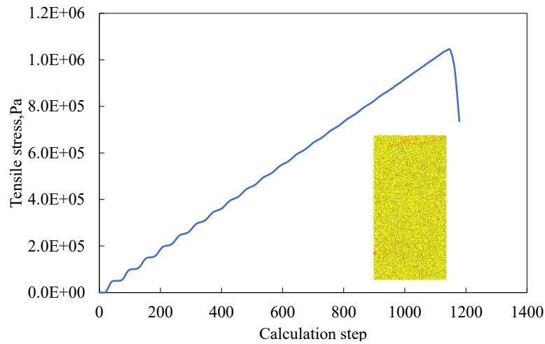
Fig. 5- 3 Calibration of direct tensile strength
