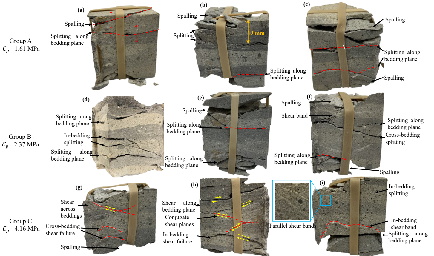
Fig. 3- 15 Failure mode of (a)-(c) group A, (d)-(f) group B, (g)-(i) group C subjected to biaxial stress
