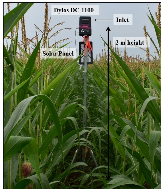
Figure 2. Dylos monitor in the field. The solar panel was used as backup power to the device in case of battery failure.
