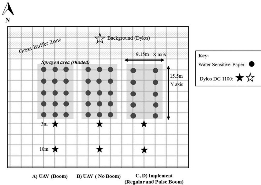
Figure 1. Field sampling layout by application type. The sprayed areas are shaded. One trial field was used for both implement spray trials to accommodate a wider path for the implement sprayer. Each box on the grid represents ~3 m. The prevailing wind was from the north.
