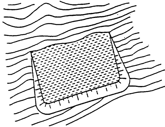
Sidehill Impoundment
