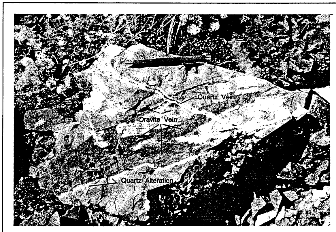
Figure 2. --Irregular dravite-tourmaline veining cross-cut by later quartz veins in quartz-tourmaline-altered hornfels
