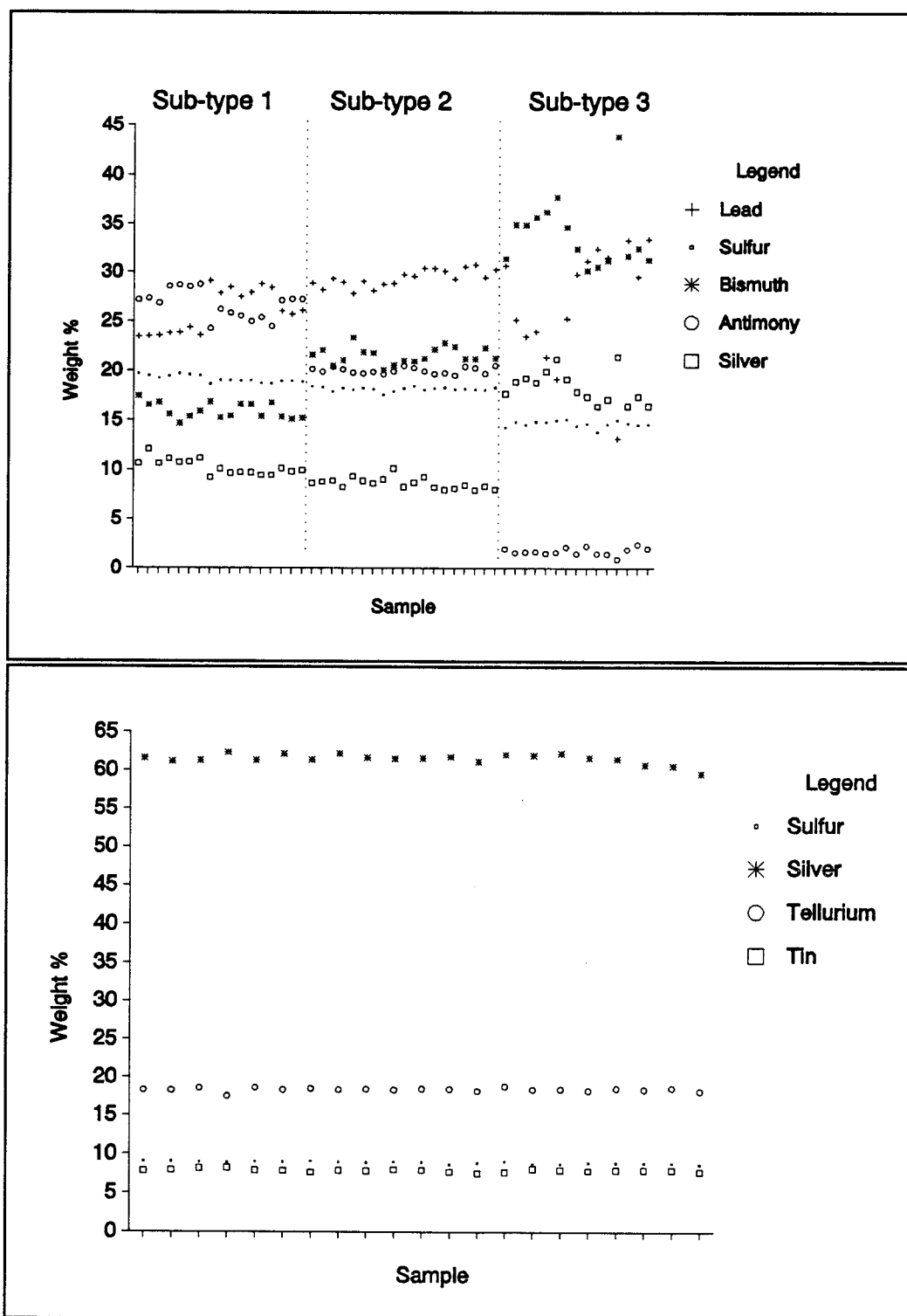
Figure 7. --Graphical representation of electron microprobe analysis of Pb-Bi-Sb-Ag-S and Ag-Te-Sn-S minerals in sample 6, appendix.
