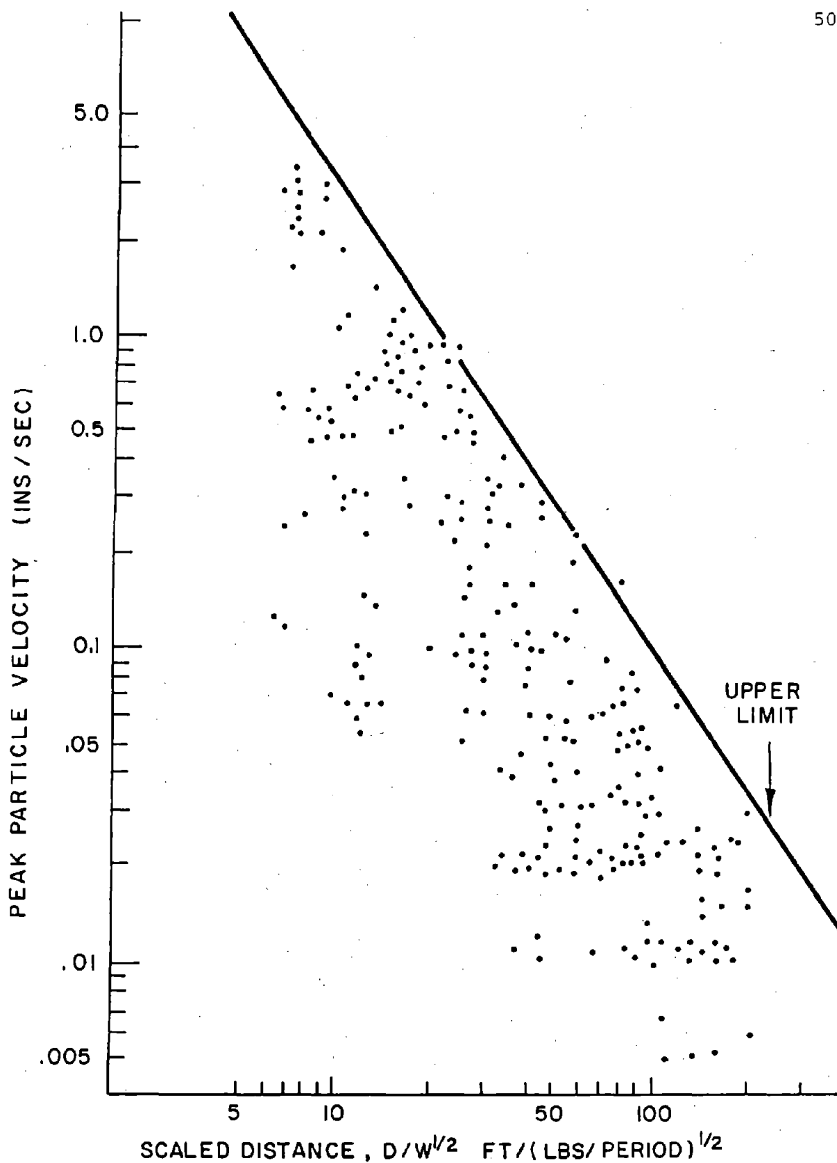
FIGURE 2-14: TYPICAL VIBRATION DATA FROM MULTIPERIOD DELAY BLASTS IN OPEN PITS AND ROCK STRIP MINES.
