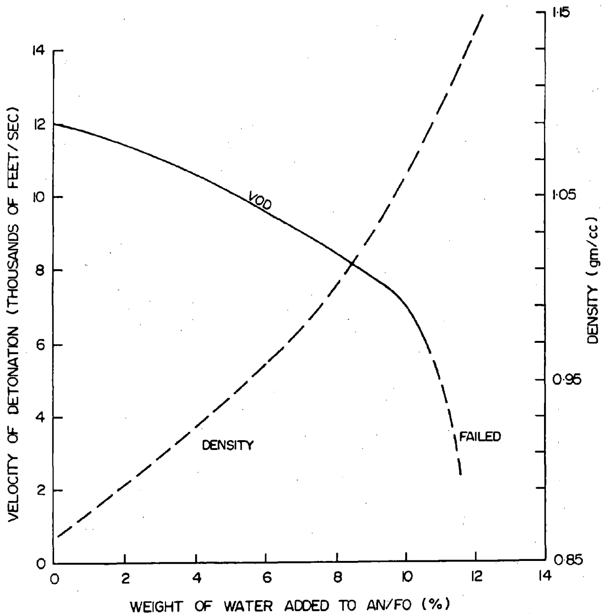
FIGURE 2-9: THE EFFECT OF WATER ADDITION TO AN/FO FIRED WITHIN 5 HOURS OF MIXING IN 4" DIAMETER PLASTIC PIPES USING 1# PROCORE PRIMERS.
