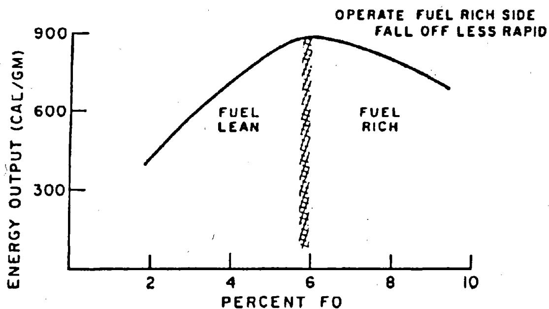
FIGURE 2-7: ENERGY OUTPUT VS. PERCENT FUEL OIL ADDED TO AMMONIUM NITRATE.
