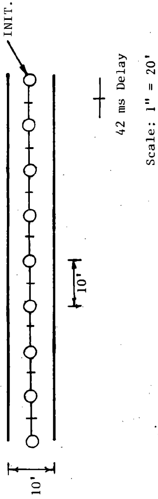
(a) Plan View of Blastholes Located Over a Mined Room Showing Hole Spacings and Firing Sequence
