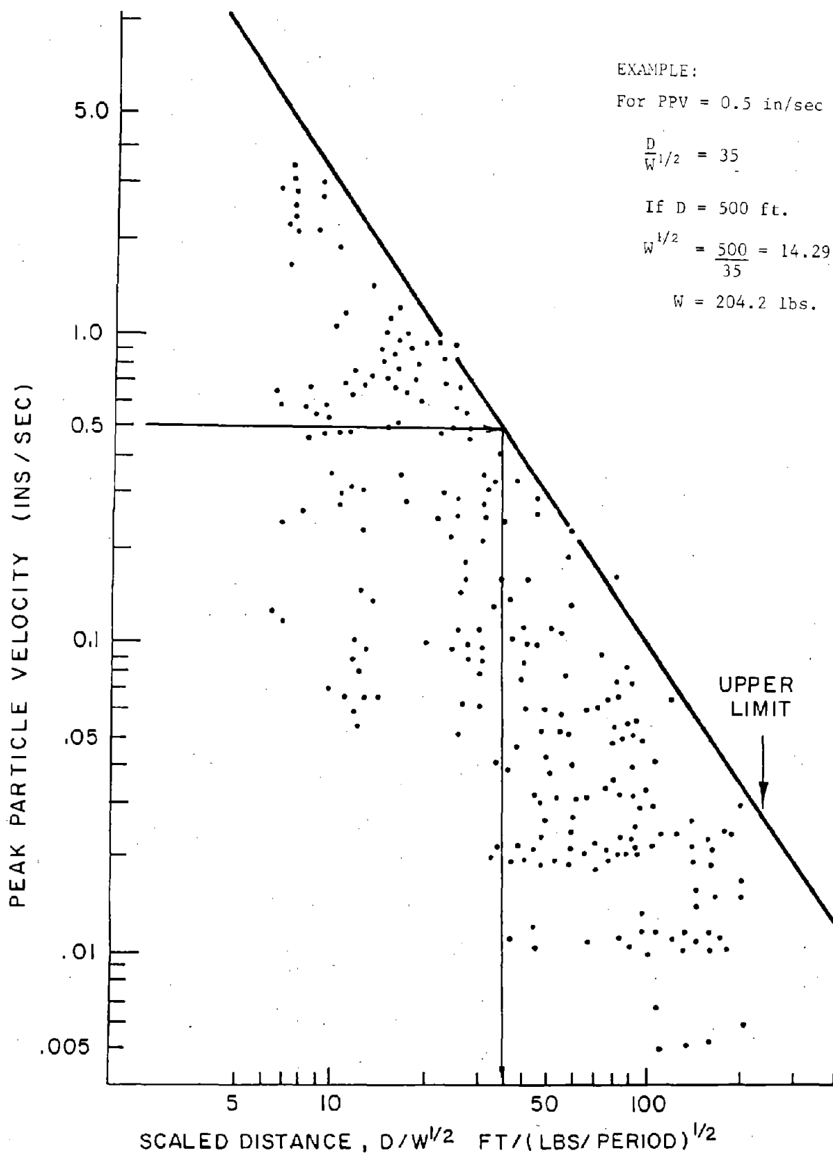
FIGURE 7-3: TYPICAL VIBRATION DATA FROM MULTIPERIOD DELAY BLASTS IN OPEN PITS AND ROCK STRIP MINES.
