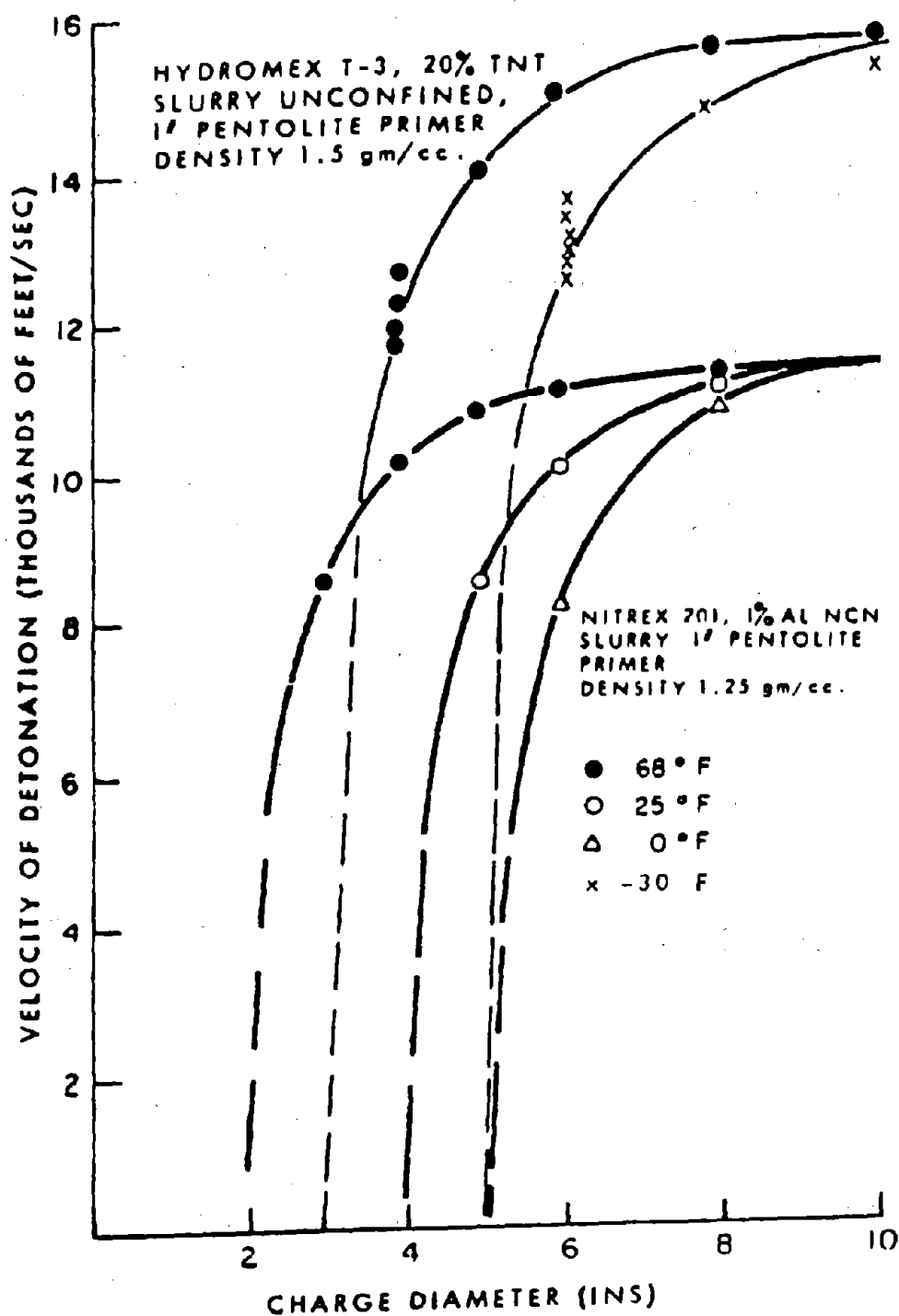
FIGURE 2-10: VELOCITY OF DETONATION CHARGE DIAMETER CURVES FOR A 1% AL NCN SLURRY, AND A 20% TNT SLURRY FIRED AT DIFFERENT TEMPERATURES.
