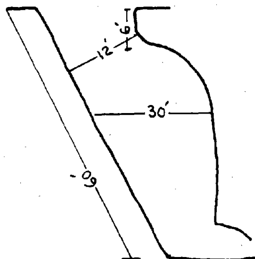
FIGURE 4-8: POST-BLASTING RESULT AND PREBLASTING DIAGRAMS OF VO-4B
