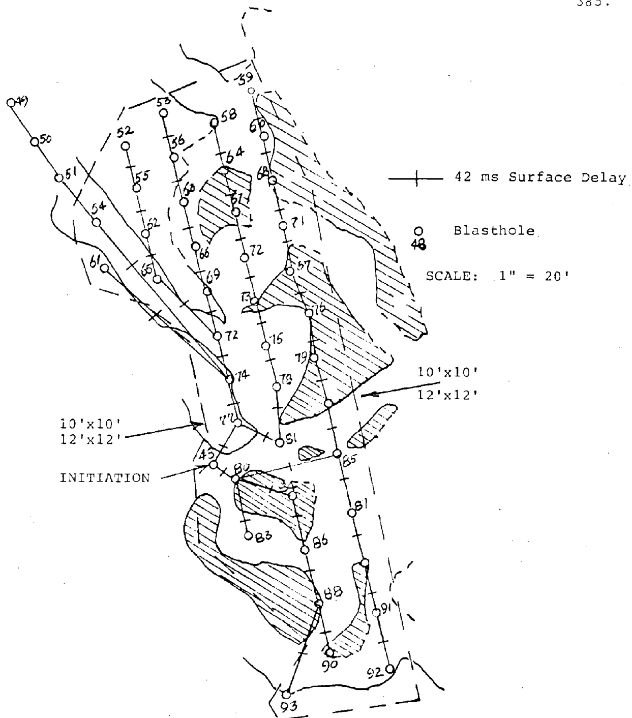
FIGURE B-6: BLASTHOLE LAYOUT AND TIE-IN DIAGRAM FOR BLAST B-6
