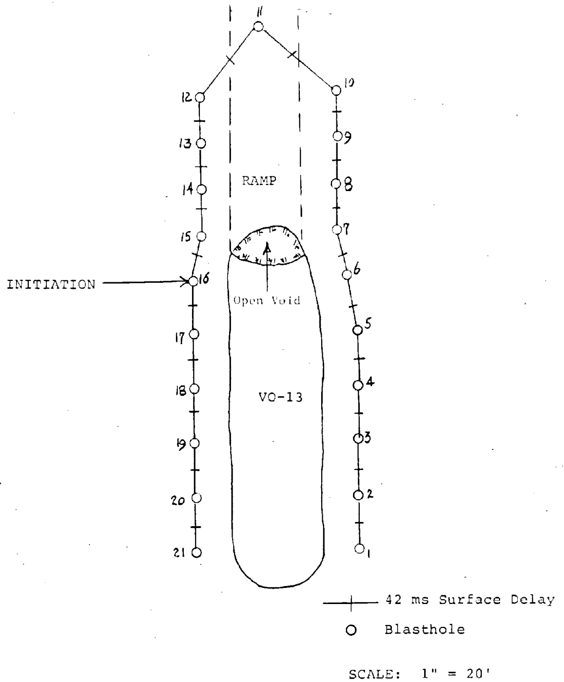
FIGURE A-18: BLAST LAYOUT AND TIE-IN FOR BLAST VC-13
