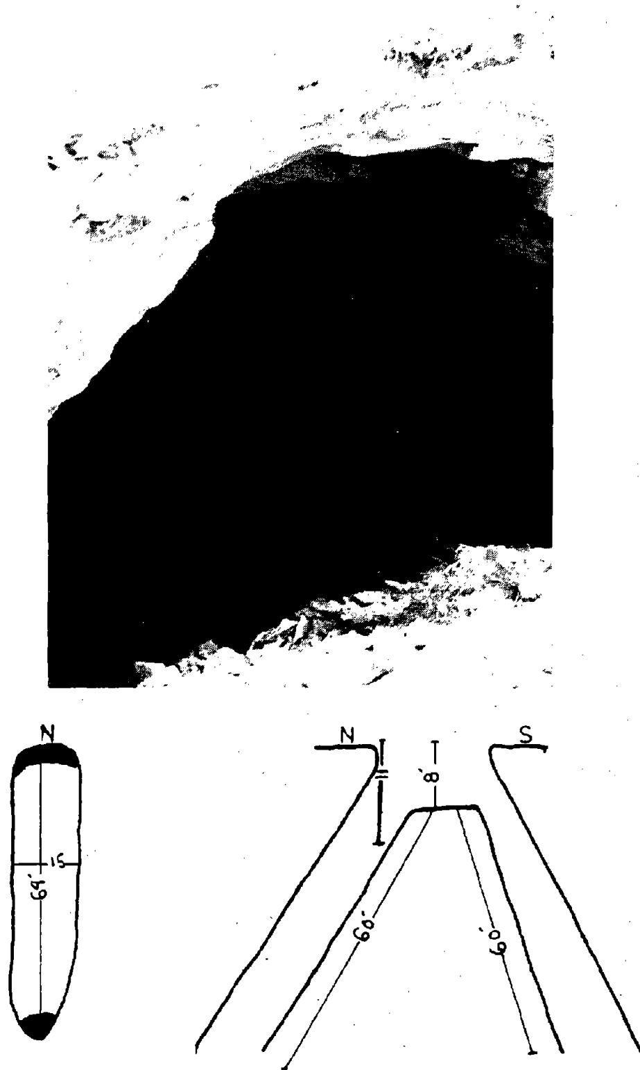
FIGURE 4-11: PREBLAST PHOTOGRAPH AND DIAGRAMS OF VO-7
