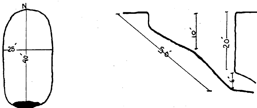
FIGURE 4-7: POST-BLASTING RESULT AND DIAGRAMS OF PREBLASTING DIMENSIONS OF VO-4A
