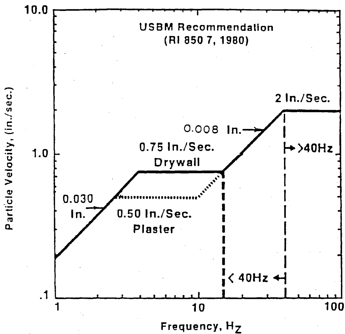
FIGURE 2-13: USBM RECOMMENDATION FOR SAFE BLASTING
