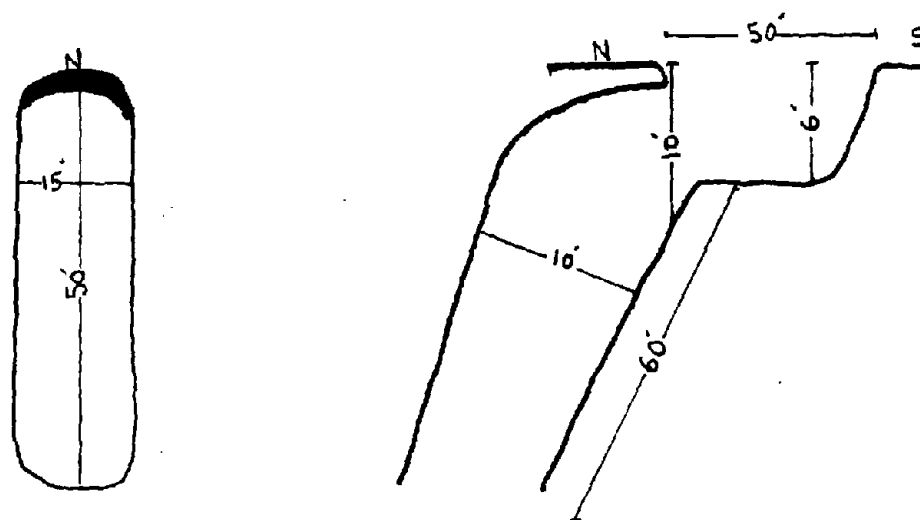
FIGURE 4-12: PREBLASTING PHOTOGRAPH OF AND DIAGRAM OF VO-8
